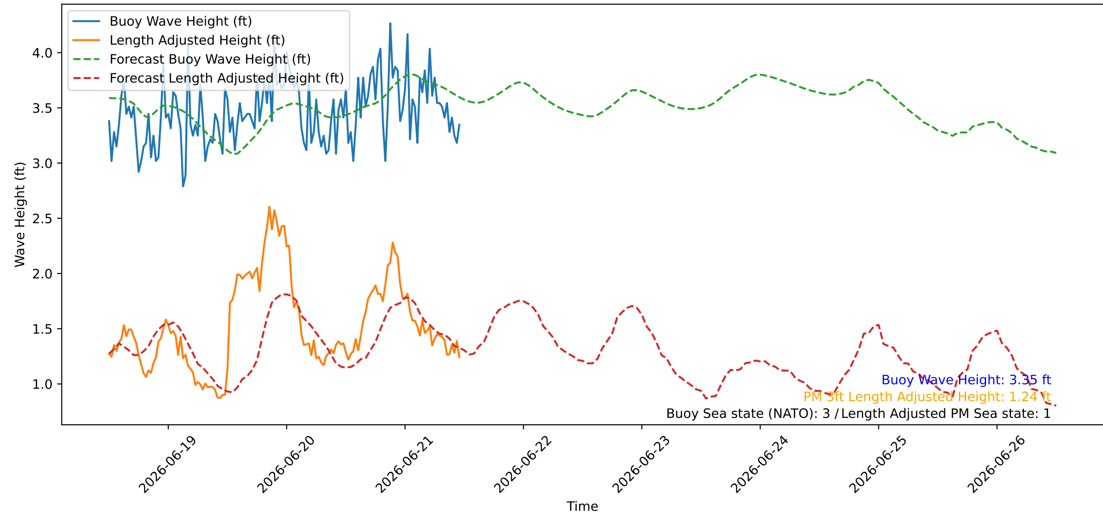
Wave Heights over Time for Oceanside Harbor at 2026-06-21 11:50:26
