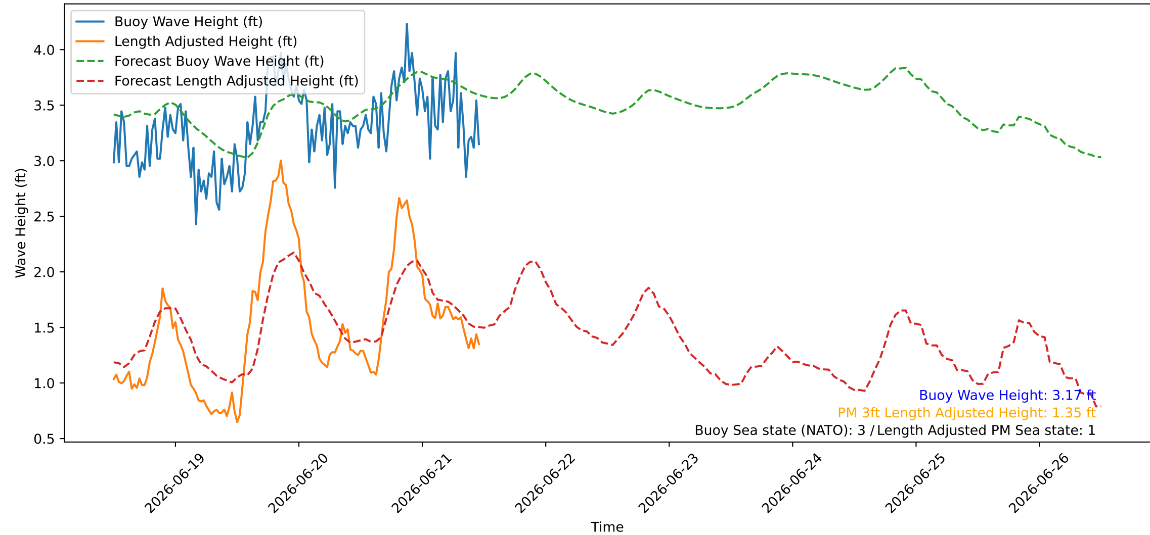
Wave Heights over Time for Green Beach at 2026-06-21 11:51:09
