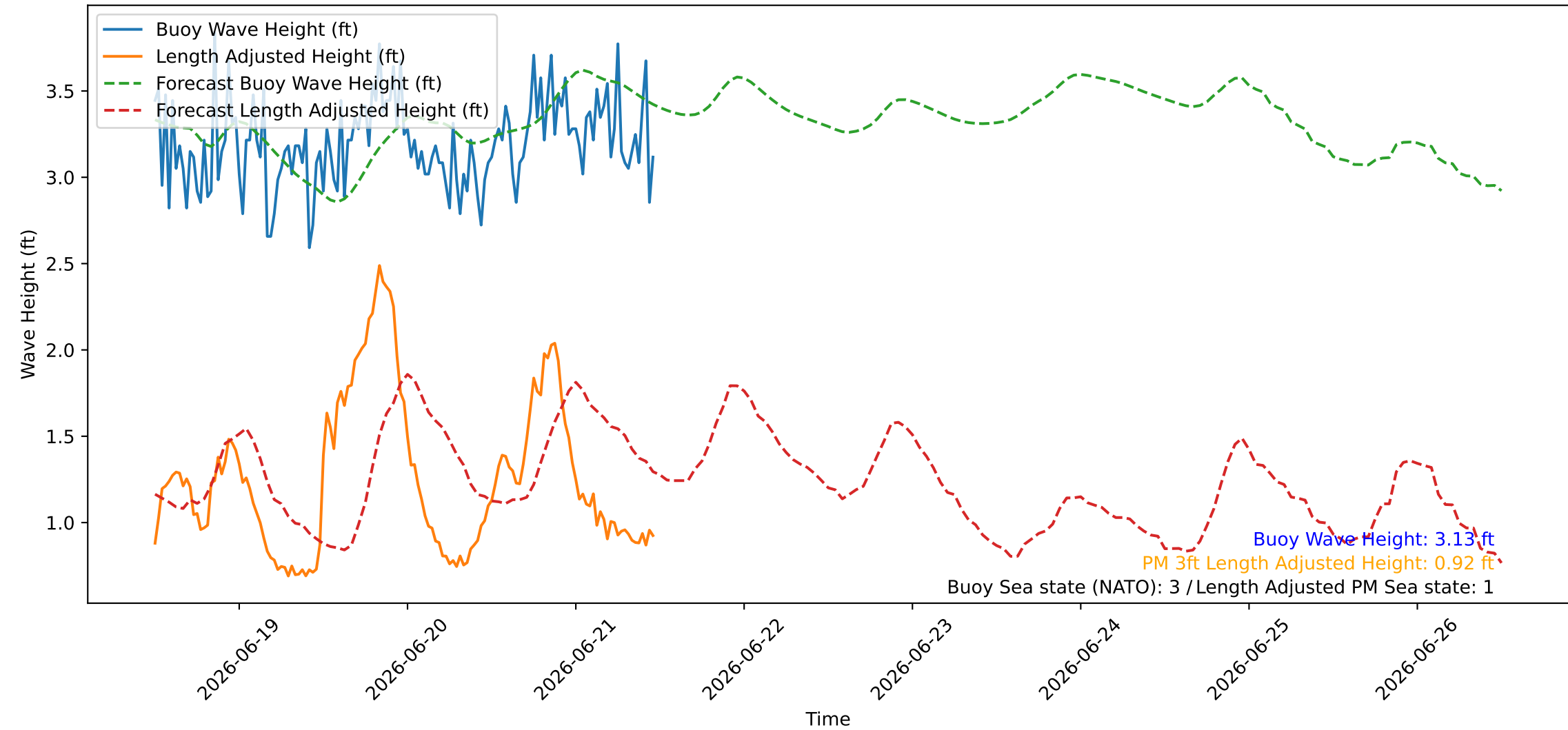
Wave Heights over Time for Red Beach at 2026-06-21 11:50:46
