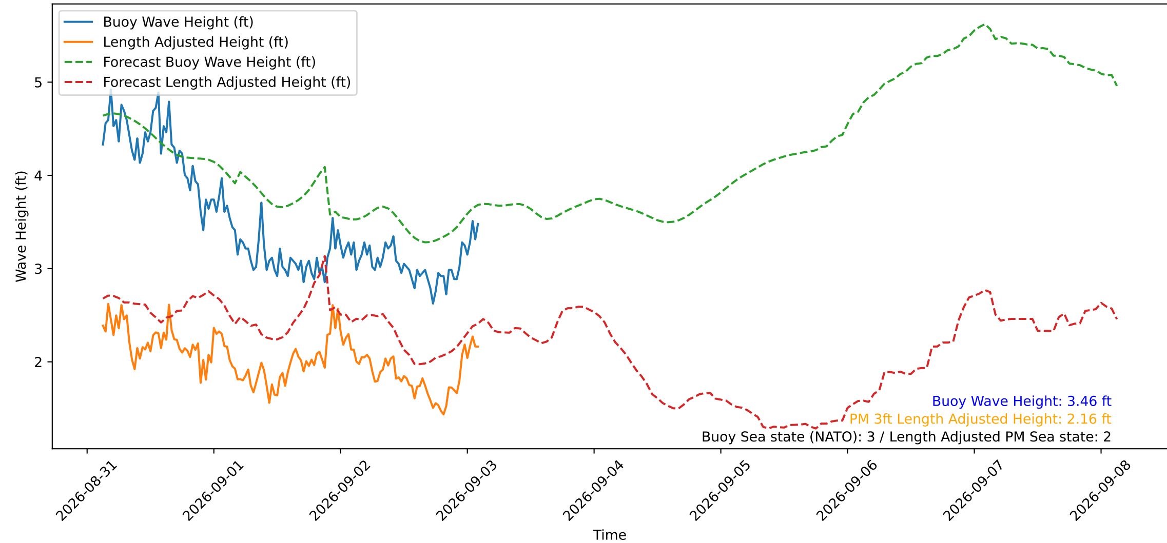
Wave Heights over Time for Oceanside Harbor at 2026-09-03 02:50:31
