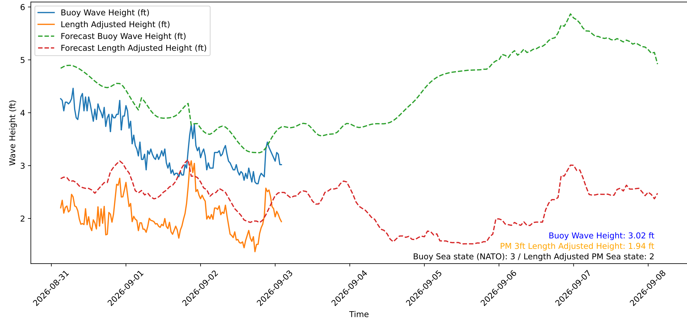
Wave Heights over Time for Green Beach at 2026-09-03 02:51:18
