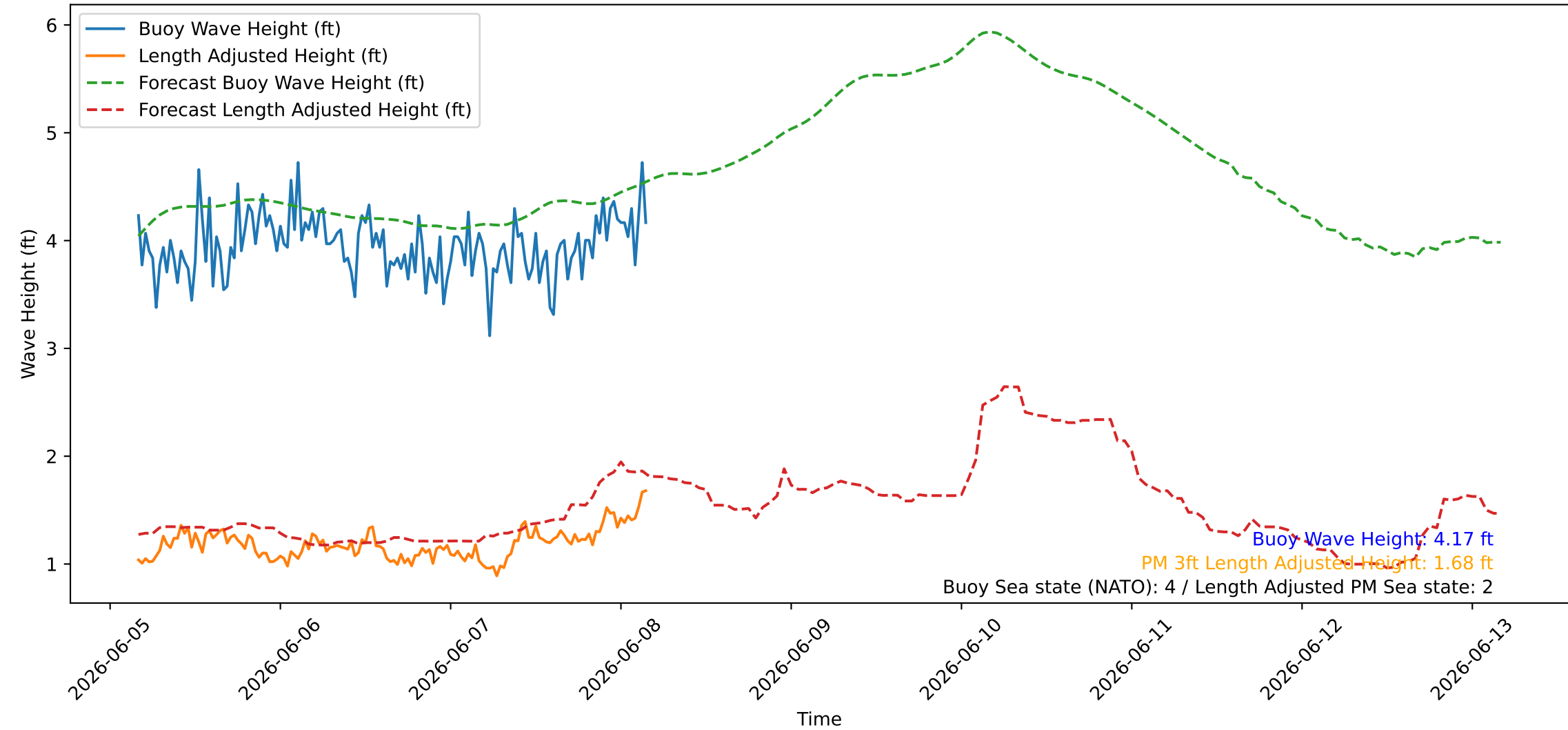
Wave Heights over Time for Green Beach at 2026-06-08 04:11:08
