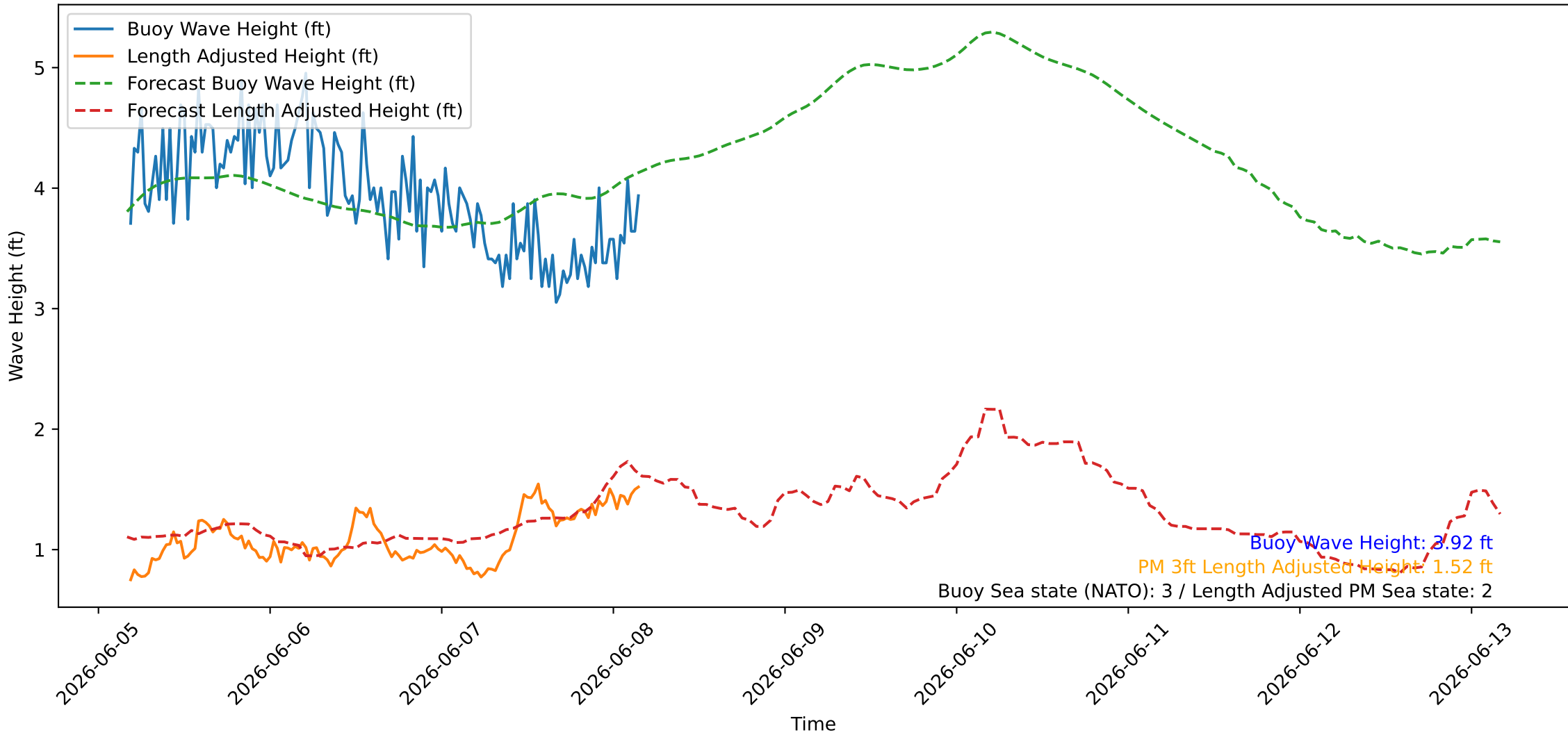
Wave Heights over Time for Red Beach at 2026-06-08 04:10:45
