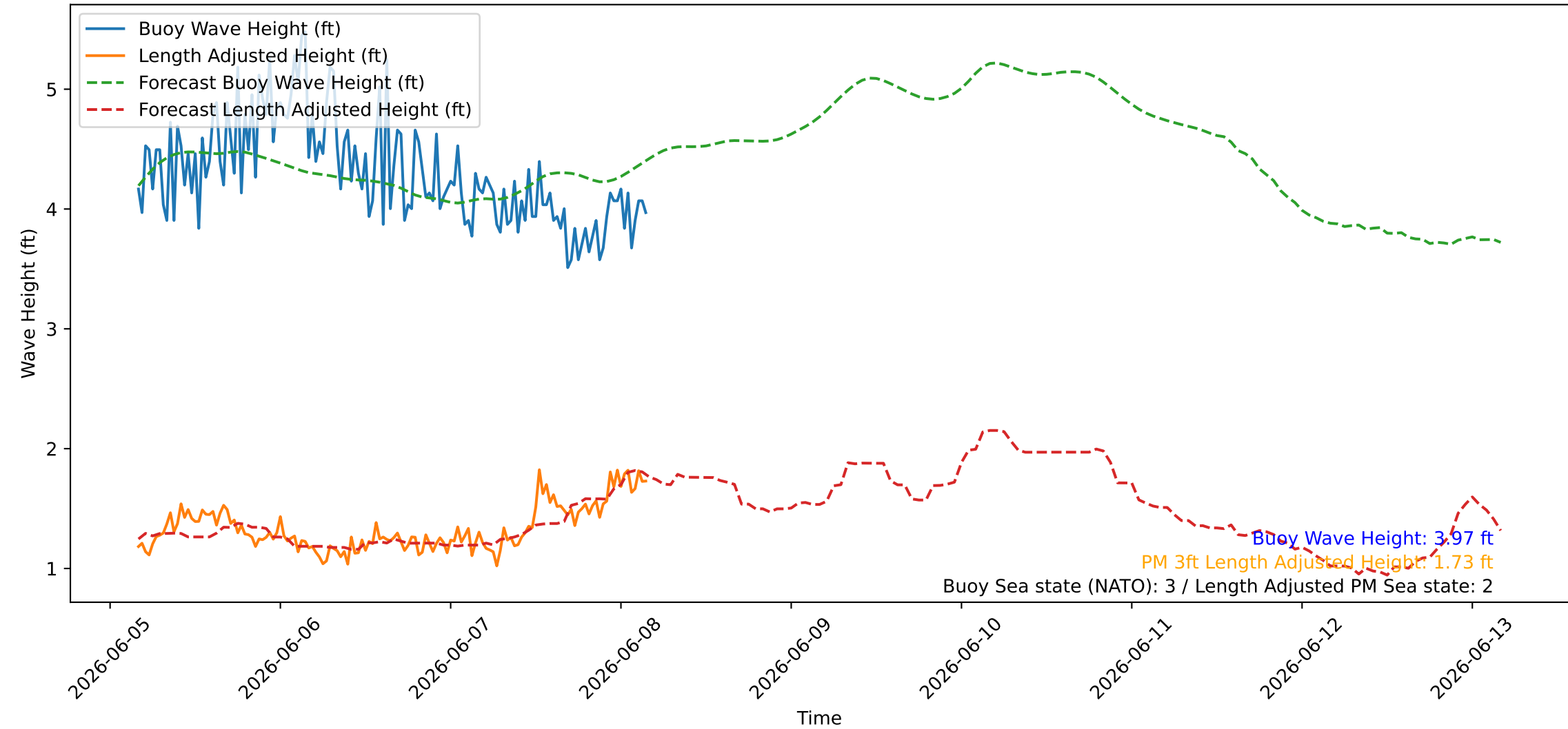
Wave Heights over Time for Oceanside Harbor at 2026-06-08 04:10:26
