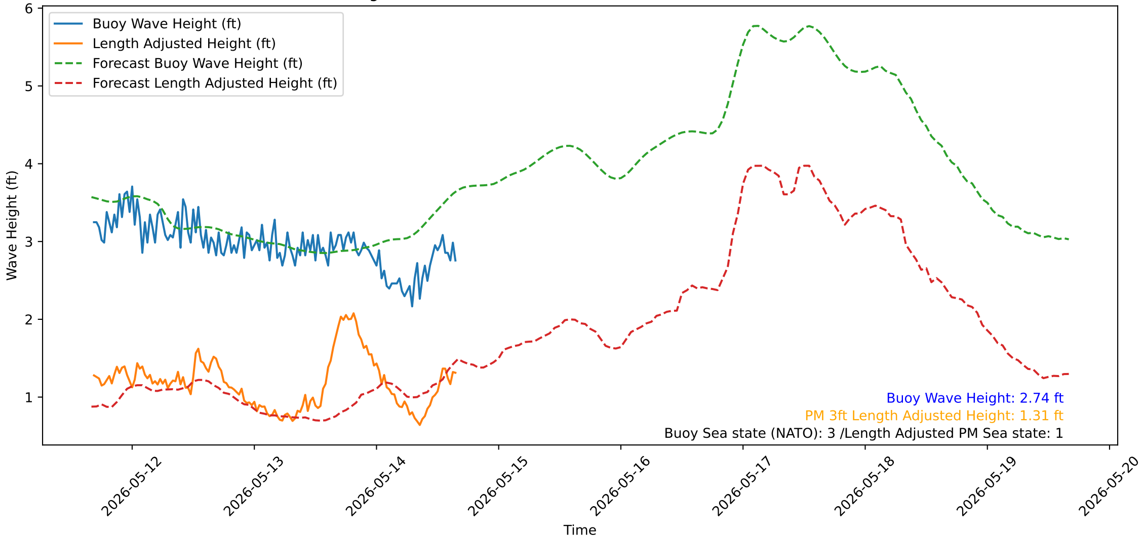
Wave Heights over Time for Oceanside Harbor at 2026-05-14 16:20:33
