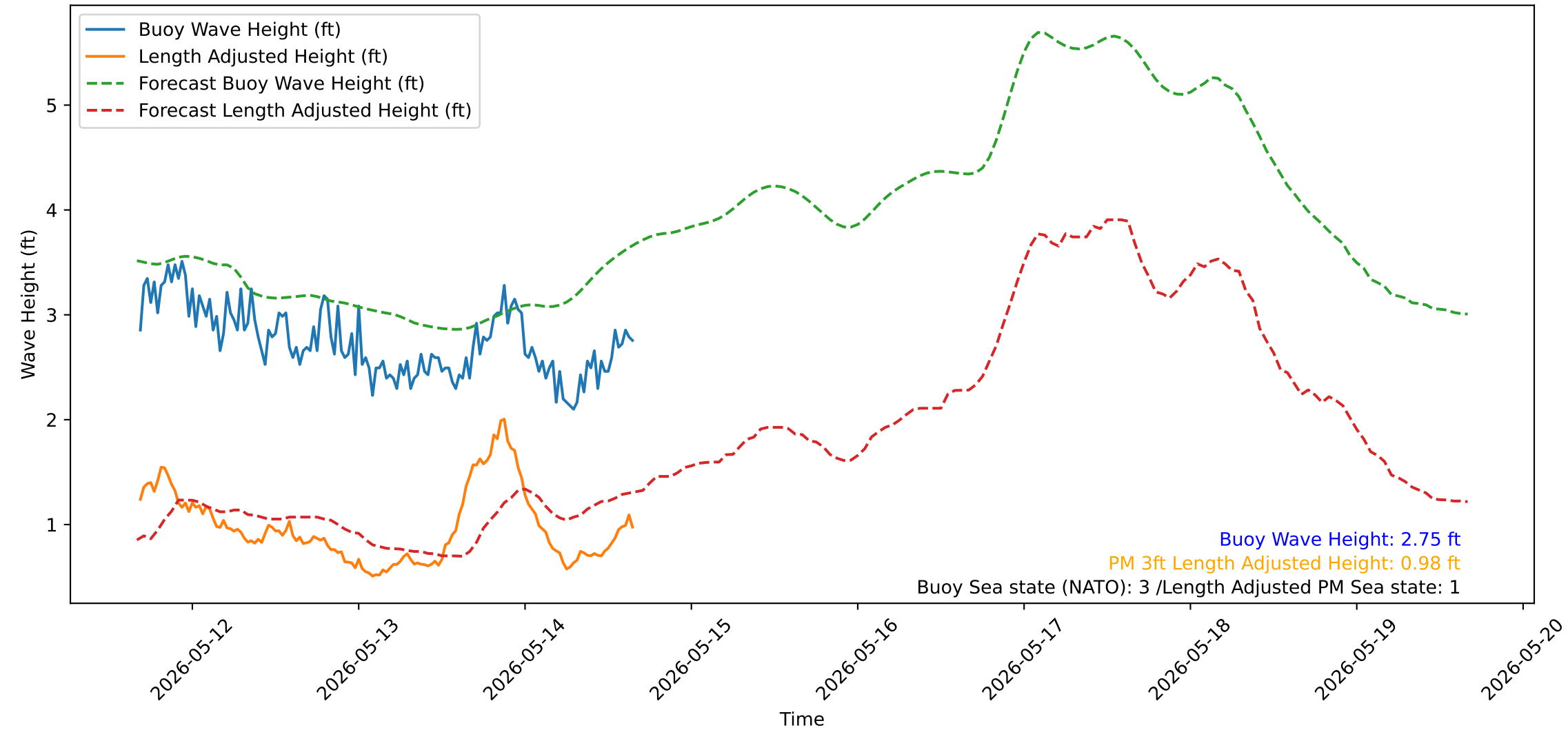
Wave Heights over Time for Green Beach at 2026-05-14 16:21:17
