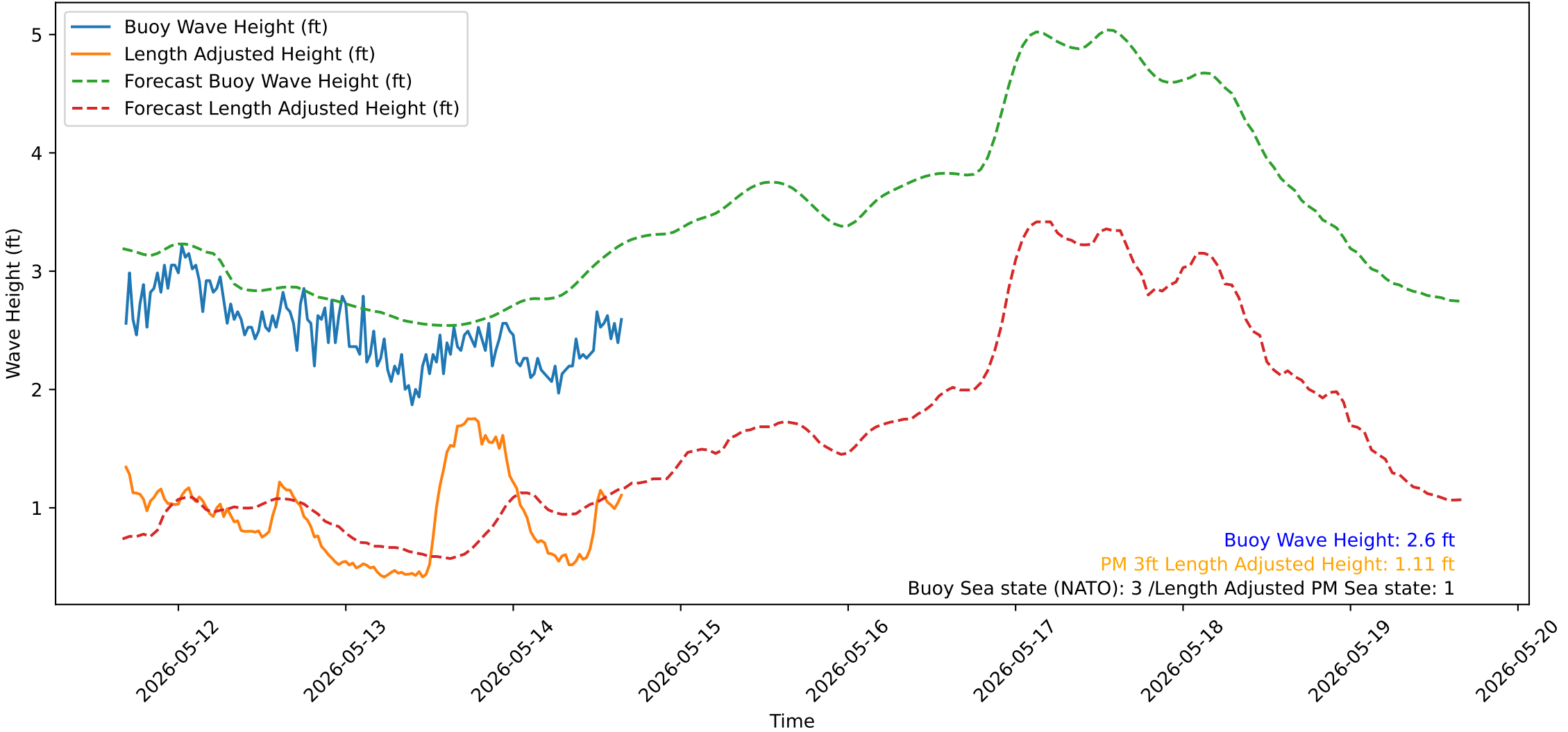
Wave Heights over Time for Red Beach at 2026-05-14 16:20:54
