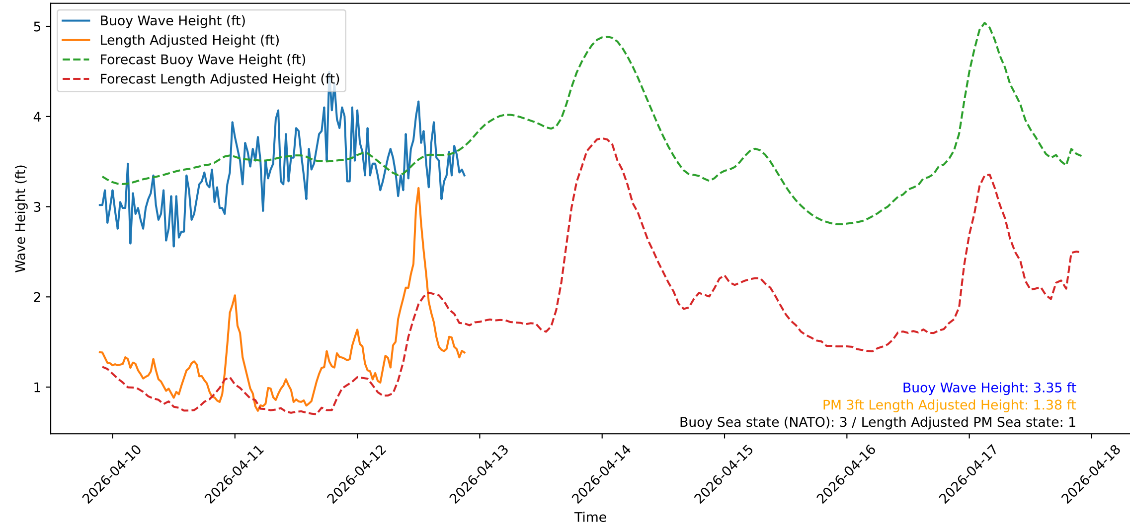
Wave Heights over Time for Green Beach at 2026-04-12 21:41:12
