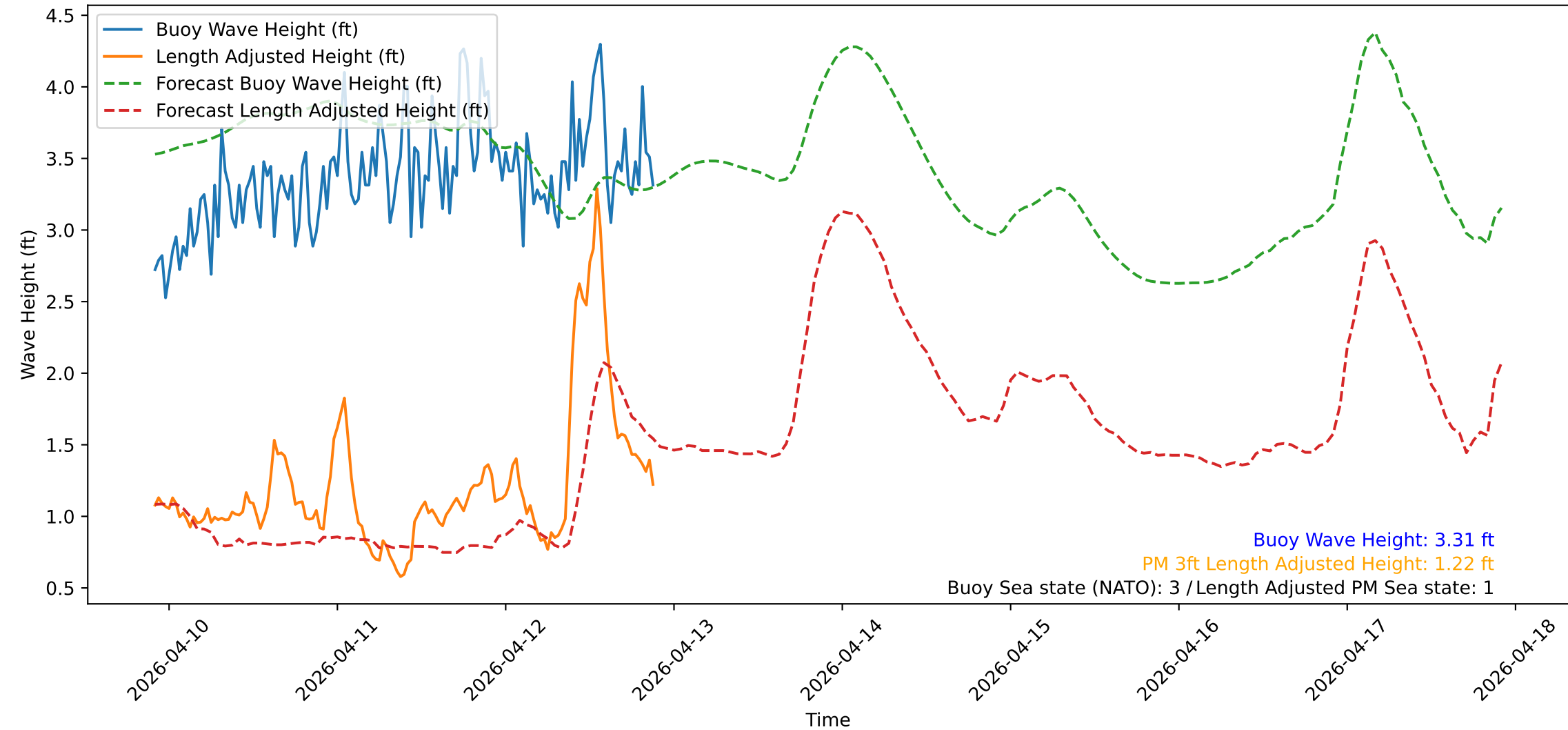
Wave Heights over Time for Red Beach at 2026-04-12 21:40:50
