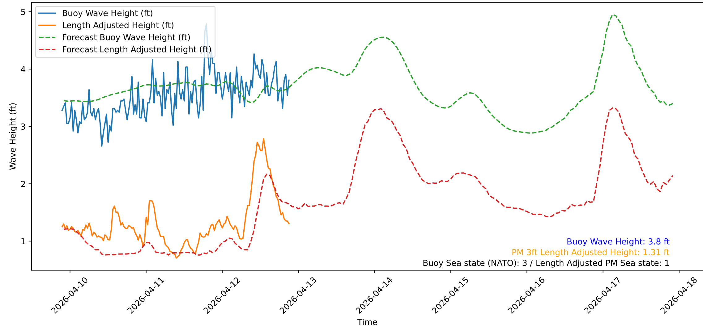
Wave Heights over Time for Oceanside Harbor at 2026-04-12 21:40:31
