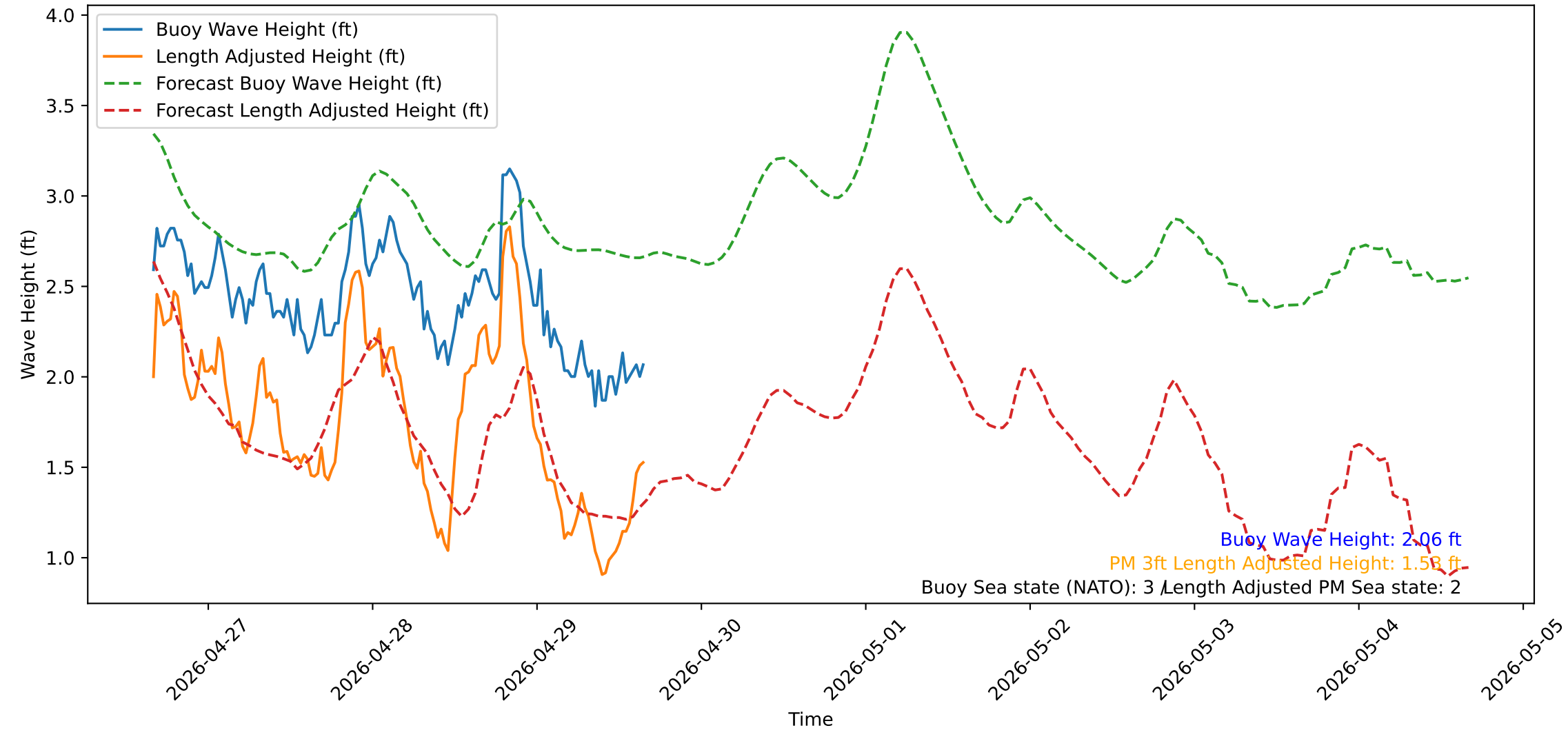
Wave Heights over Time for Green Beach at 2026-04-29 16:11:13
