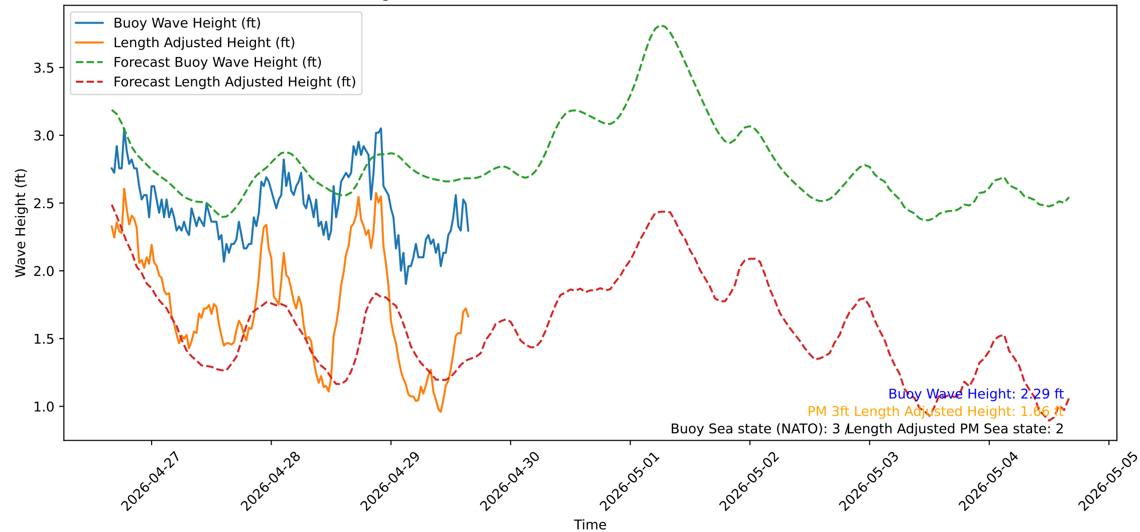
Wave Heights over Time for Oceanside Harbor at 2026-04-29 16:10:31
