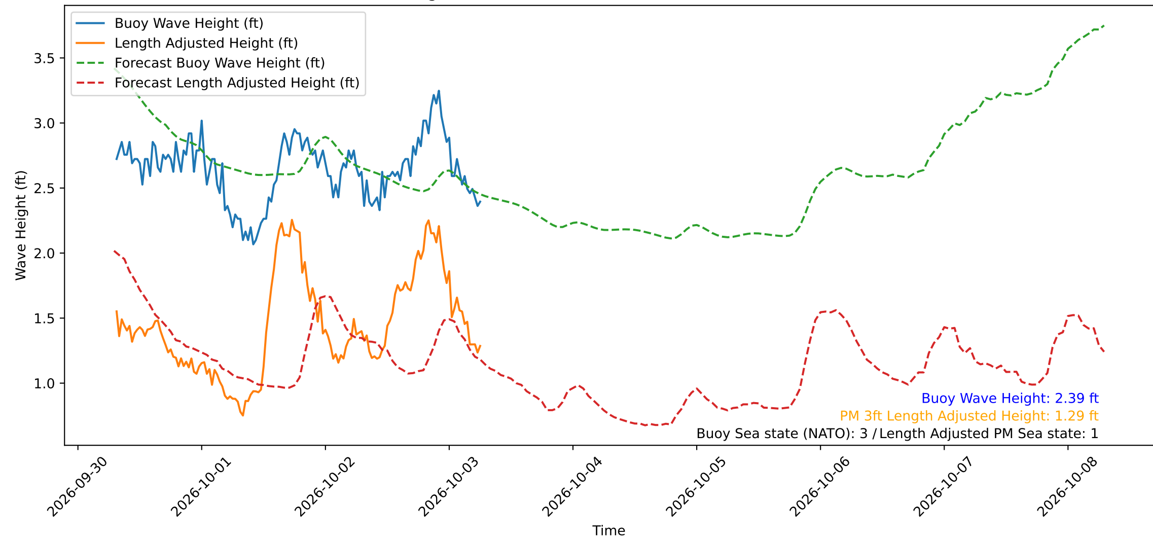
Wave Heights over Time for Red Beach at 2026-10-03 07:00:49
