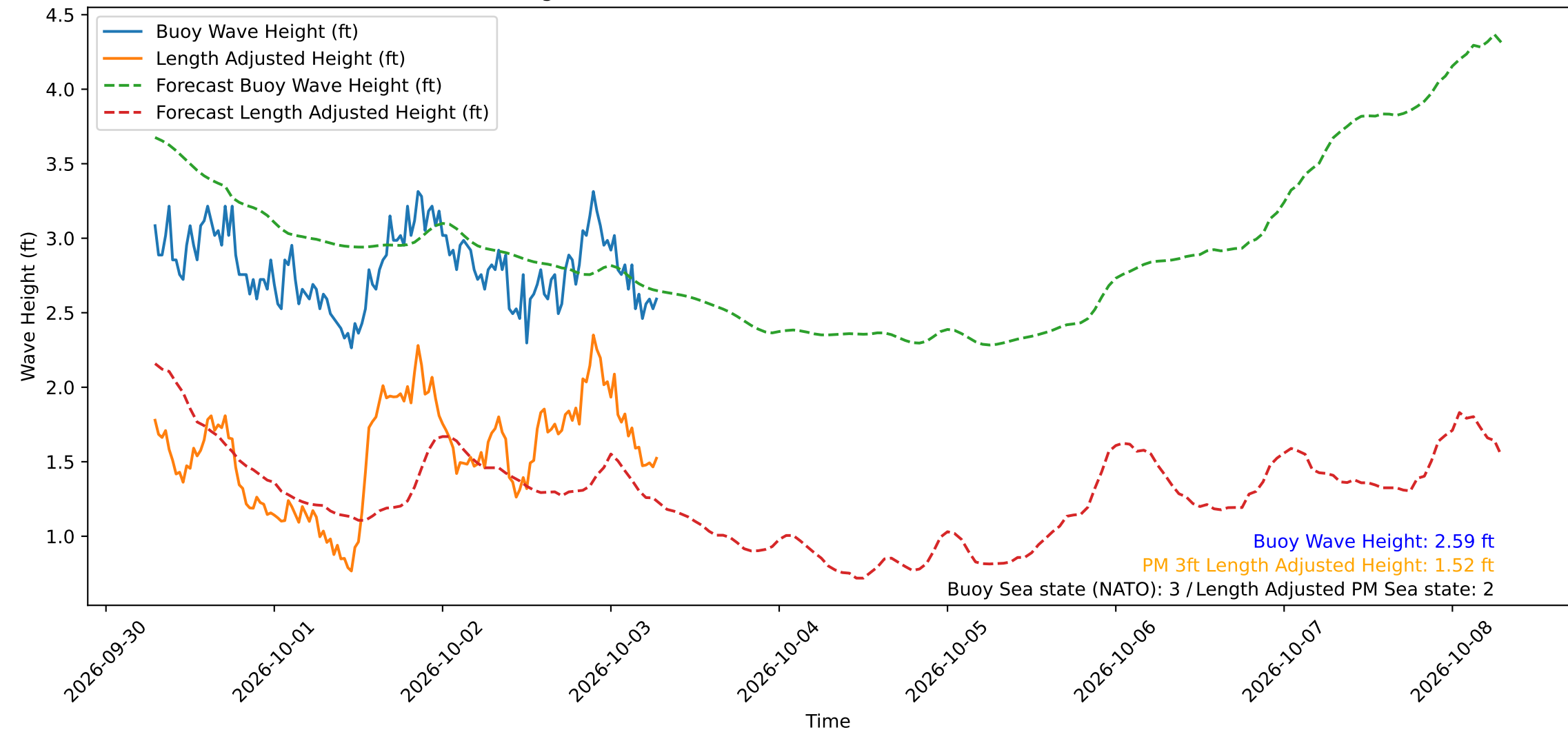
Wave Heights over Time for Oceanside Harbor at 2026-10-03 07:00:29
