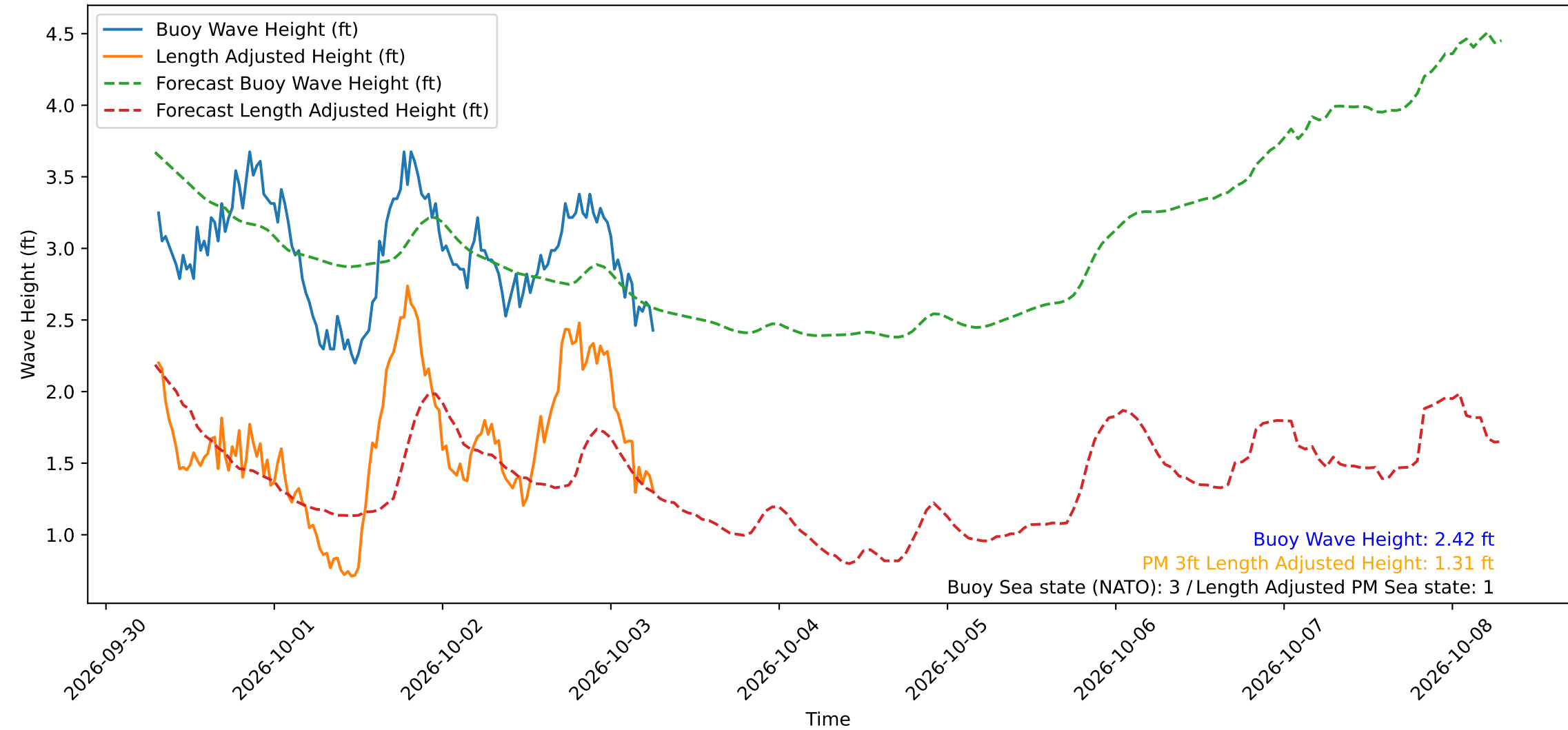
Wave Heights over Time for Green Beach at 2026-10-03 07:01:11
