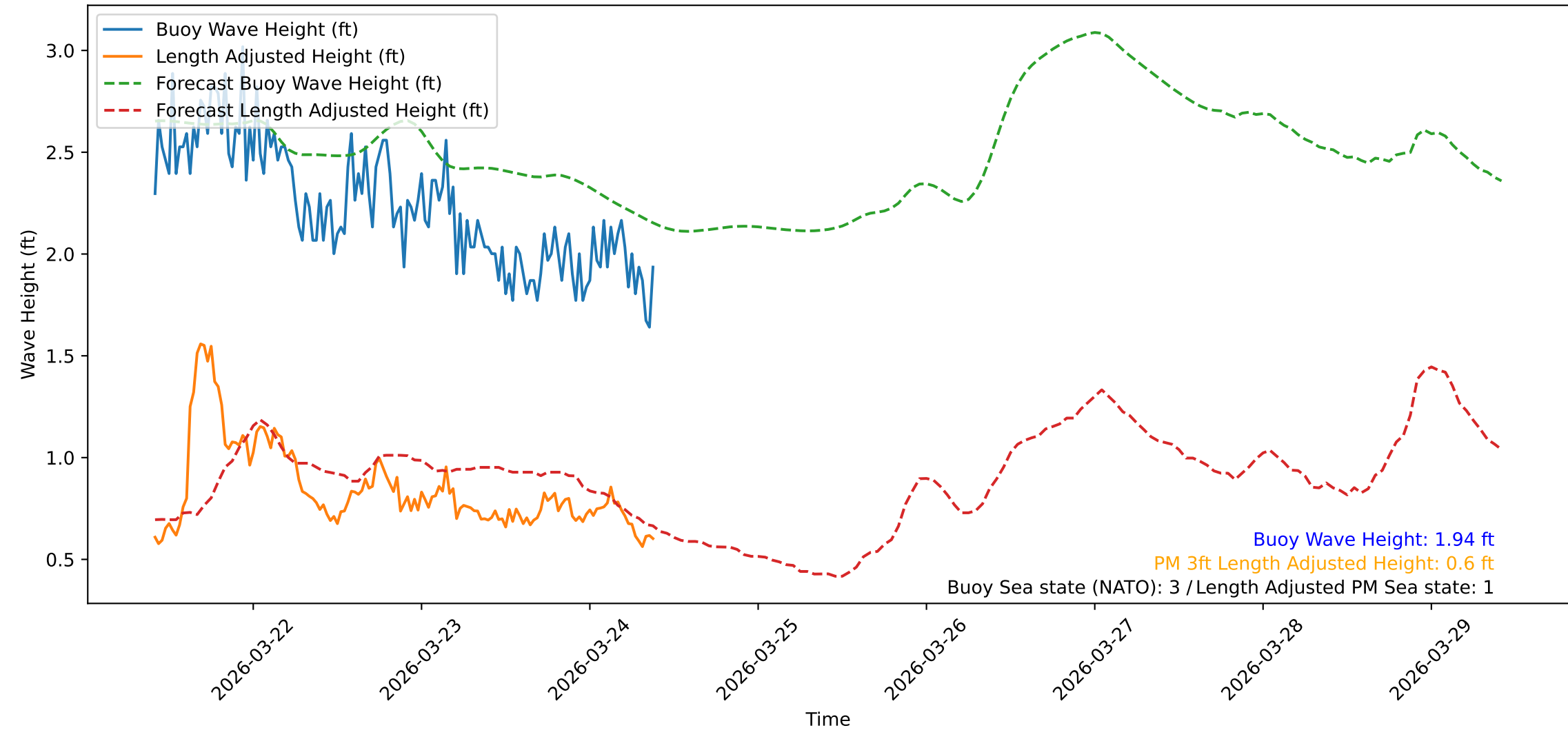
Wave Heights over Time for Oceanside Harbor at 2026-03-24 10:00:31
