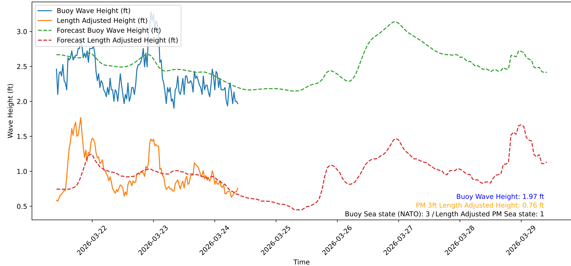
Wave Heights over Time for Green Beach at 2026-03-24 10:01:09
