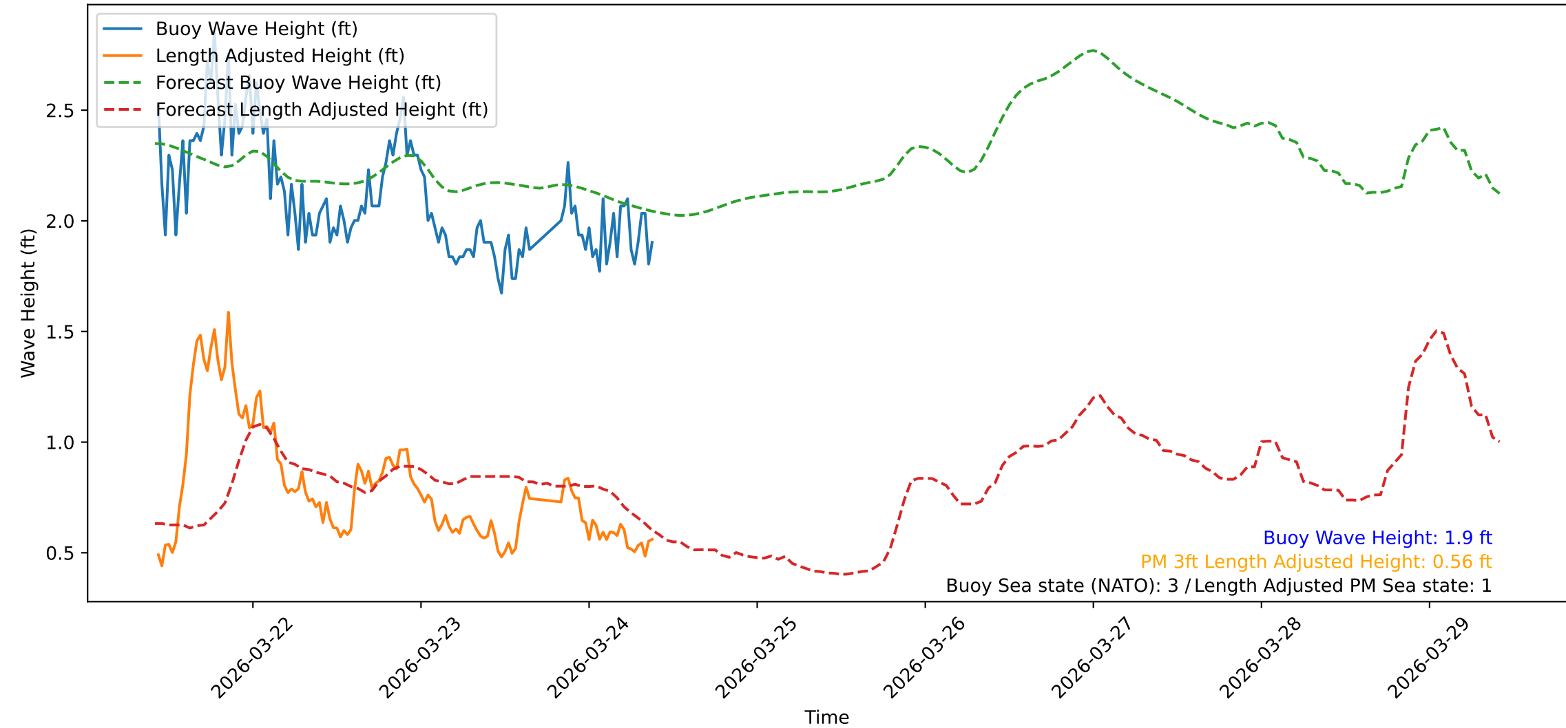
Wave Heights over Time for Red Beach at 2026-03-24 10:00:47
