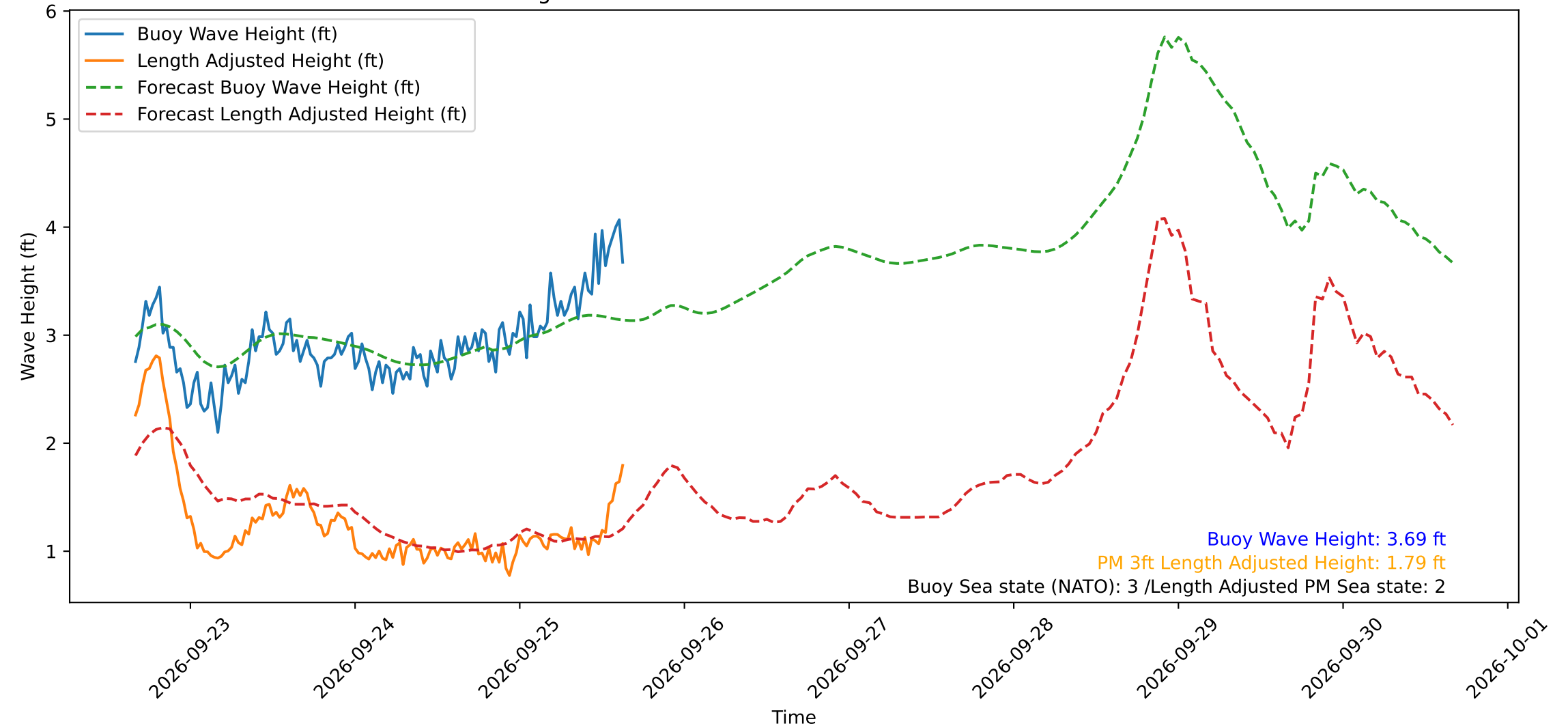
Wave Heights over Time for Green Beach at 2026-09-25 15:41:11
