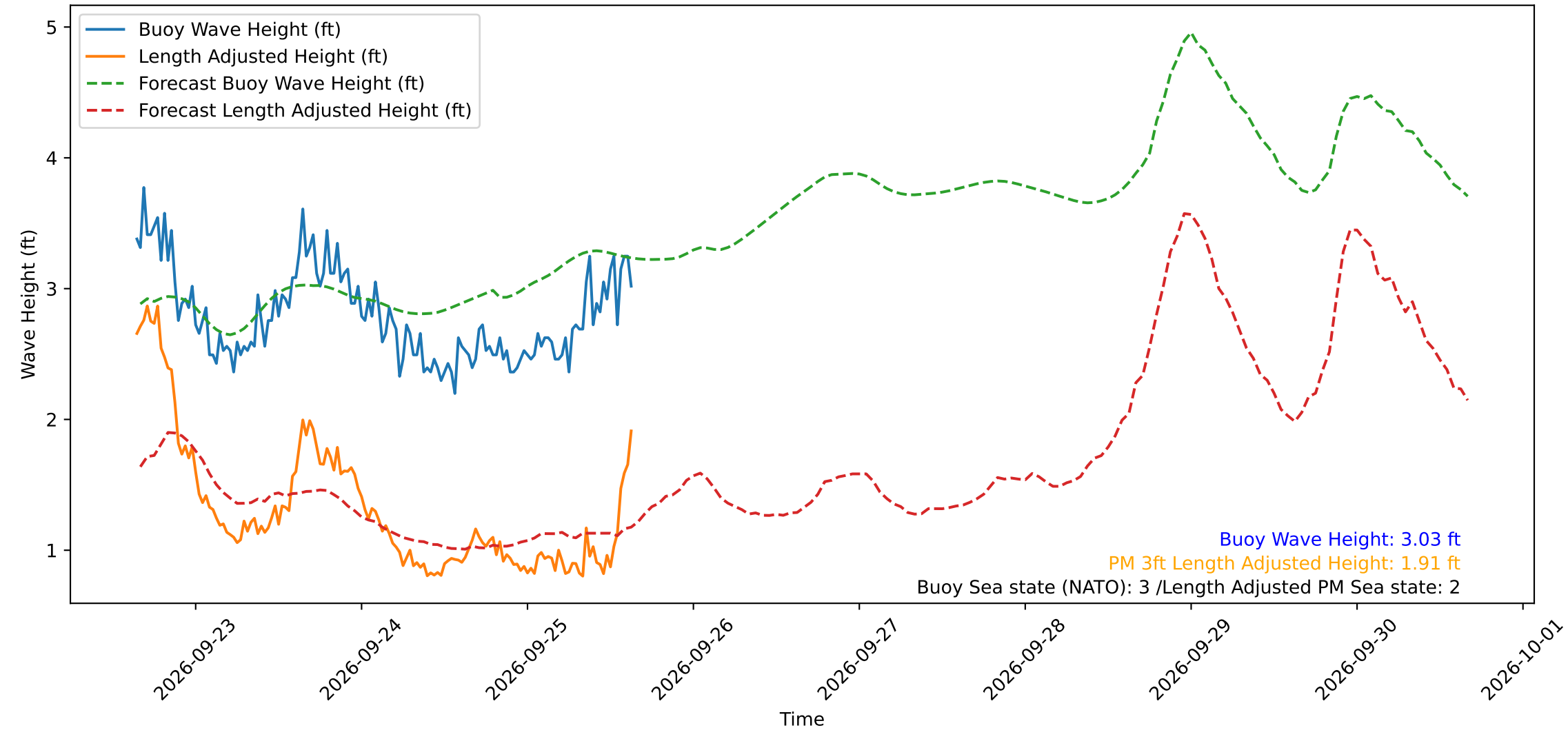
Wave Heights over Time for Oceanside Harbor at 2026-09-25 15:40:29
