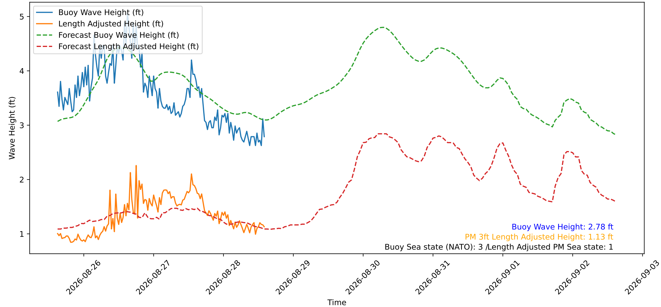
Wave Heights over Time for Red Beach at 2026-08-28 14:40:50
