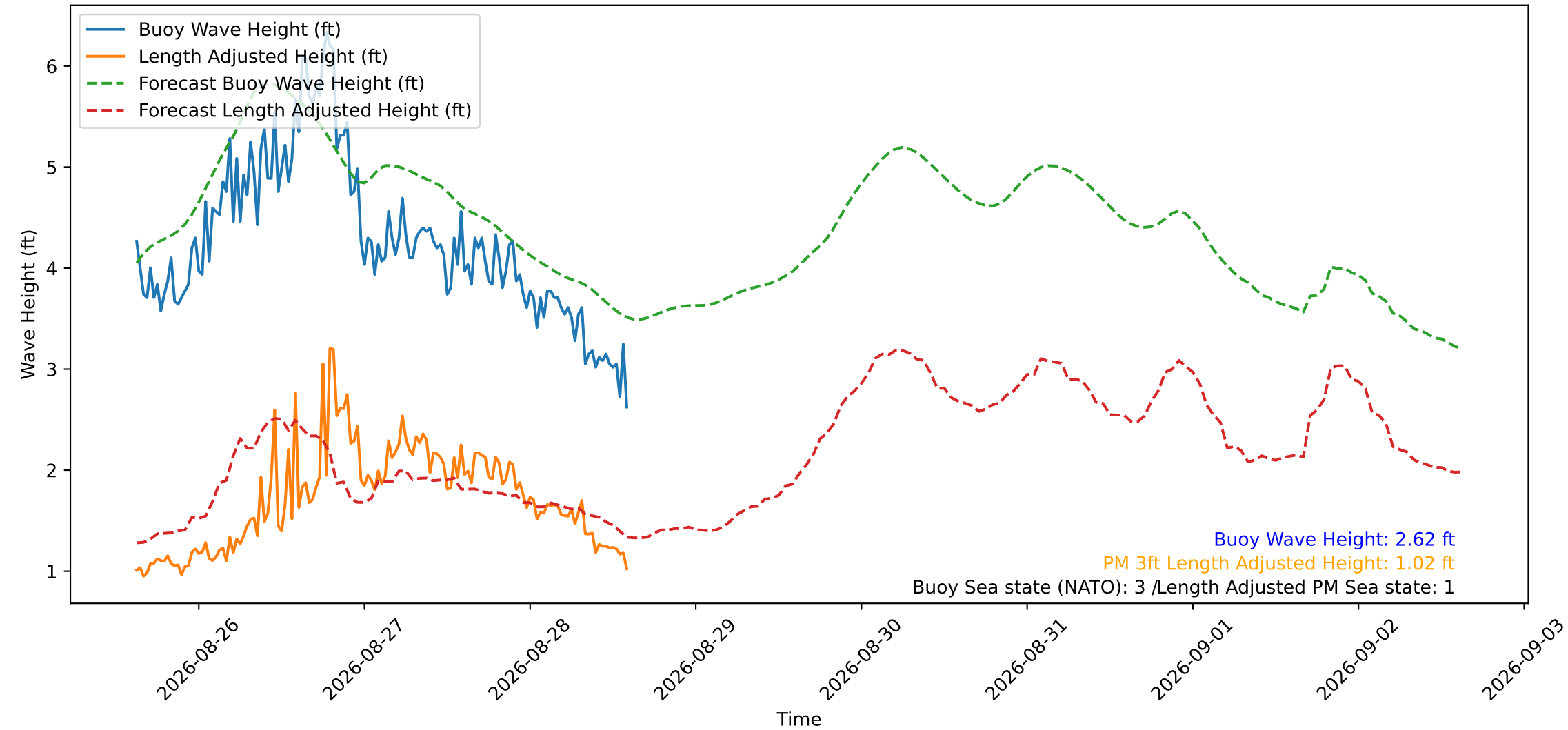
Wave Heights over Time for Green Beach at 2026-08-28 14:41:15
