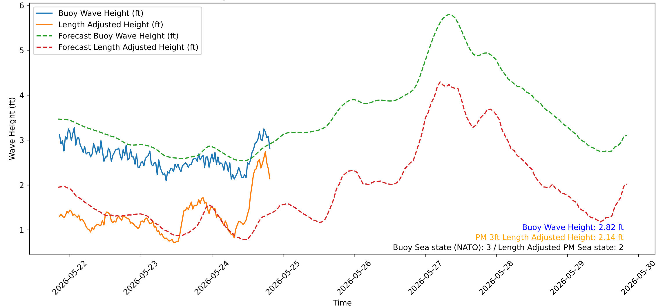
Wave Heights over Time for Oceanside Harbor at 2026-05-24 20:20:32
