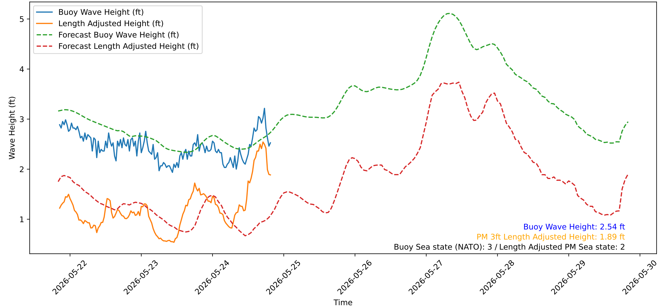
Wave Heights over Time for Red Beach at 2026-05-24 20:20:53
