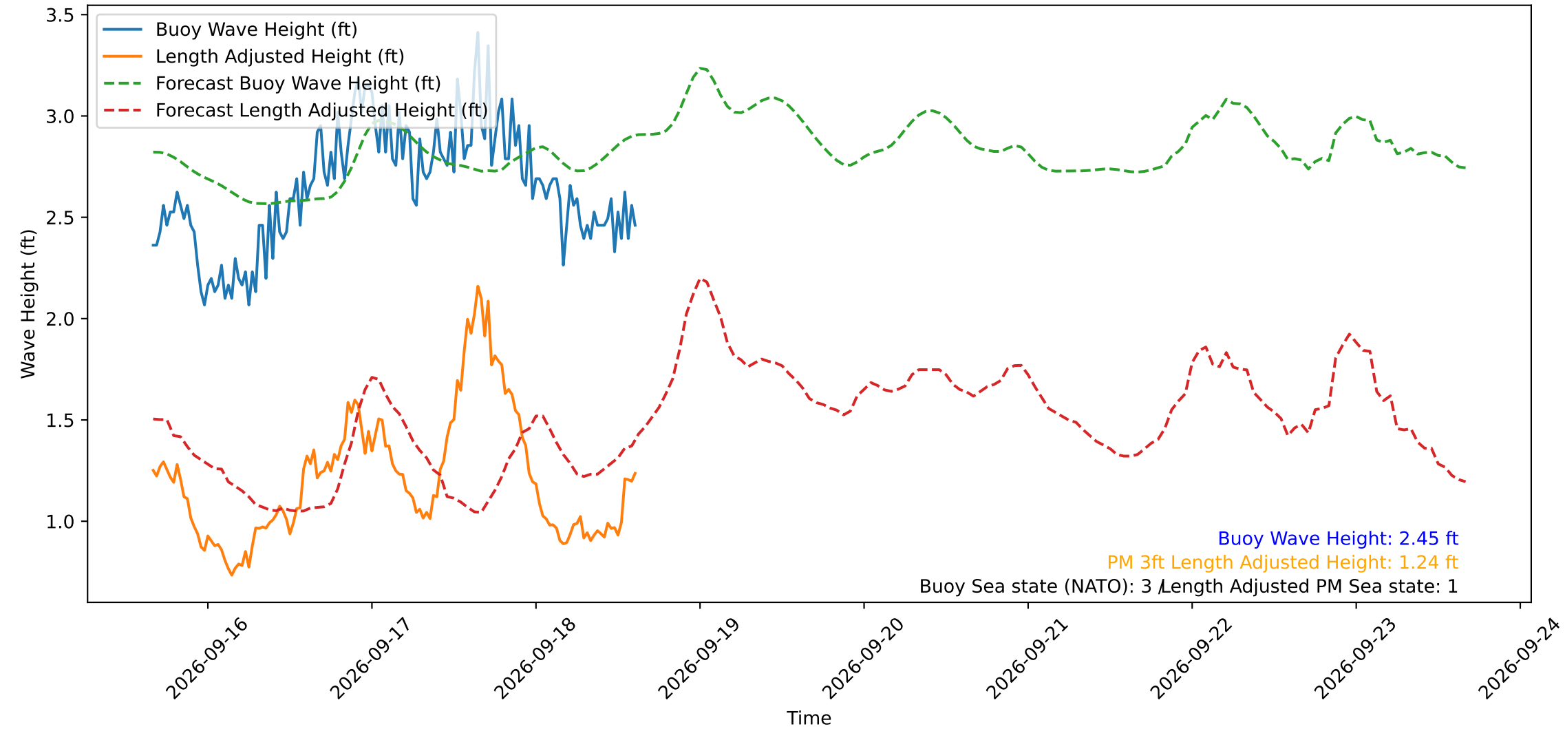
Wave Heights over Time for Red Beach at 2026-09-18 15:30:49
