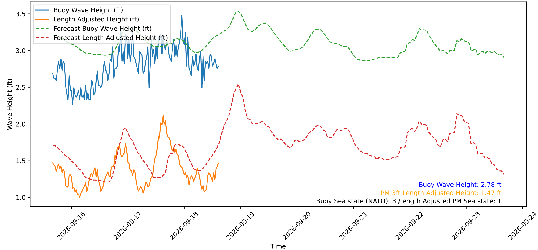
Wave Heights over Time for Green Beach at 2026-09-18 15:31:11
