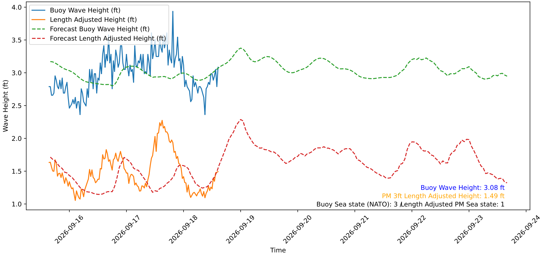
Wave Heights over Time for Oceanside Harbor at 2026-09-18 15:30:29
