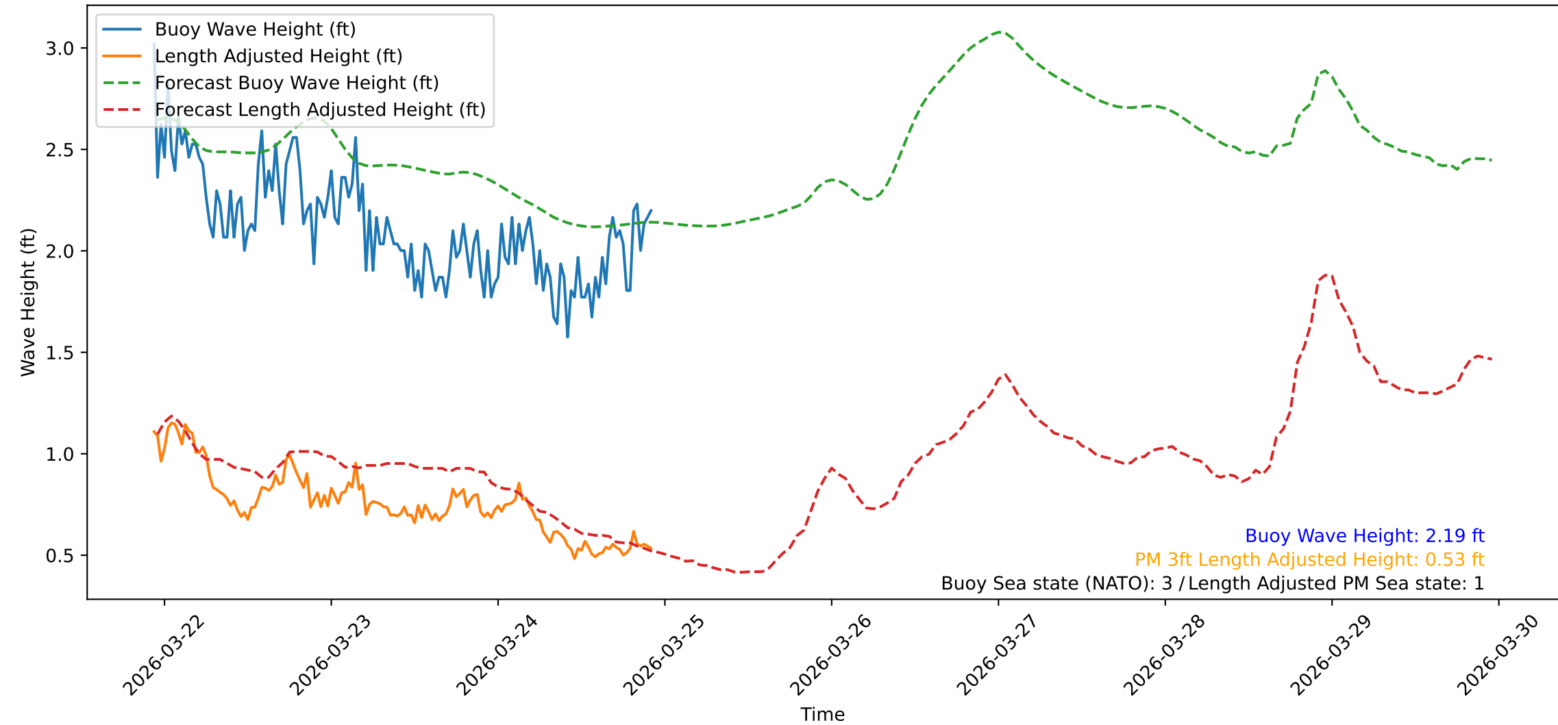
Wave Heights over Time for Oceanside Harbor at 2026-03-24 22:40:32
