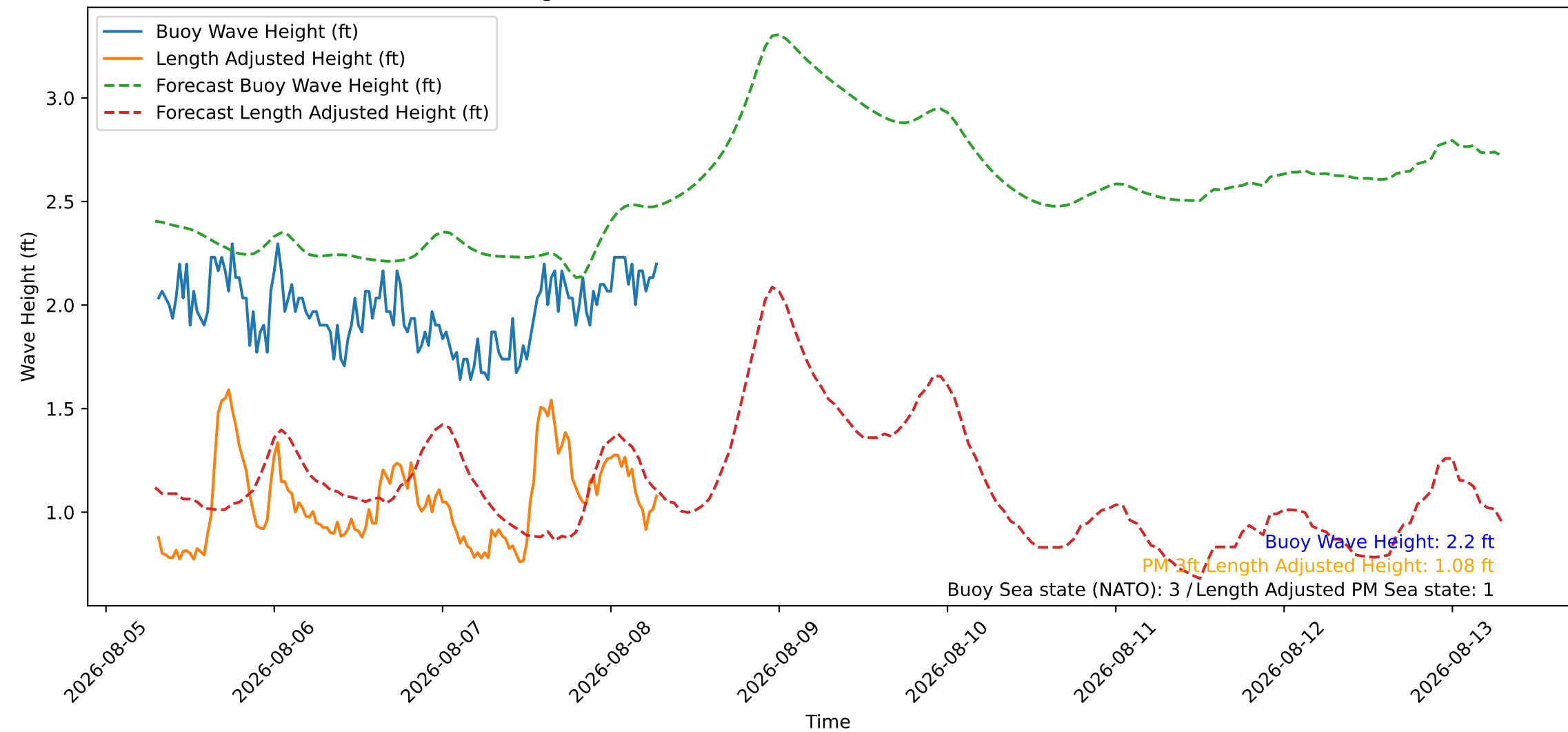
Wave Heights over Time for Oceanside Harbor at 2026-08-08 07:20:27
