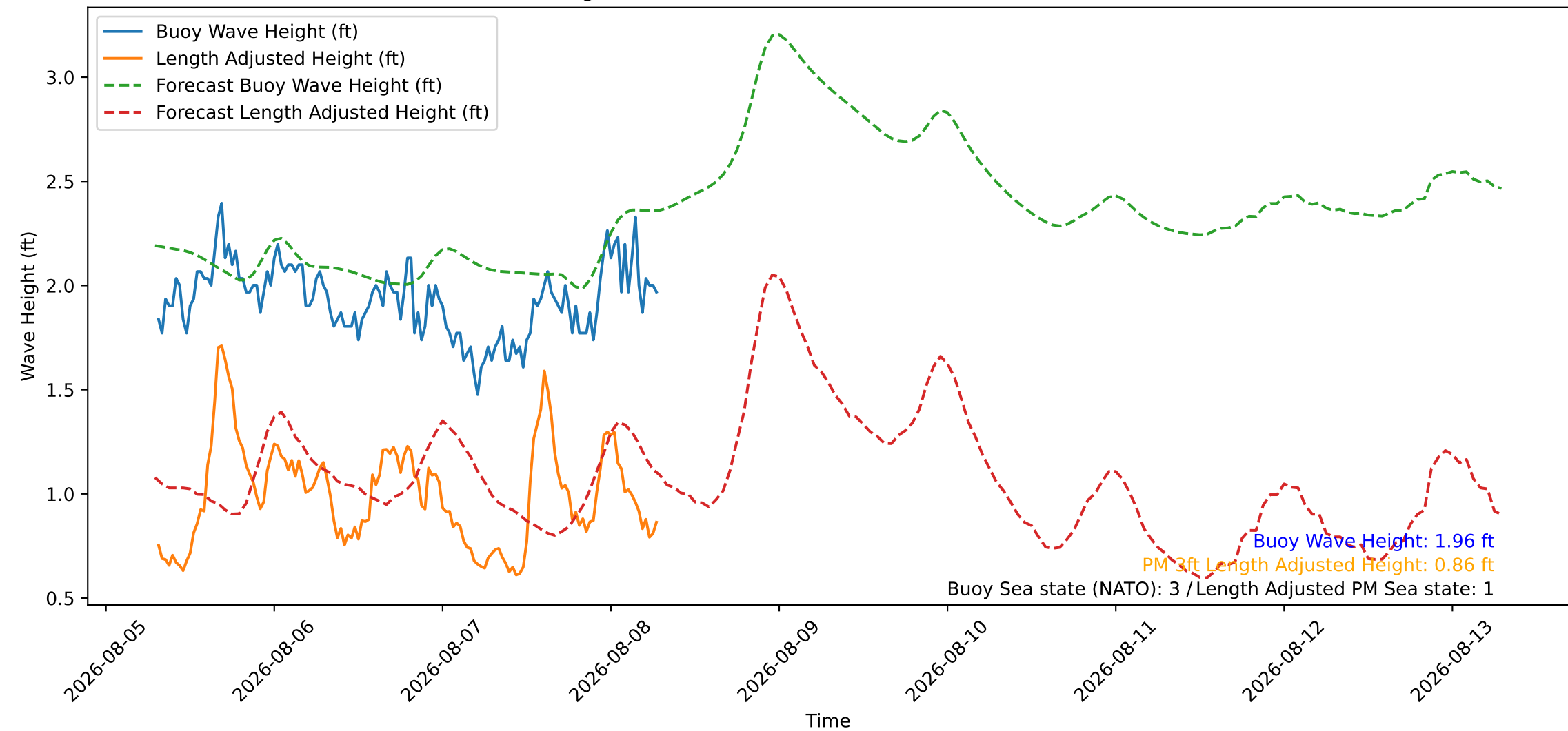
Wave Heights over Time for Red Beach at 2026-08-08 07:20:48
