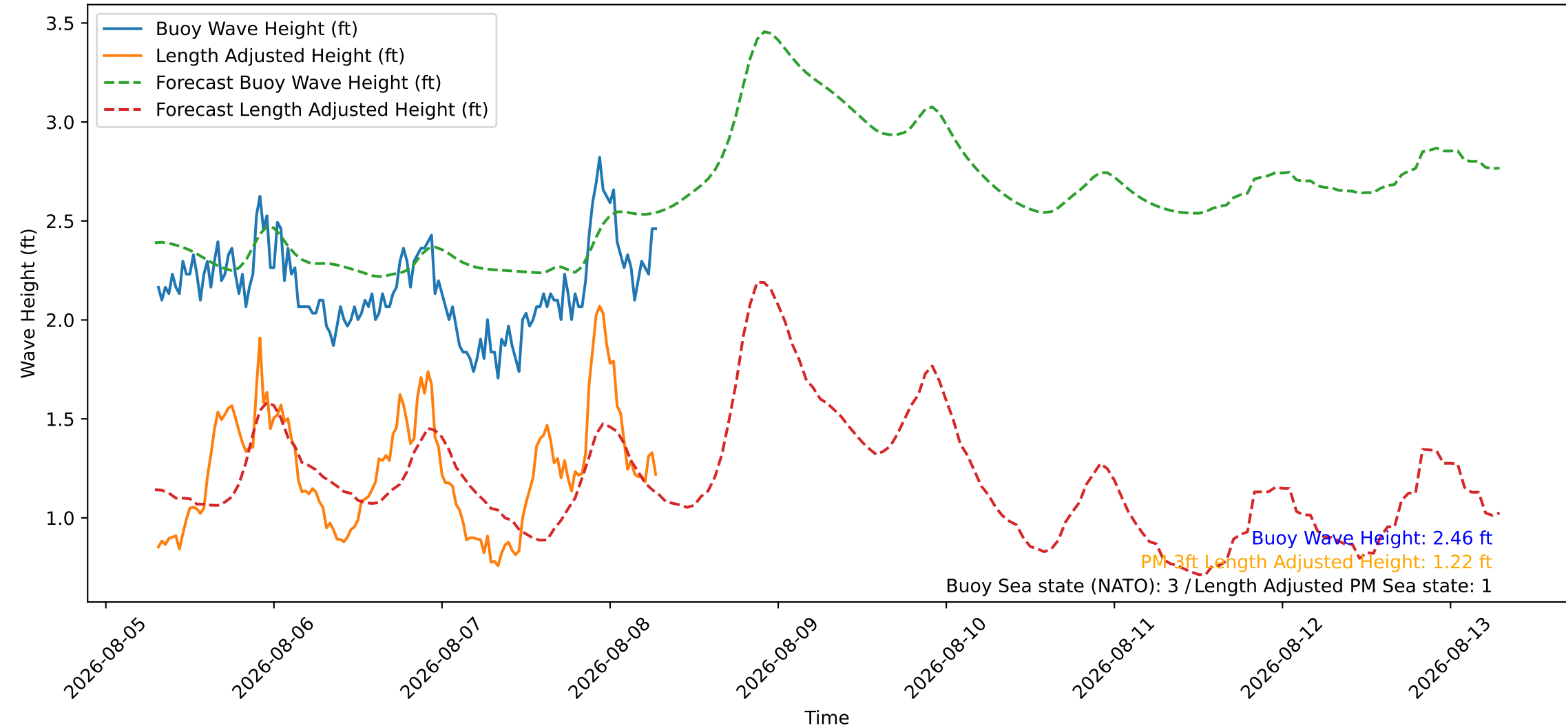
Wave Heights over Time for Green Beach at 2026-08-08 07:21:10
