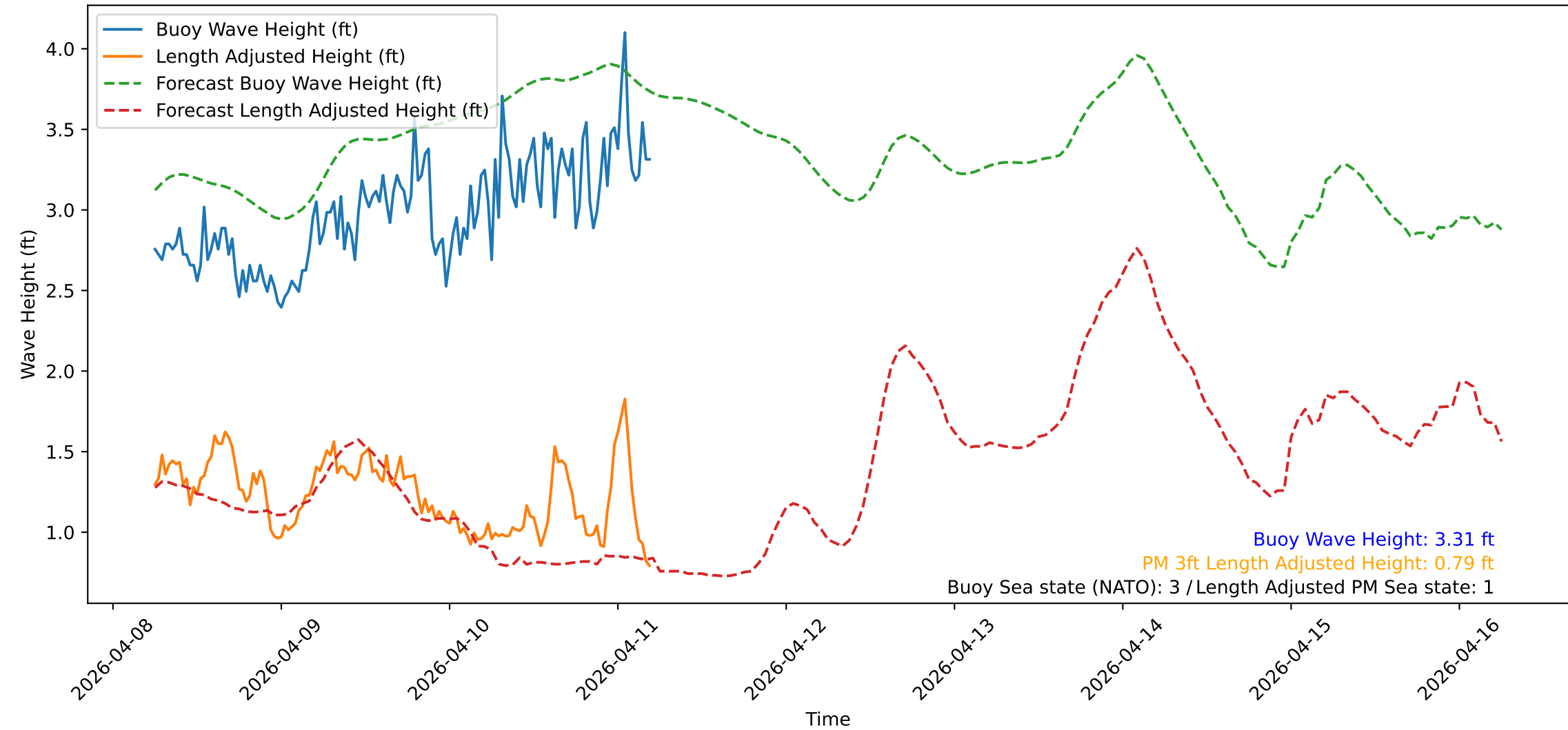
Wave Heights over Time for Red Beach at 2026-04-11 05:30:51
