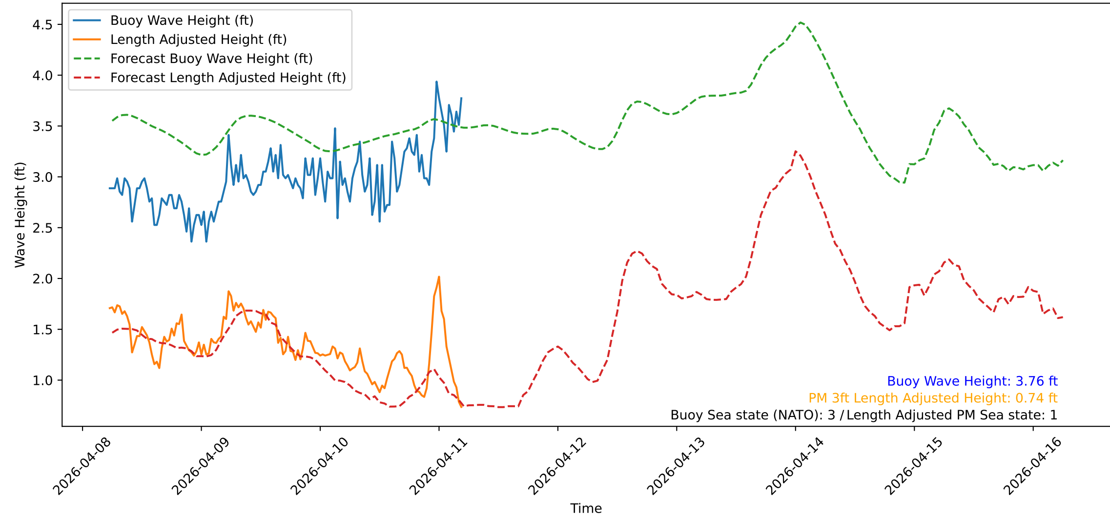
Wave Heights over Time for Green Beach at 2026-04-11 05:31:14
