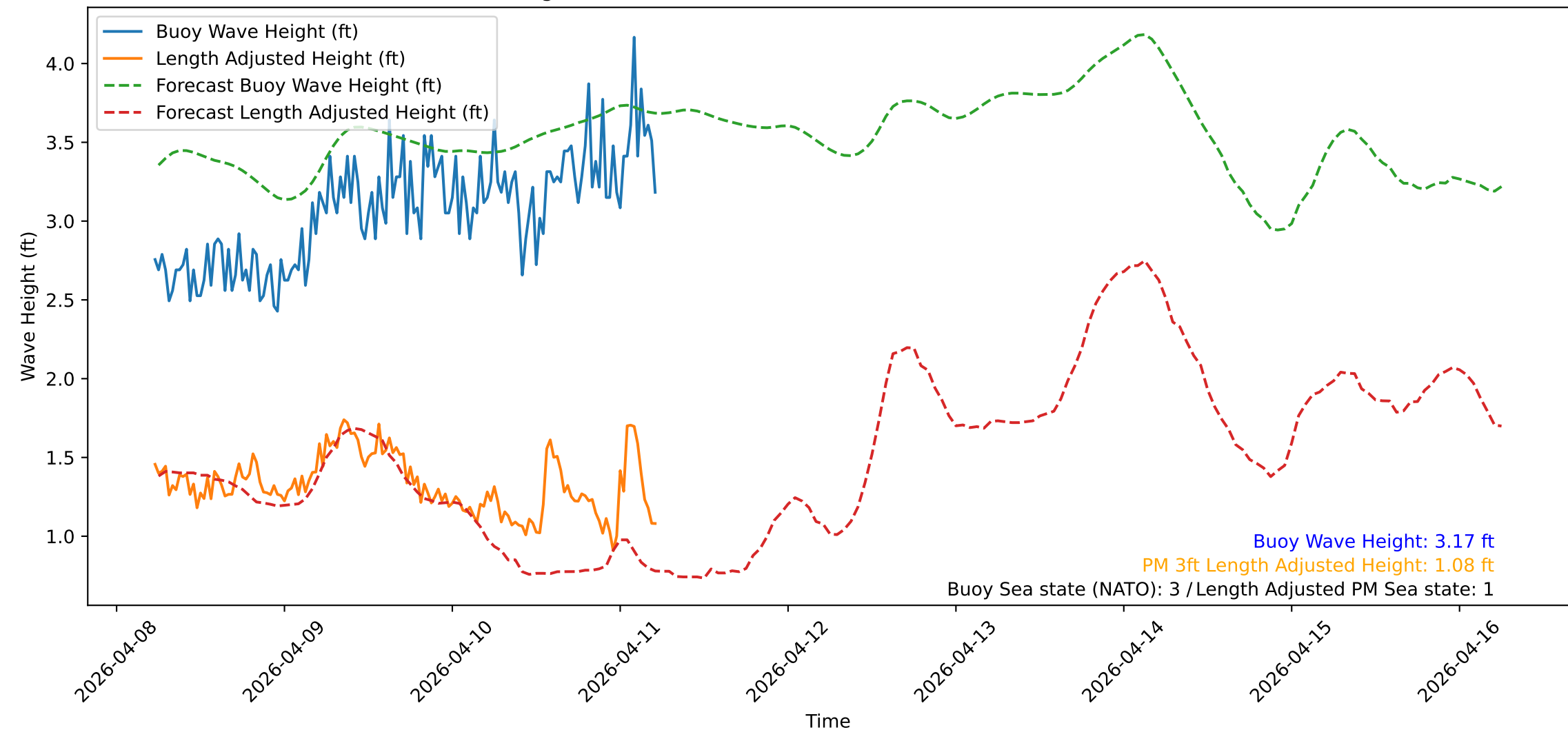
Wave Heights over Time for Oceanside Harbor at 2026-04-11 05:30:32
