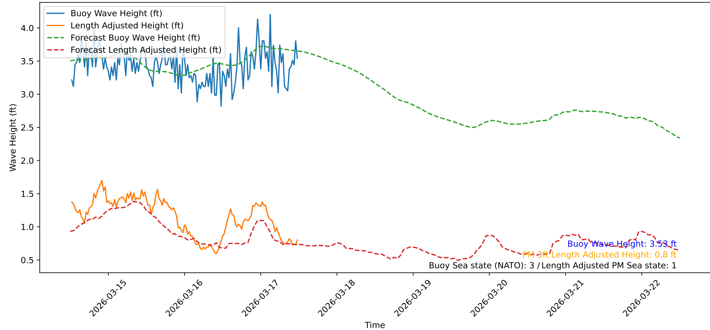
Wave Heights over Time for Green Beach at 2026-03-17 12:21:42
