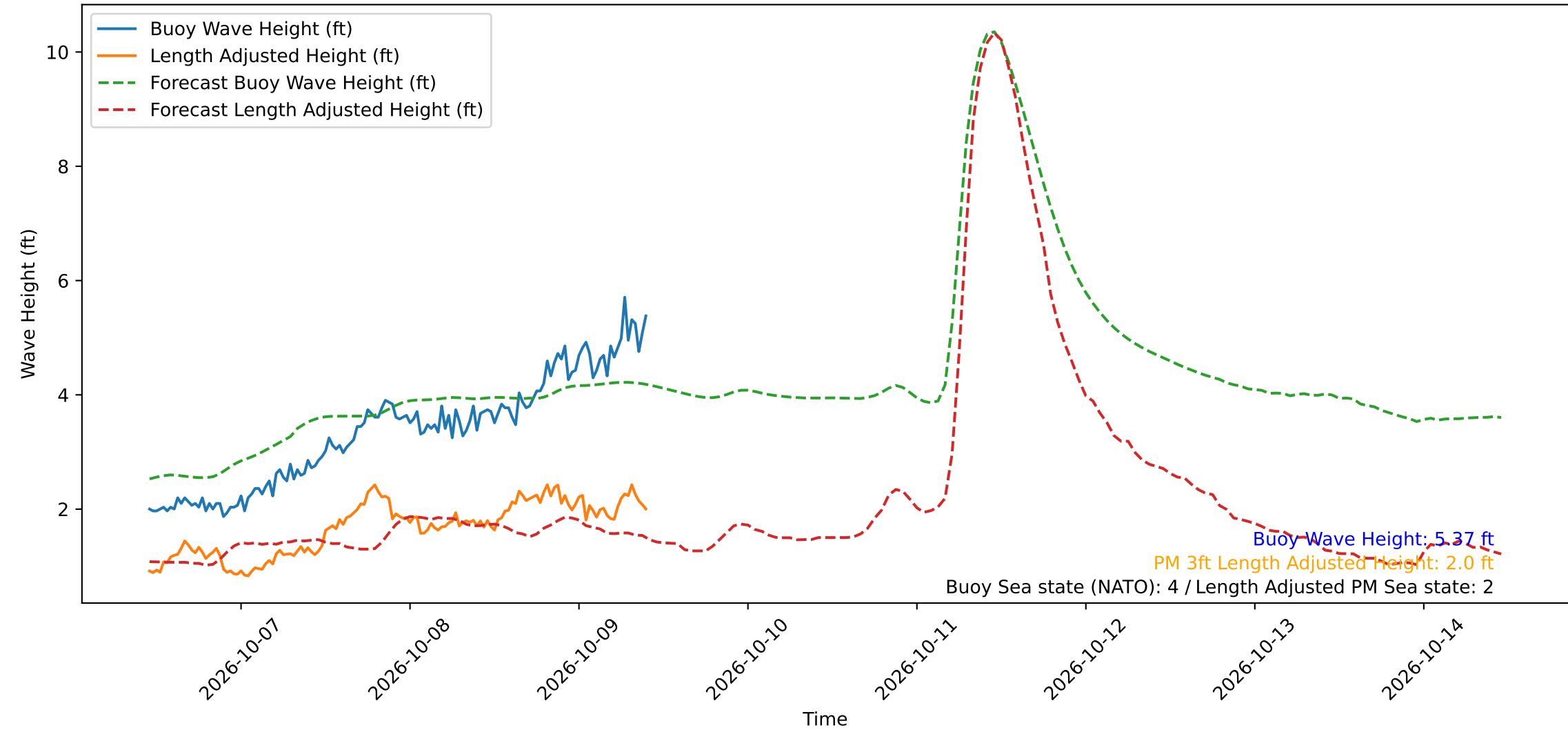
Wave Heights over Time for Red Beach at 2026-10-09 10:30:50
