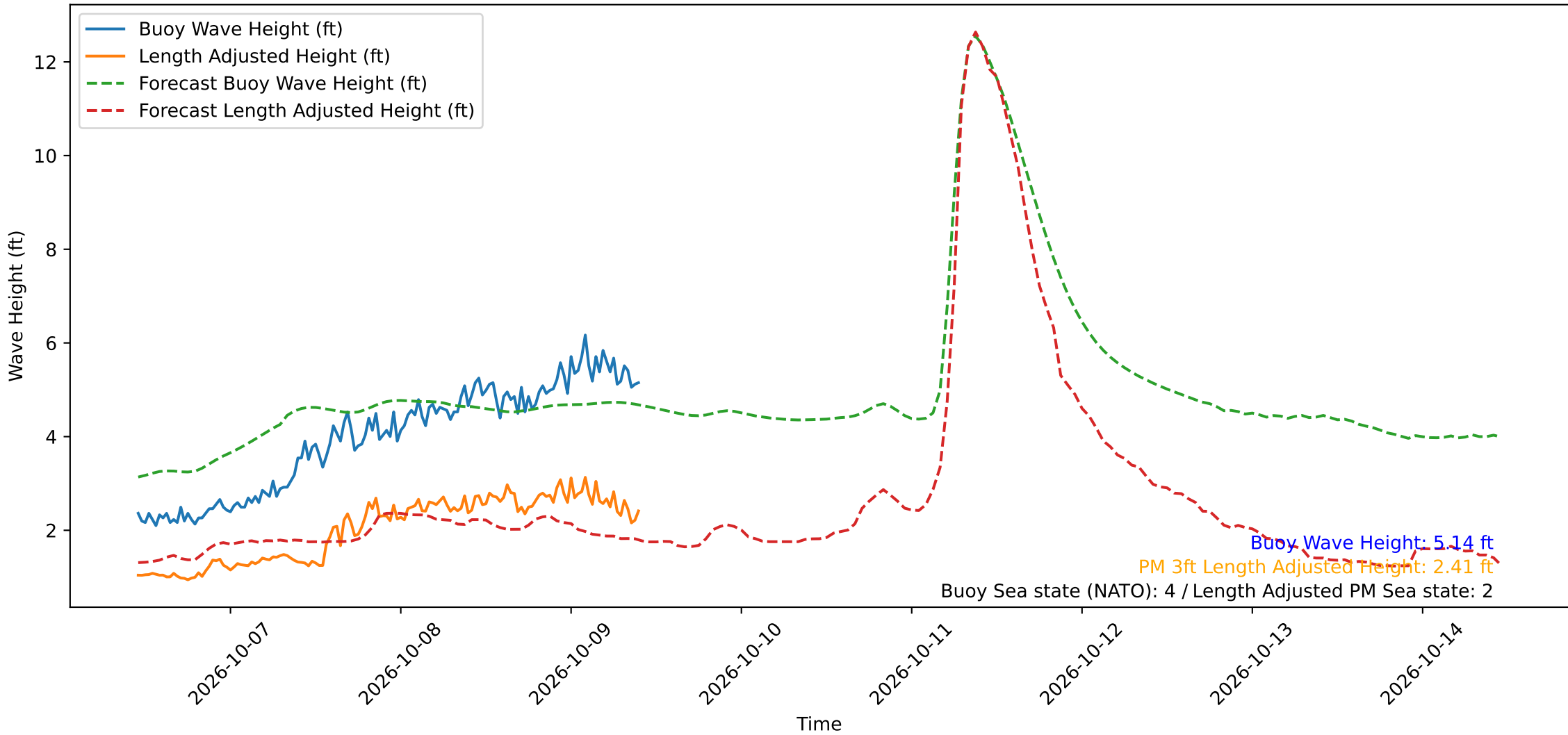
Wave Heights over Time for Green Beach at 2026-10-09 10:31:12
