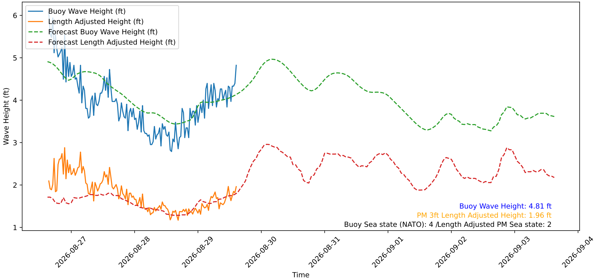
Wave Heights over Time for Oceanside Harbor at 2026-08-29 15:20:29
