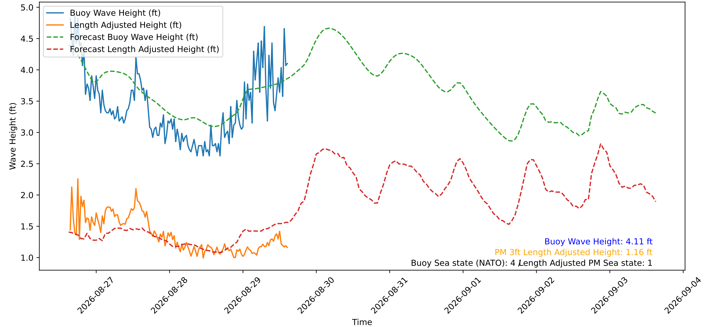
Wave Heights over Time for Red Beach at 2026-08-29 15:20:49
