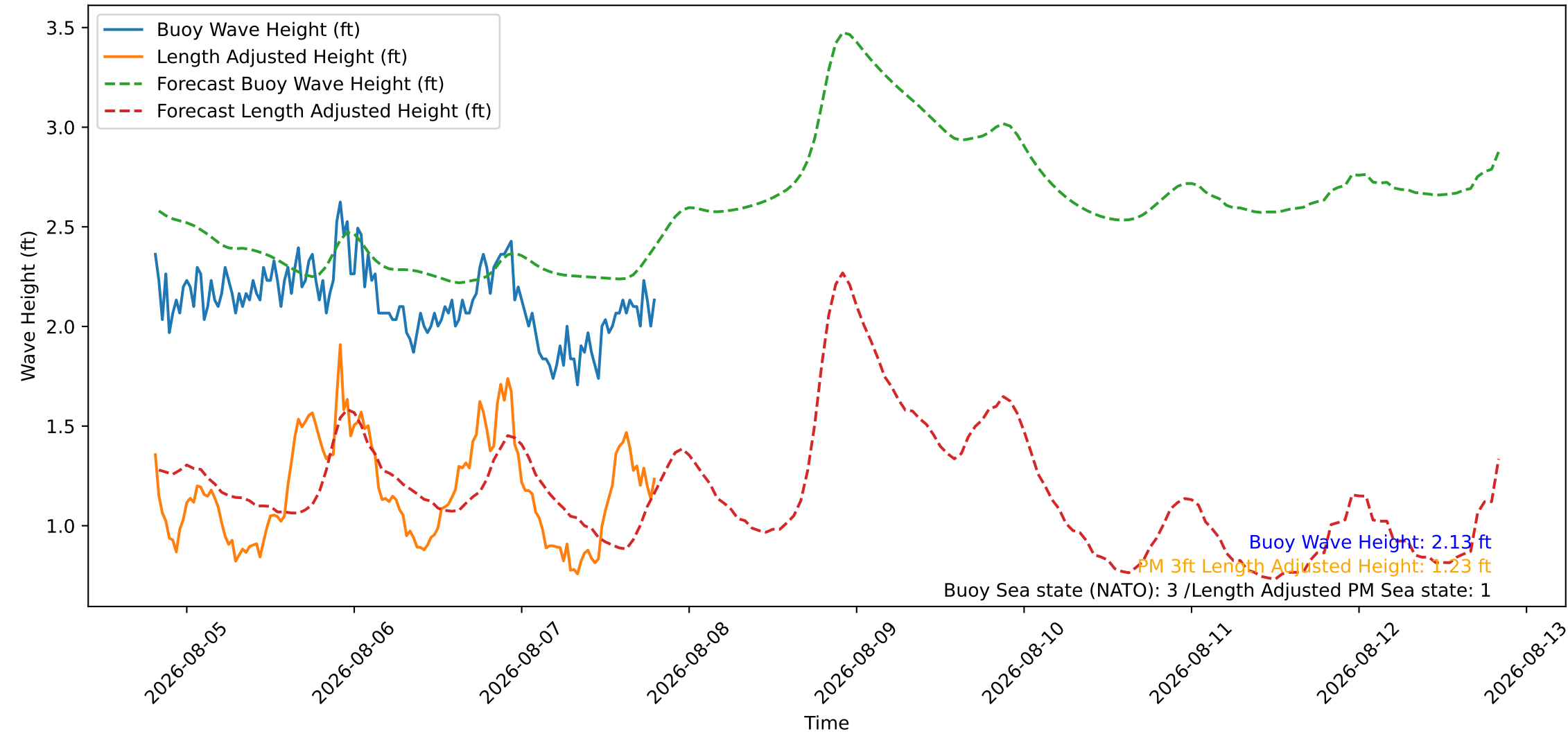
Wave Heights over Time for Green Beach at 2026-08-07 19:41:08
