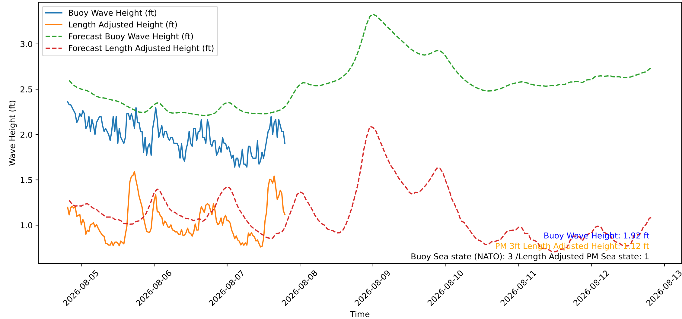
Wave Heights over Time for Oceanside Harbor at 2026-08-07 19:40:26
