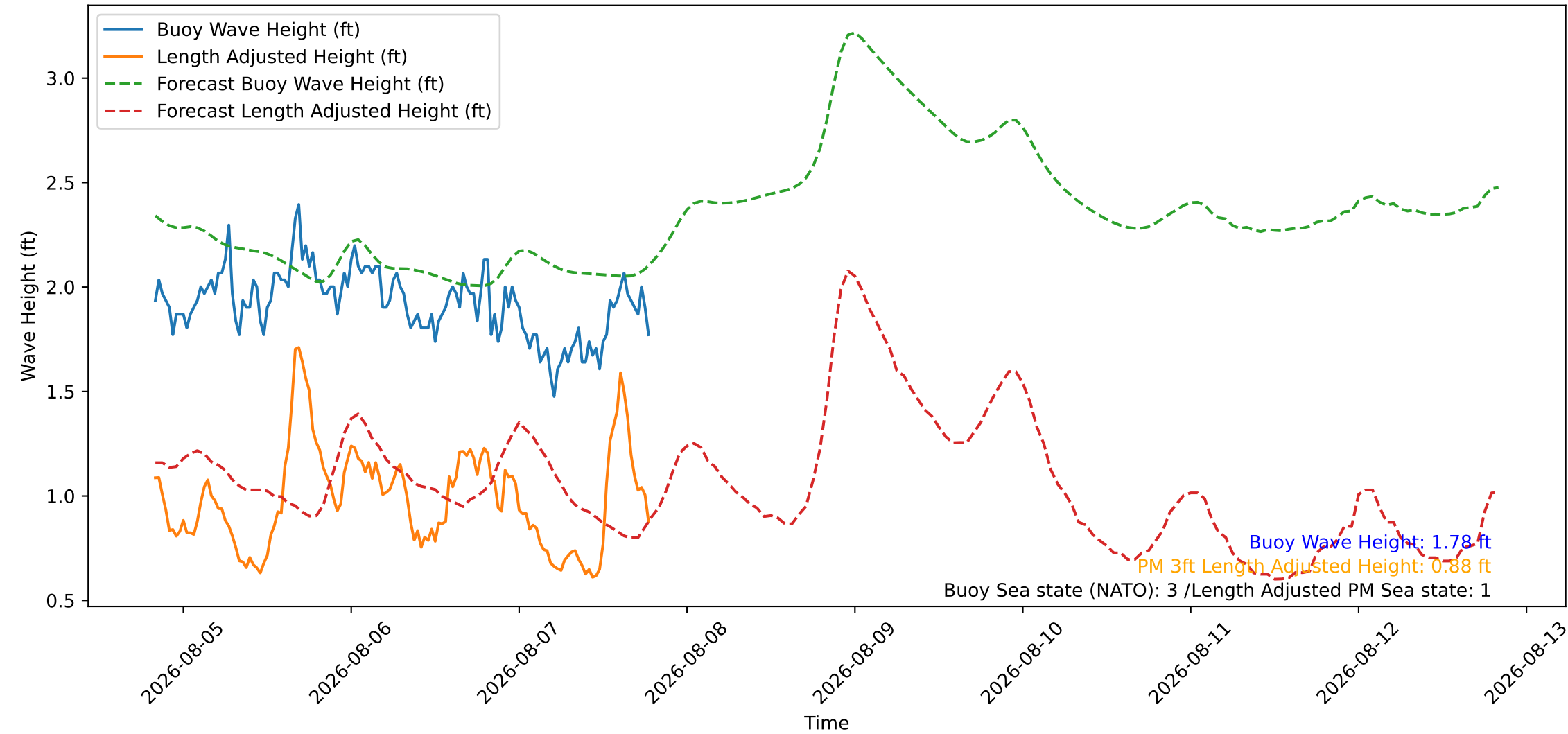
Wave Heights over Time for Red Beach at 2026-08-07 19:40:46
