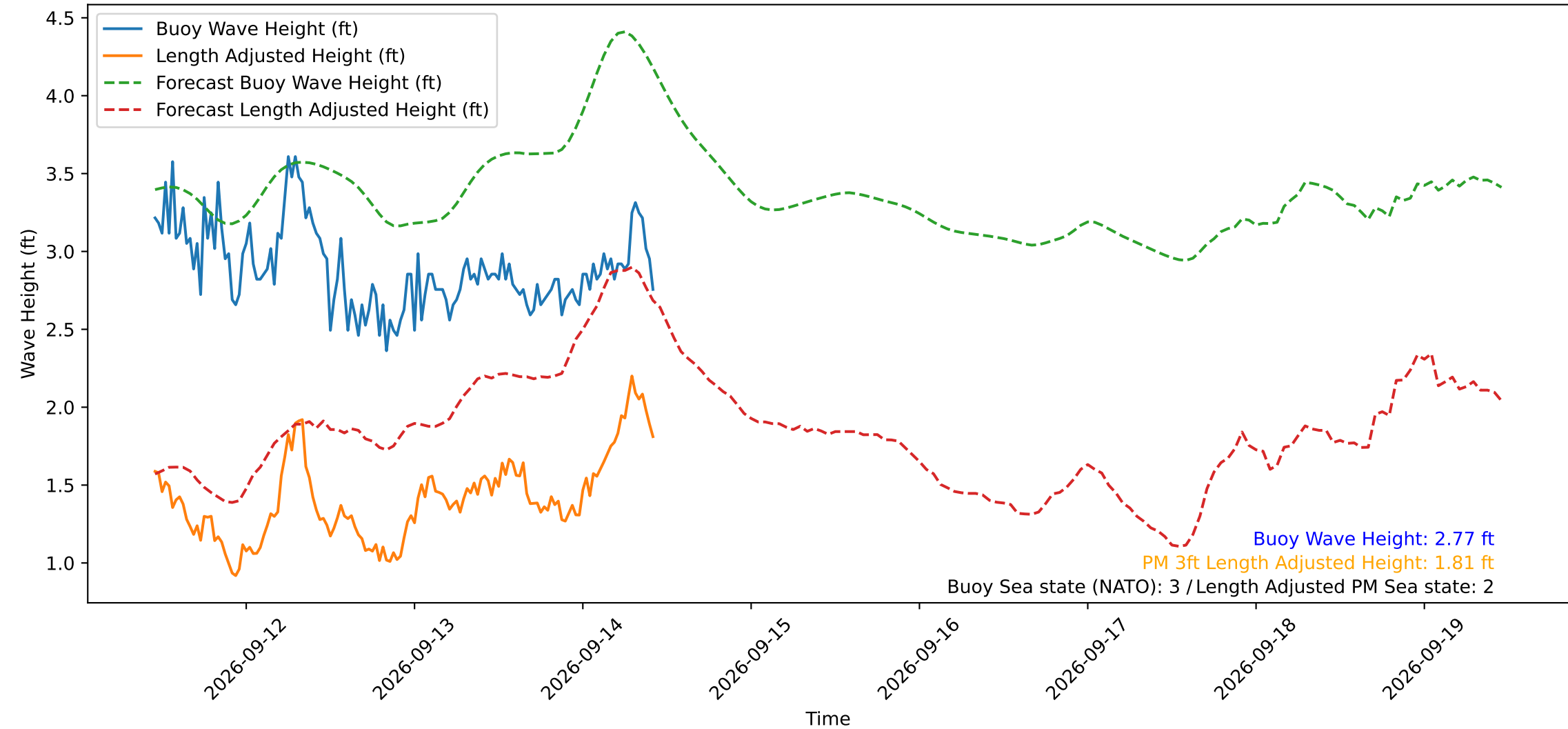
Wave Heights over Time for Green Beach at 2026-09-14 10:51:14
