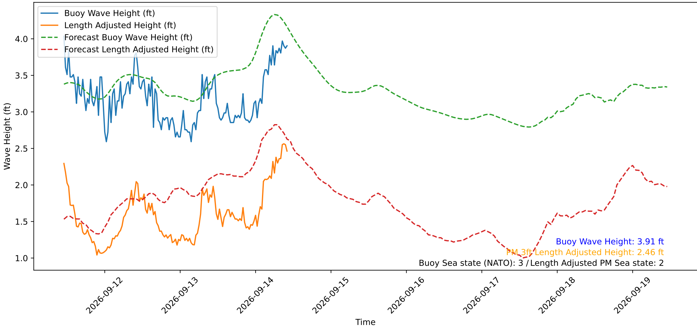
Wave Heights over Time for Oceanside Harbor at 2026-09-14 10:50:30
