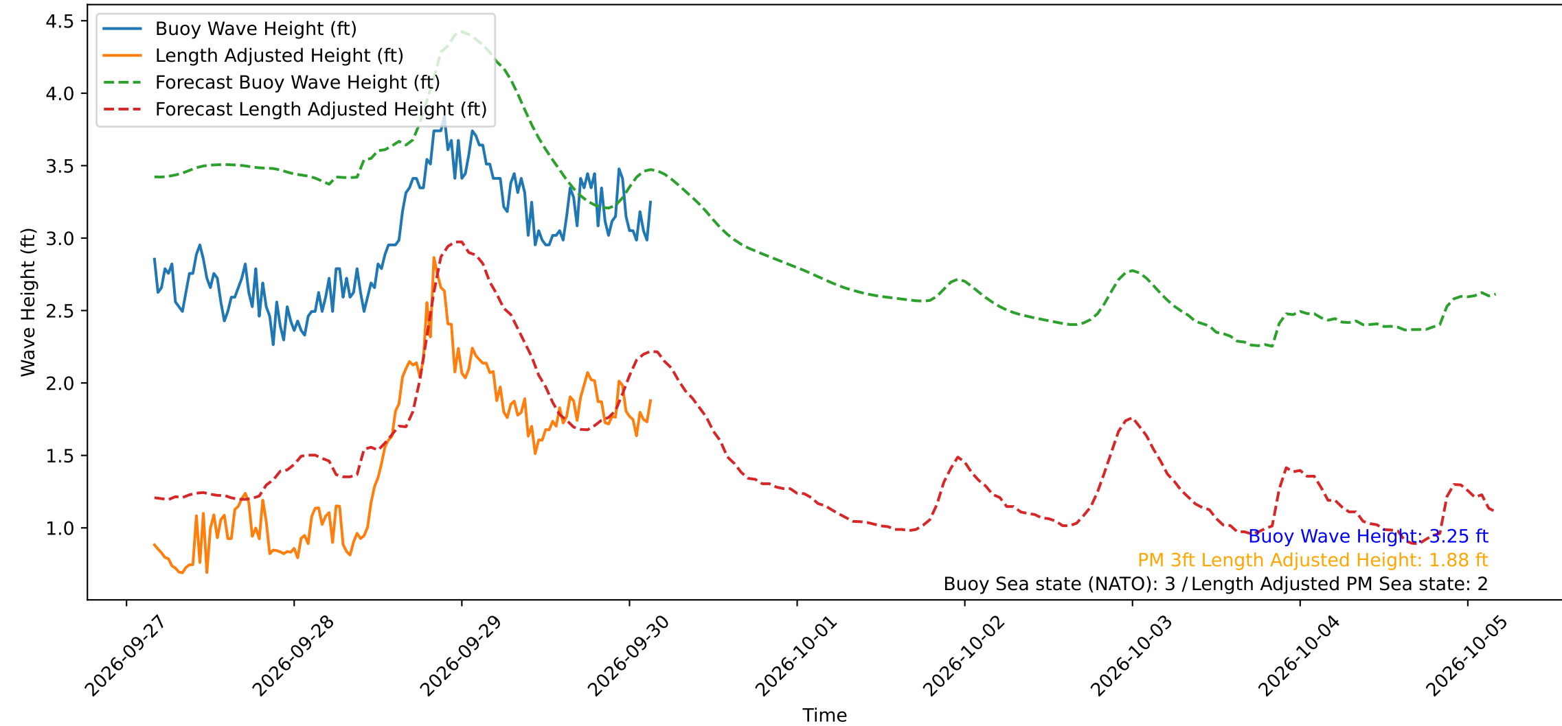
Wave Heights over Time for Red Beach at 2026-09-30 03:40:52
