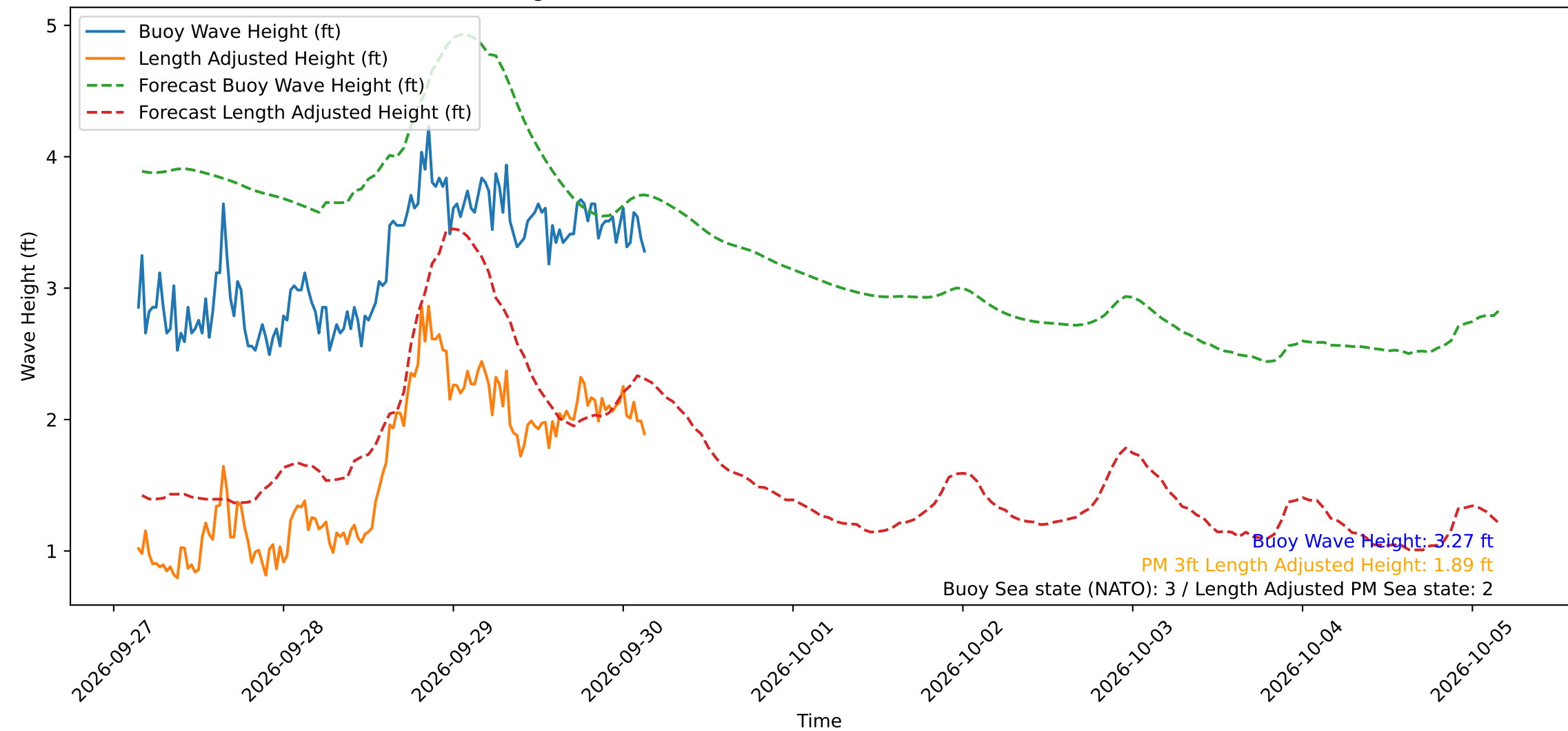
Wave Heights over Time for Oceanside Harbor at 2026-09-30 03:40:30
