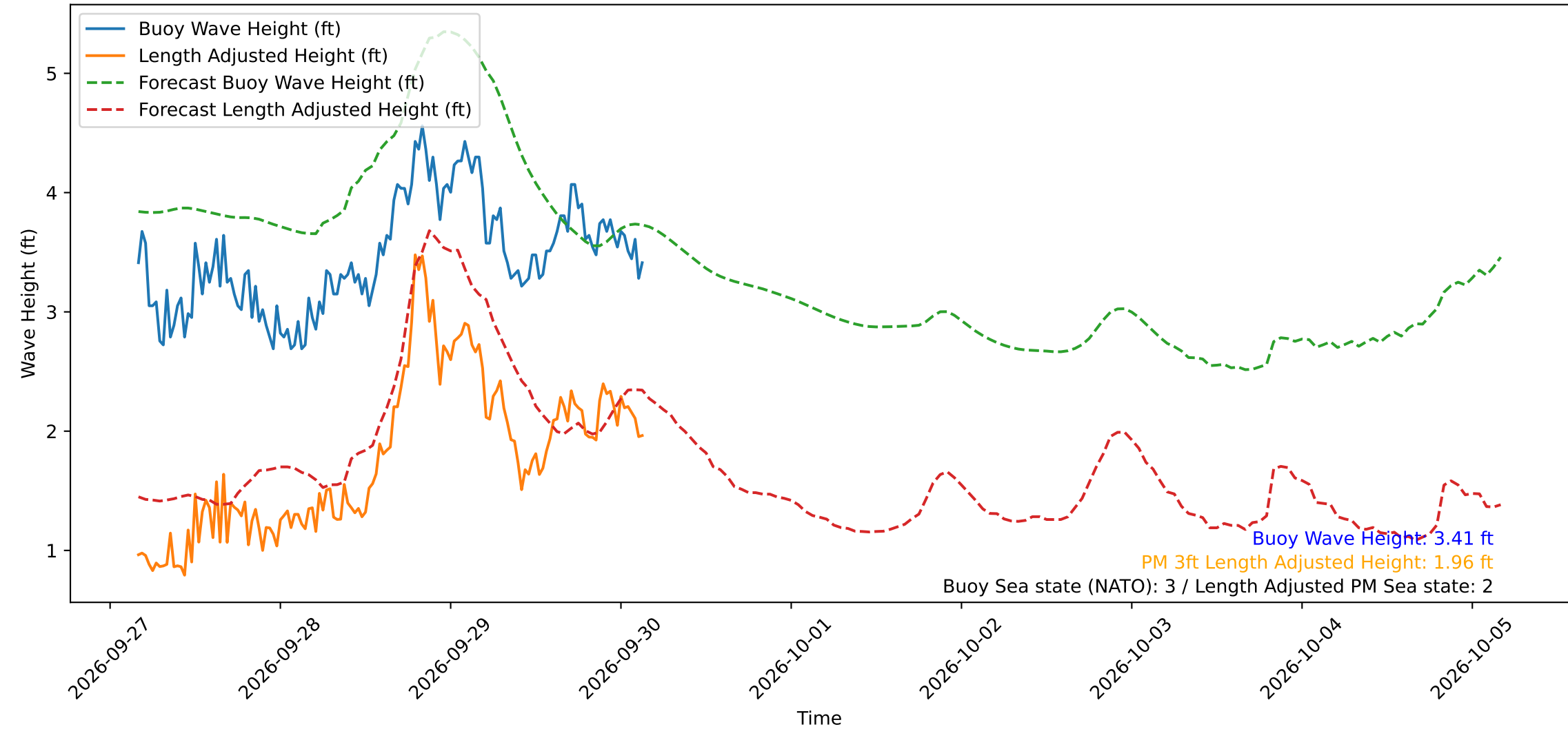
Wave Heights over Time for Green Beach at 2026-09-30 03:41:14
