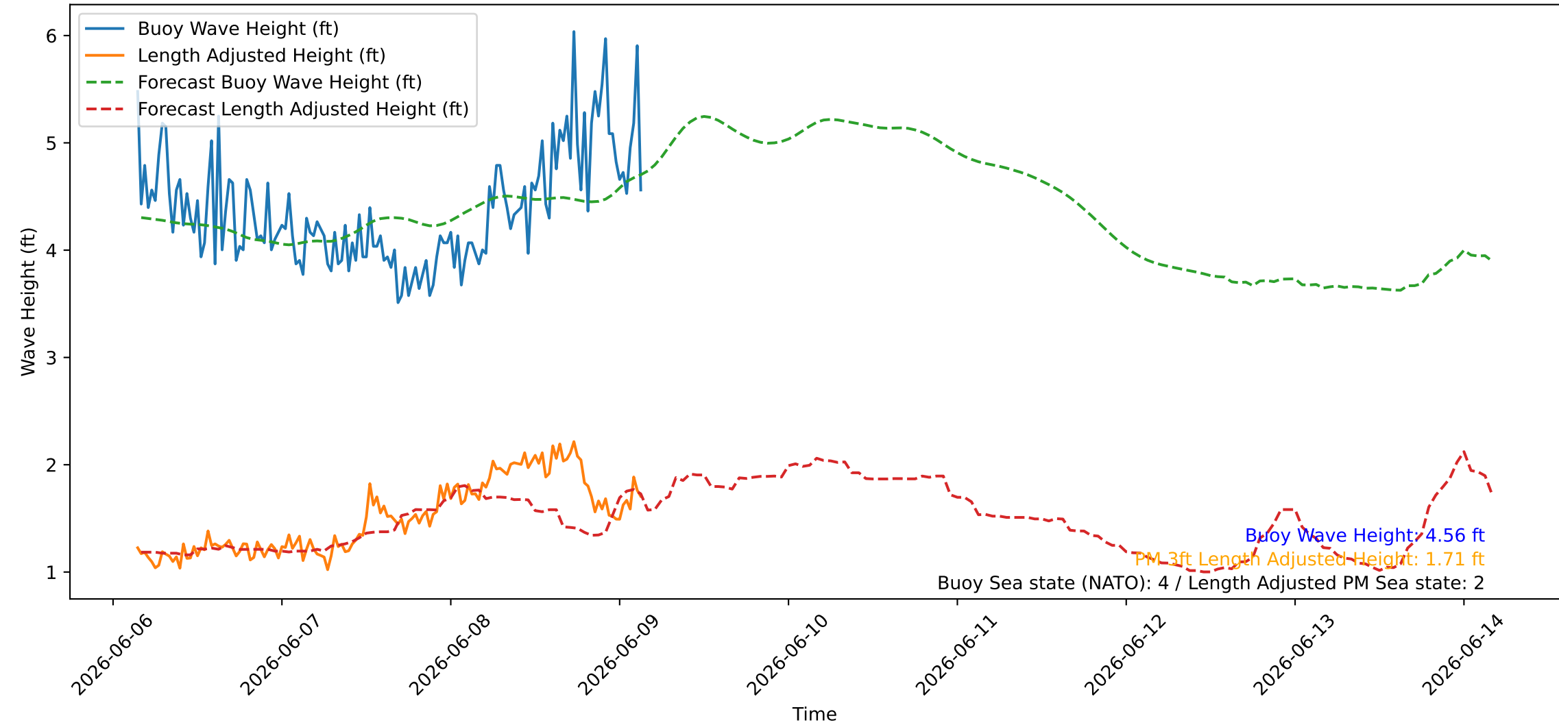
Wave Heights over Time for Oceanside Harbor at 2026-06-09 03:30:26
