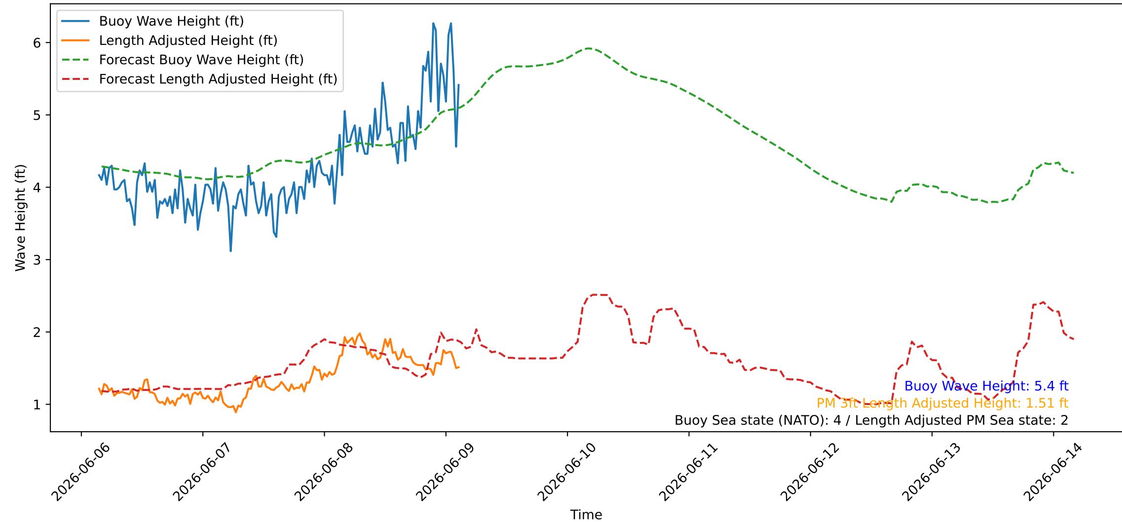
Wave Heights over Time for Green Beach at 2026-06-09 03:31:09
