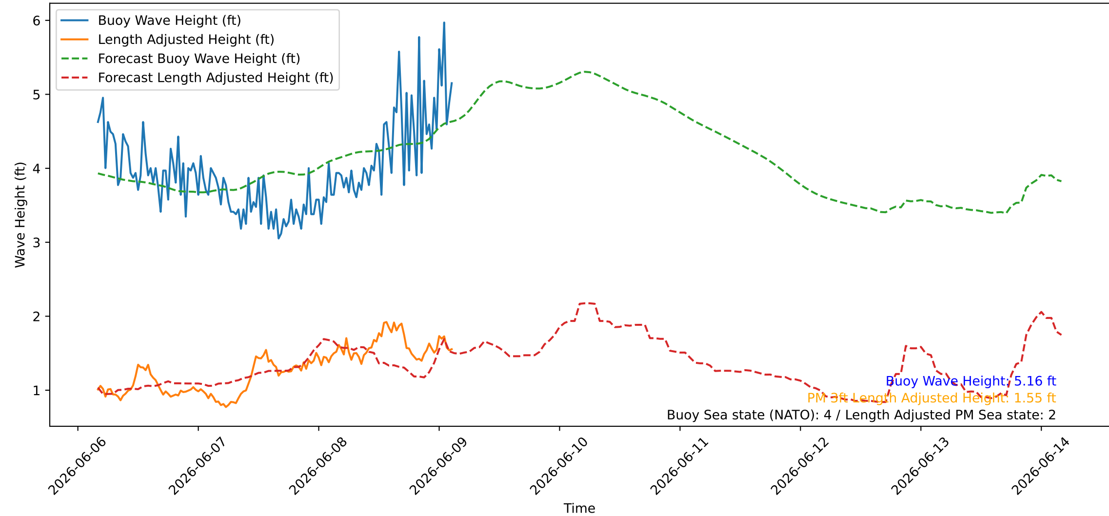
Wave Heights over Time for Red Beach at 2026-06-09 03:30:45
