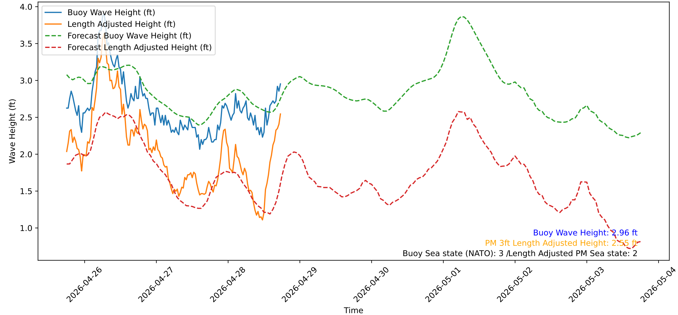
Wave Heights over Time for Oceanside Harbor at 2026-04-28 18:10:31
