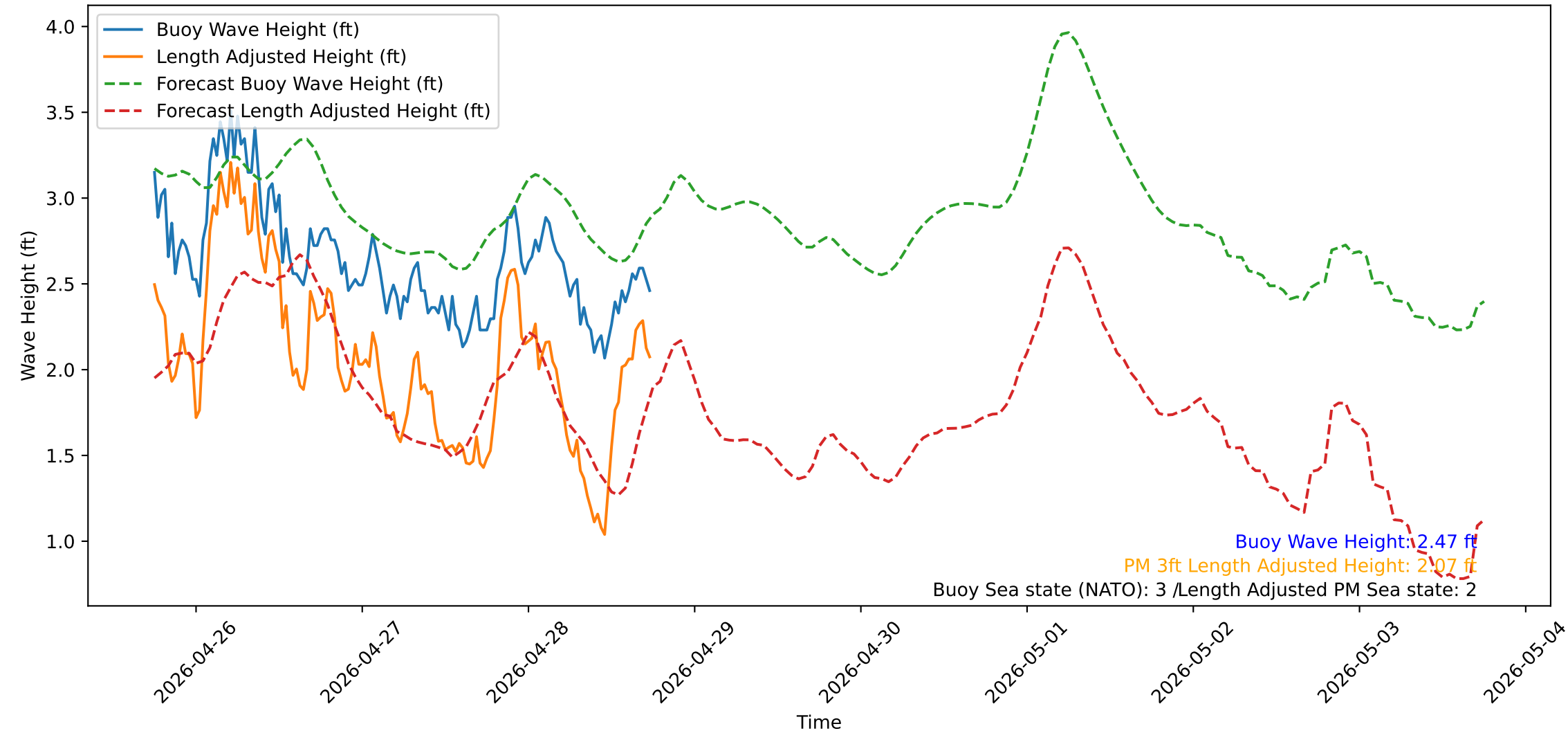
Wave Heights over Time for Green Beach at 2026-04-28 18:11:12
