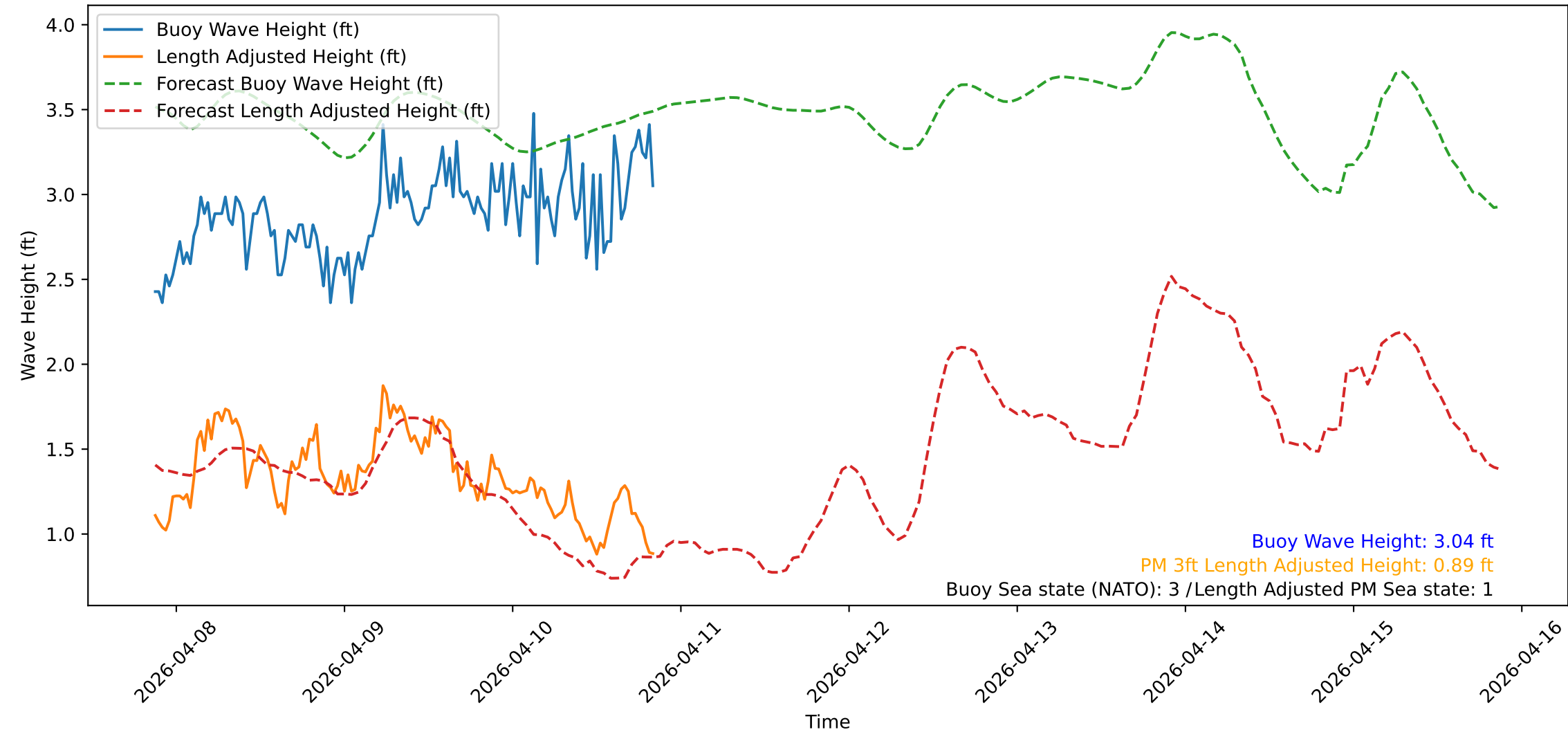
Wave Heights over Time for Green Beach at 2026-04-10 21:01:12
