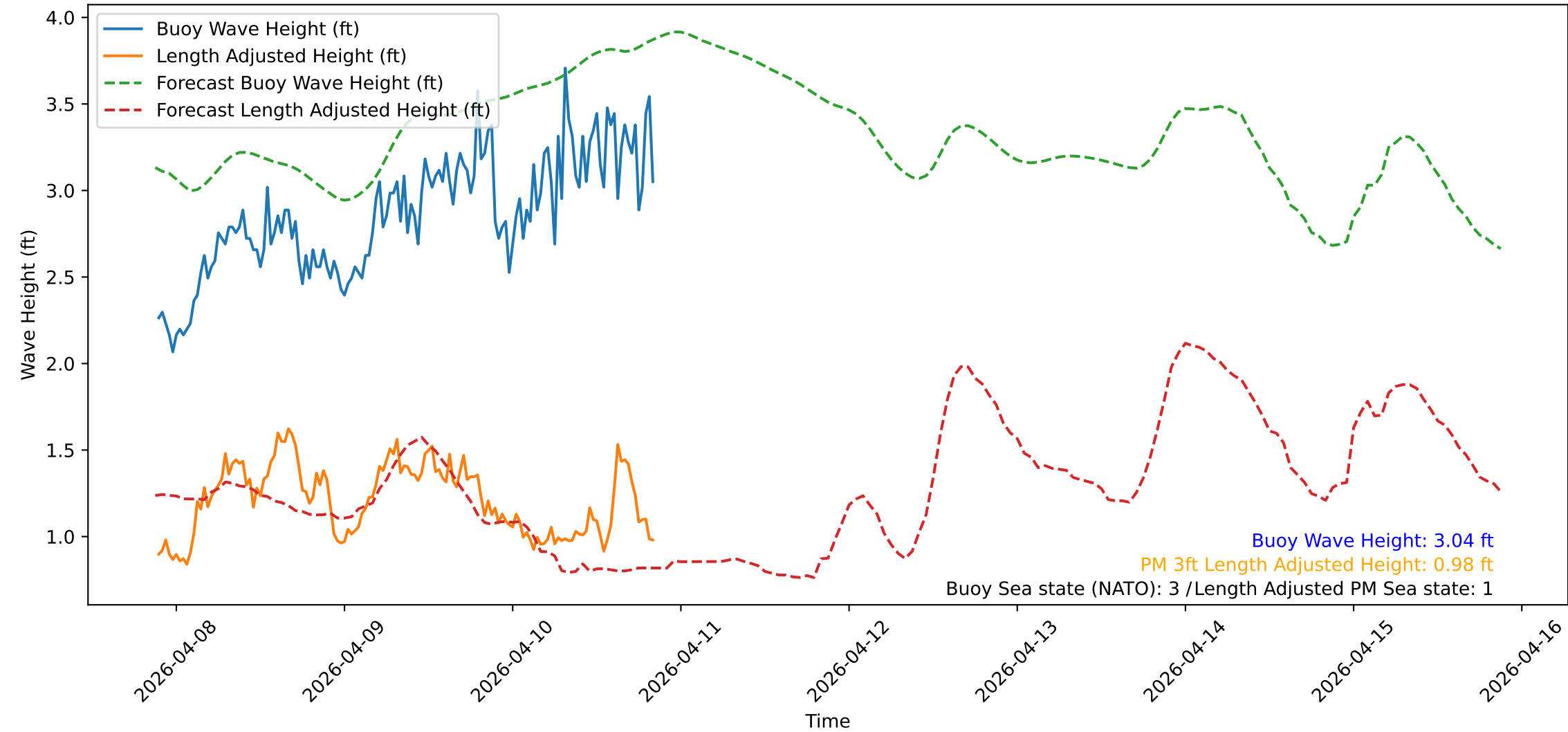
Wave Heights over Time for Red Beach at 2026-04-10 21:00:50
