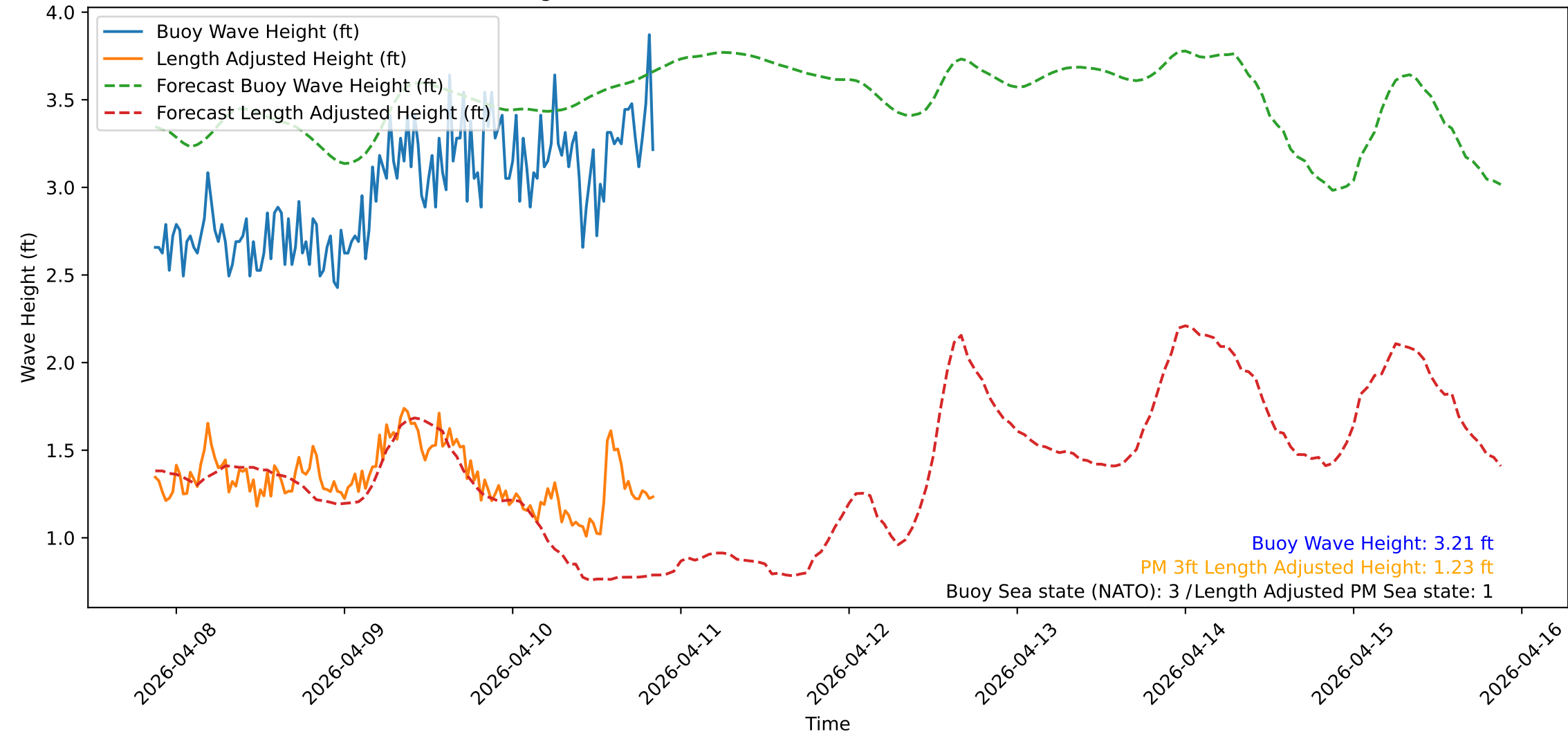
Wave Heights over Time for Oceanside Harbor at 2026-04-10 21:00:31
