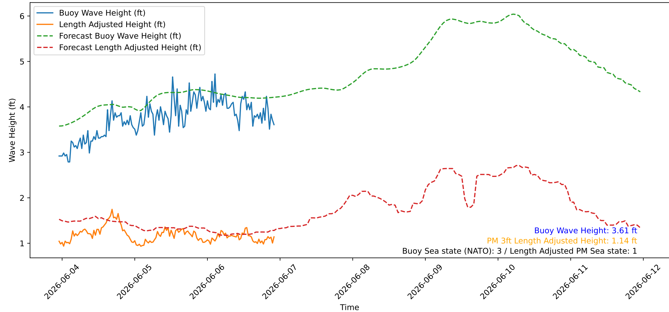
Wave Heights over Time for Green Beach at 2026-06-06 23:01:07
