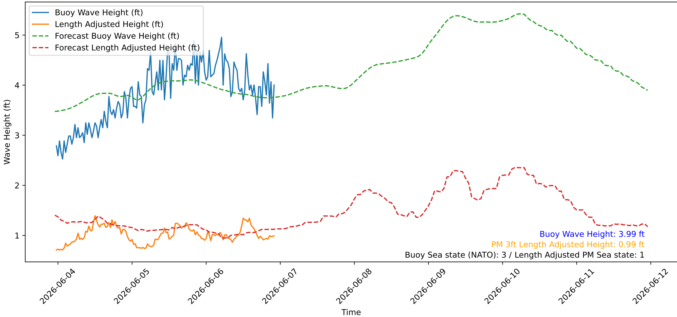
Wave Heights over Time for Red Beach at 2026-06-06 23:00:45
