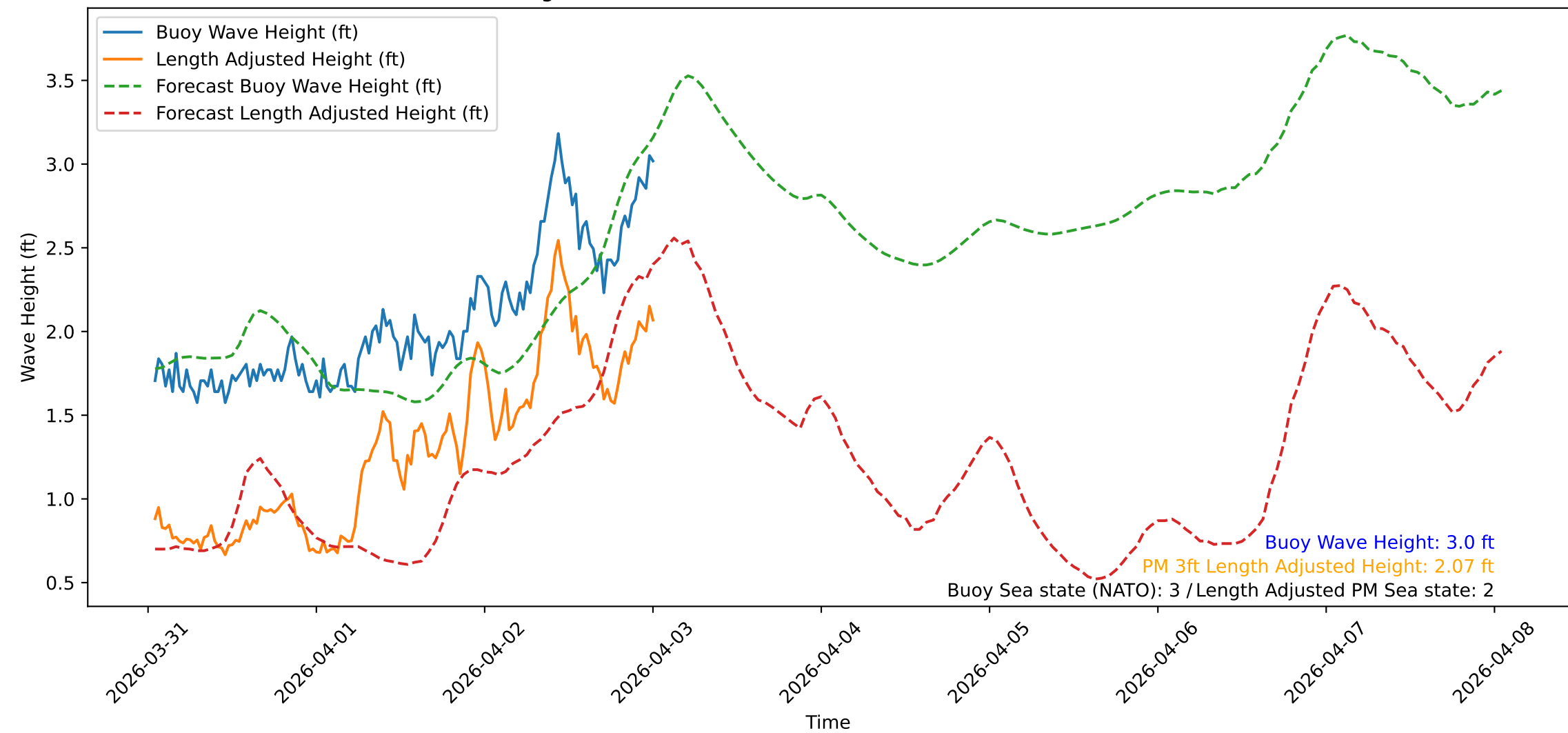
Wave Heights over Time for Oceanside Harbor at 2026-04-03 00:50:31
