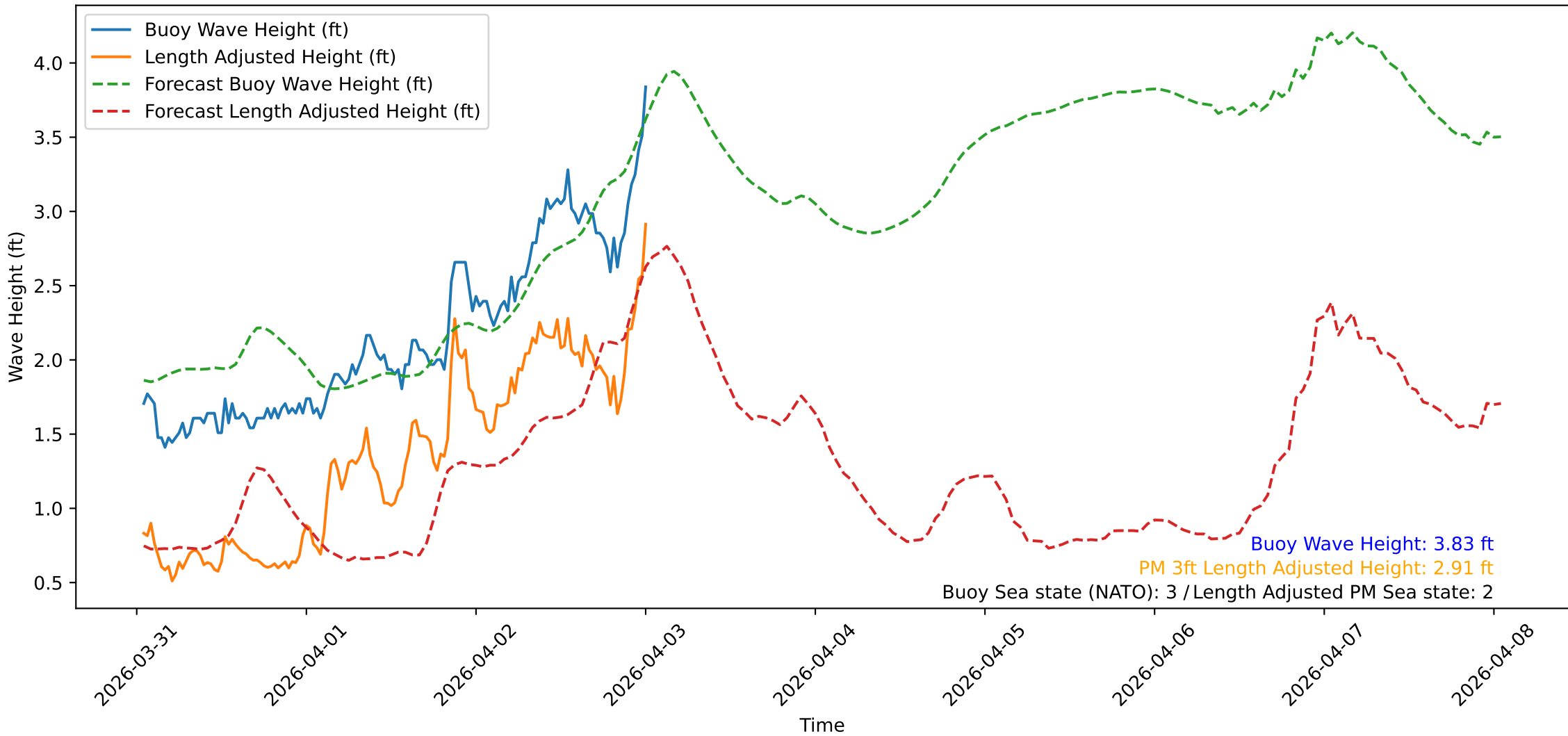
Wave Heights over Time for Green Beach at 2026-04-03 00:51:09
