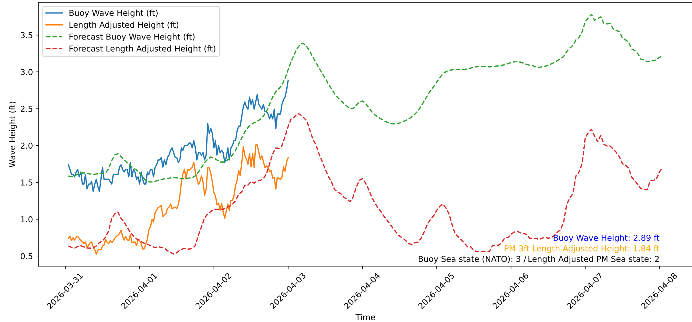
Wave Heights over Time for Red Beach at 2026-04-03 00:50:47
