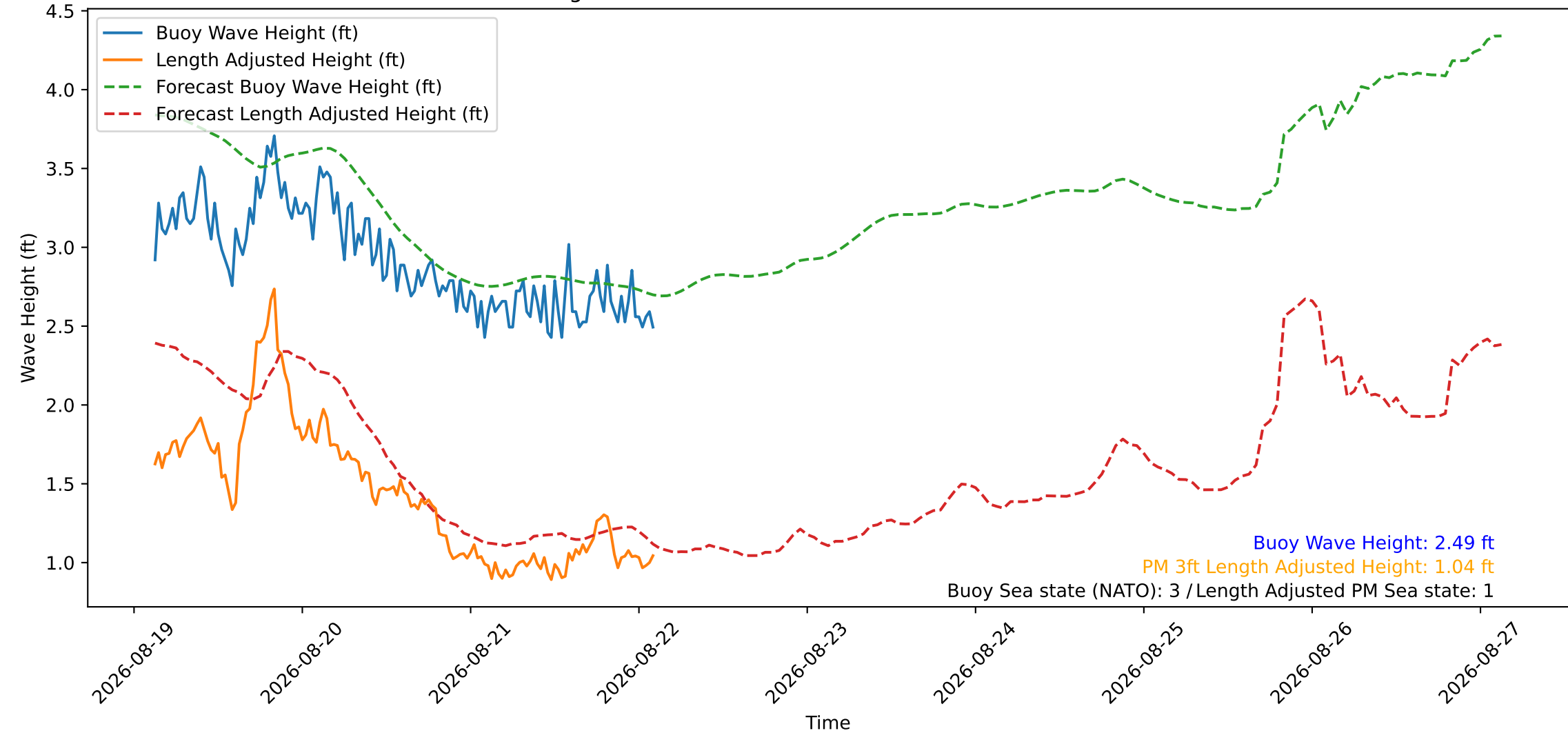
Wave Heights over Time for Green Beach at 2026-08-22 02:51:14
