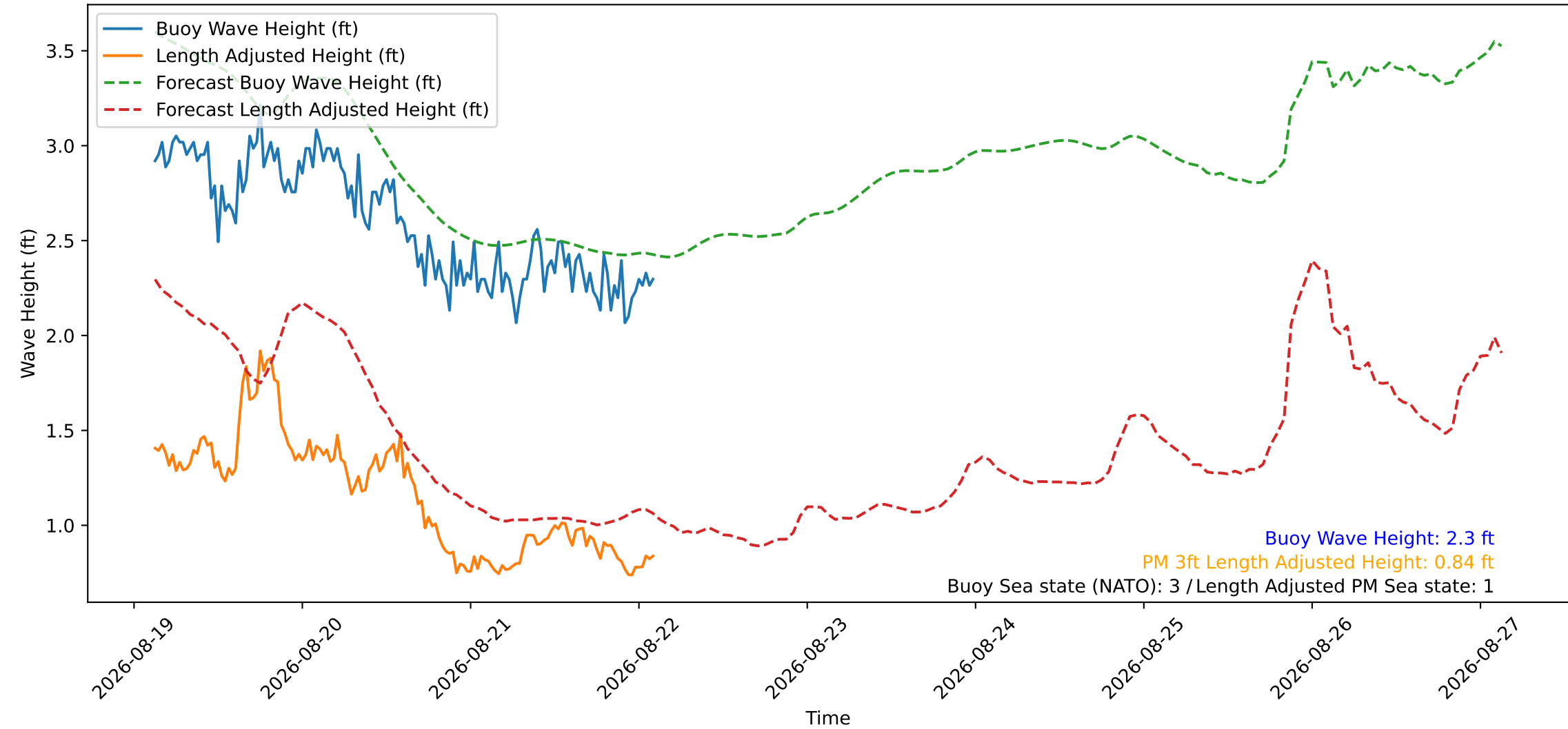
Wave Heights over Time for Red Beach at 2026-08-22 02:50:50
