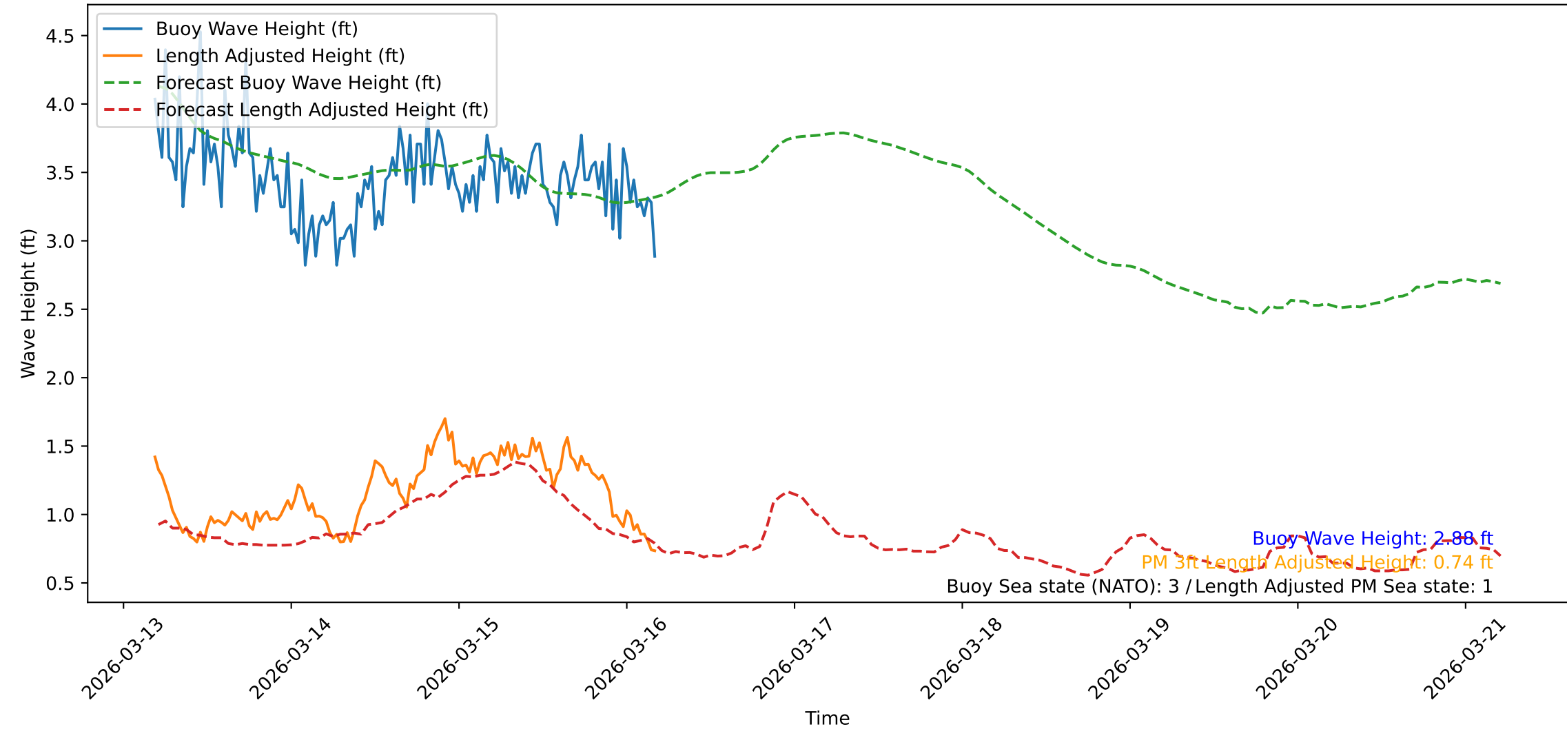
Wave Heights over Time for Green Beach at 2026-03-16 04:41:34
