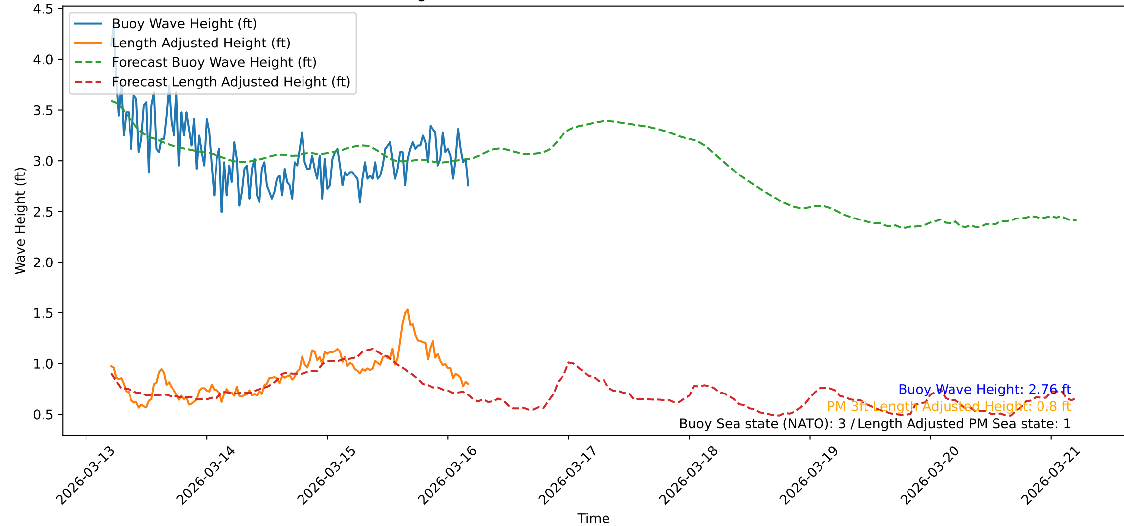
Wave Heights over Time for Red Beach at 2026-03-16 04:41:01
