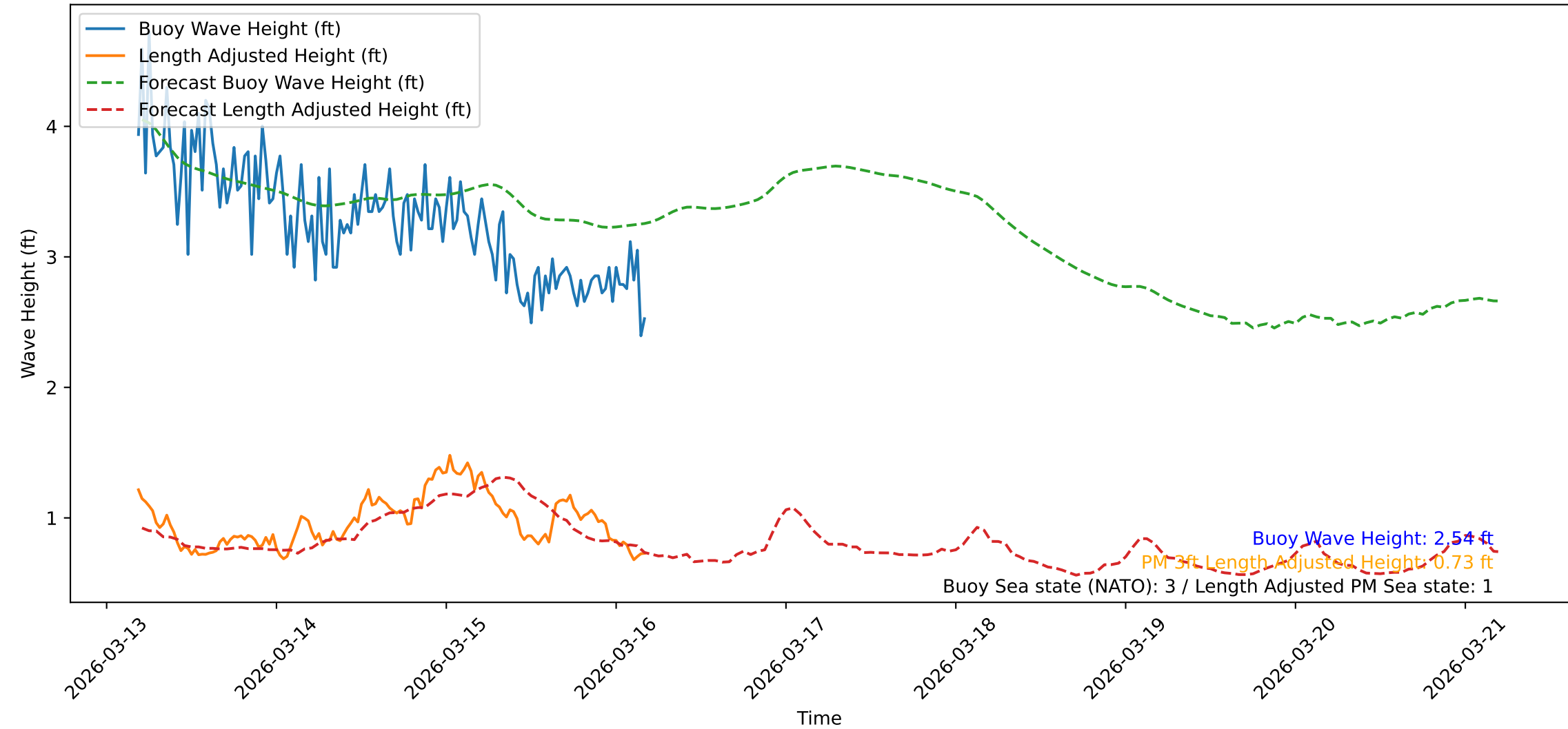
Wave Heights over Time for Oceanside Harbor at 2026-03-16 04:40:39
