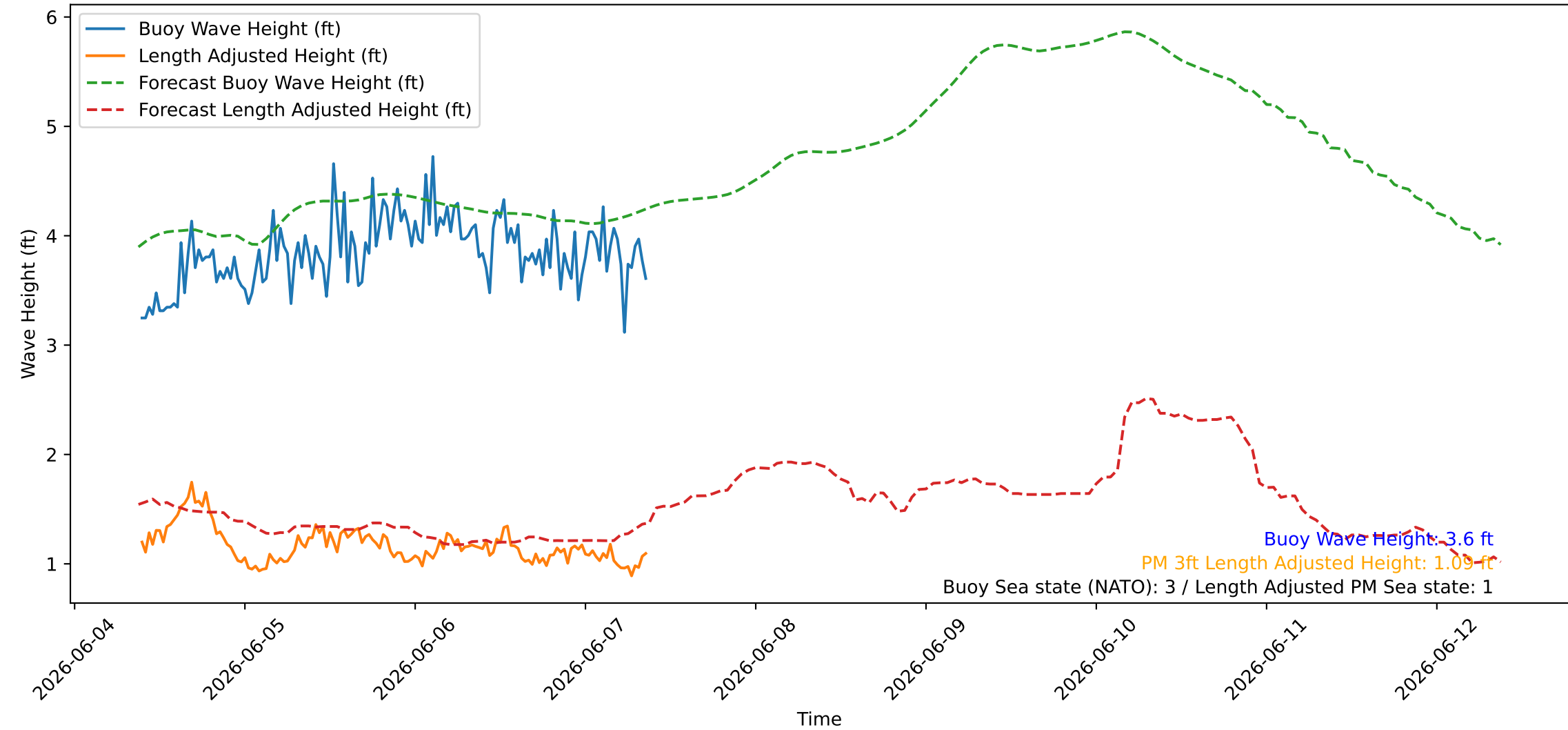
Wave Heights over Time for Green Beach at 2026-06-07 09:21:09
