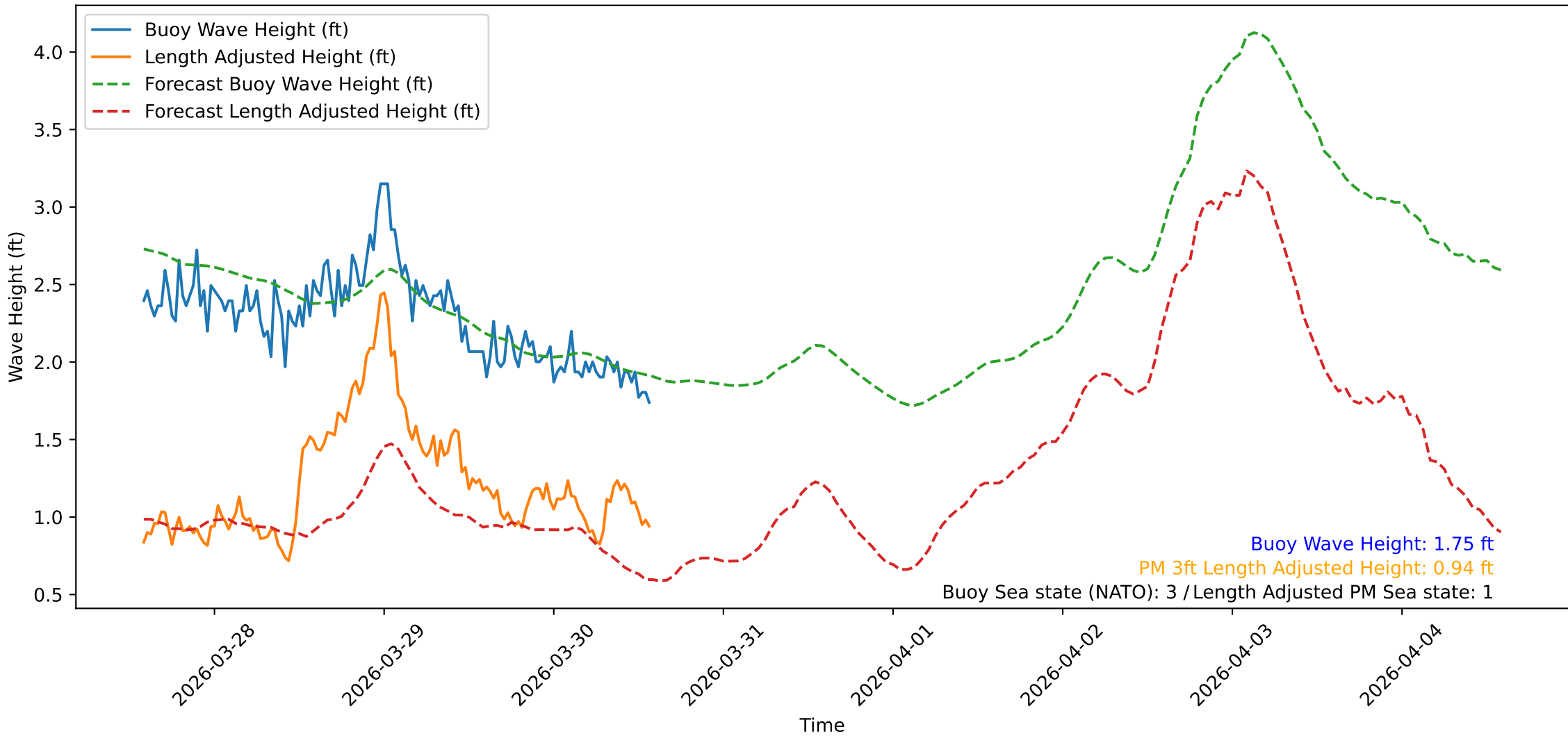
Wave Heights over Time for Oceanside Harbor at 2026-03-30 14:10:31
