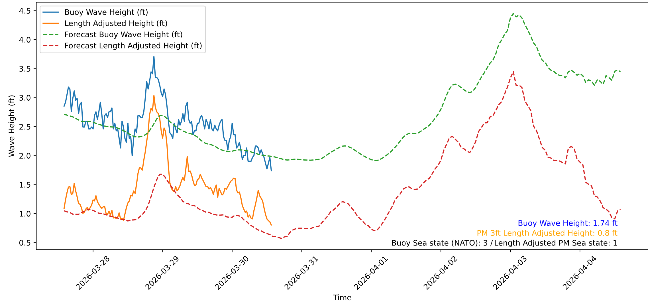
Wave Heights over Time for Green Beach at 2026-03-30 14:11:10
