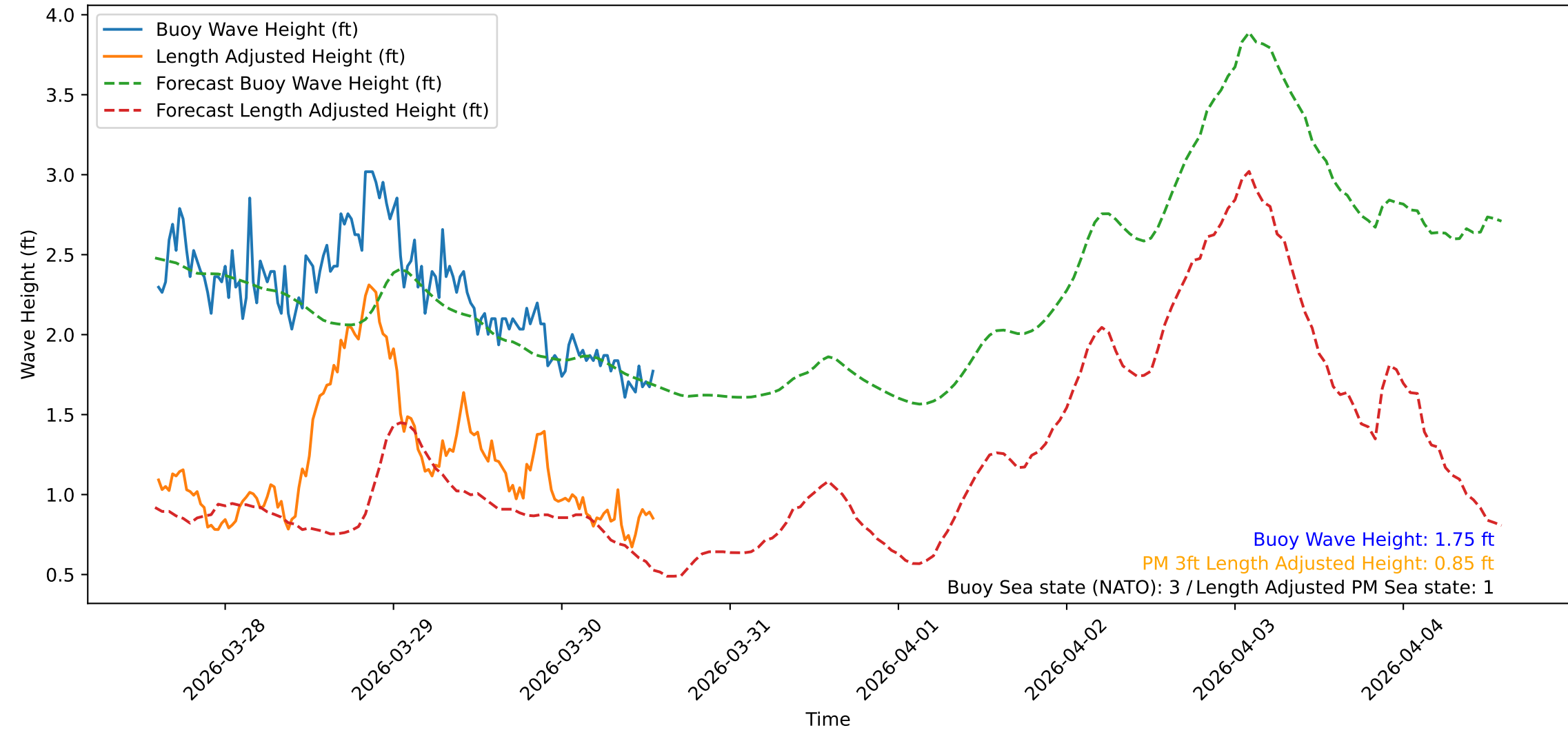
Wave Heights over Time for Red Beach at 2026-03-30 14:10:48
