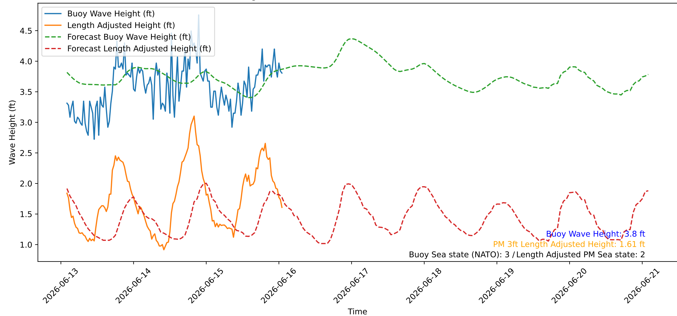
Wave Heights over Time for Red Beach at 2026-06-16 01:40:45
