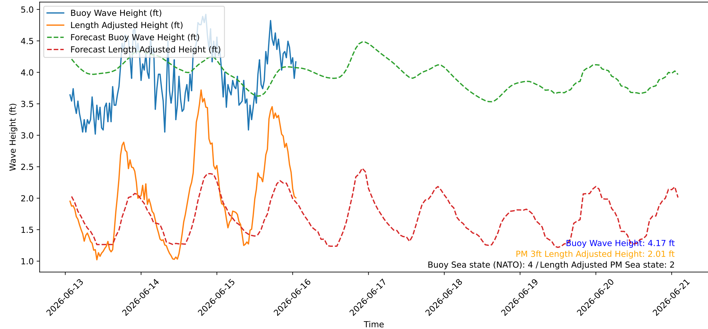
Wave Heights over Time for Green Beach at 2026-06-16 01:41:08
