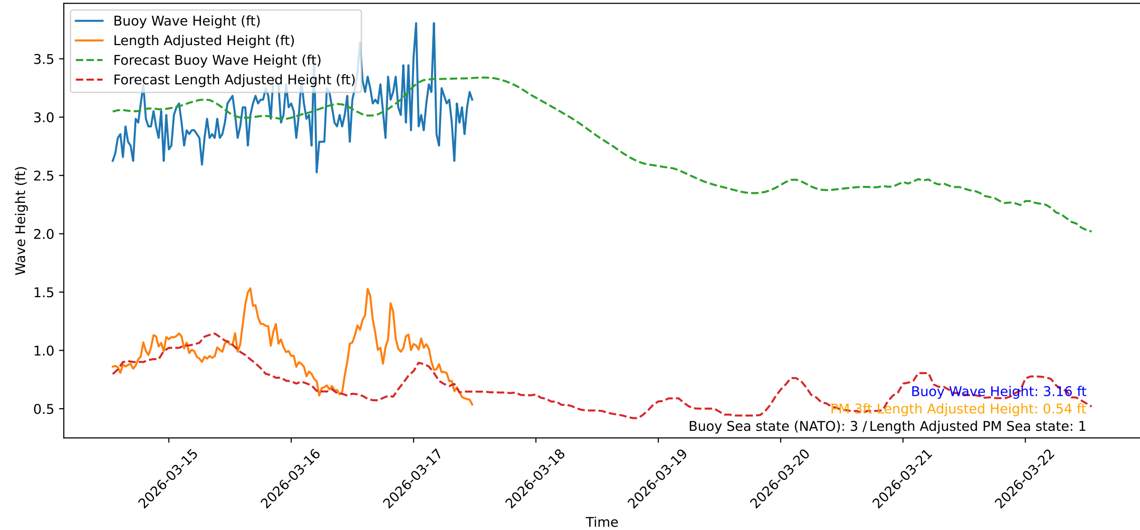
Wave Heights over Time for Red Beach at 2026-03-17 12:31:06
