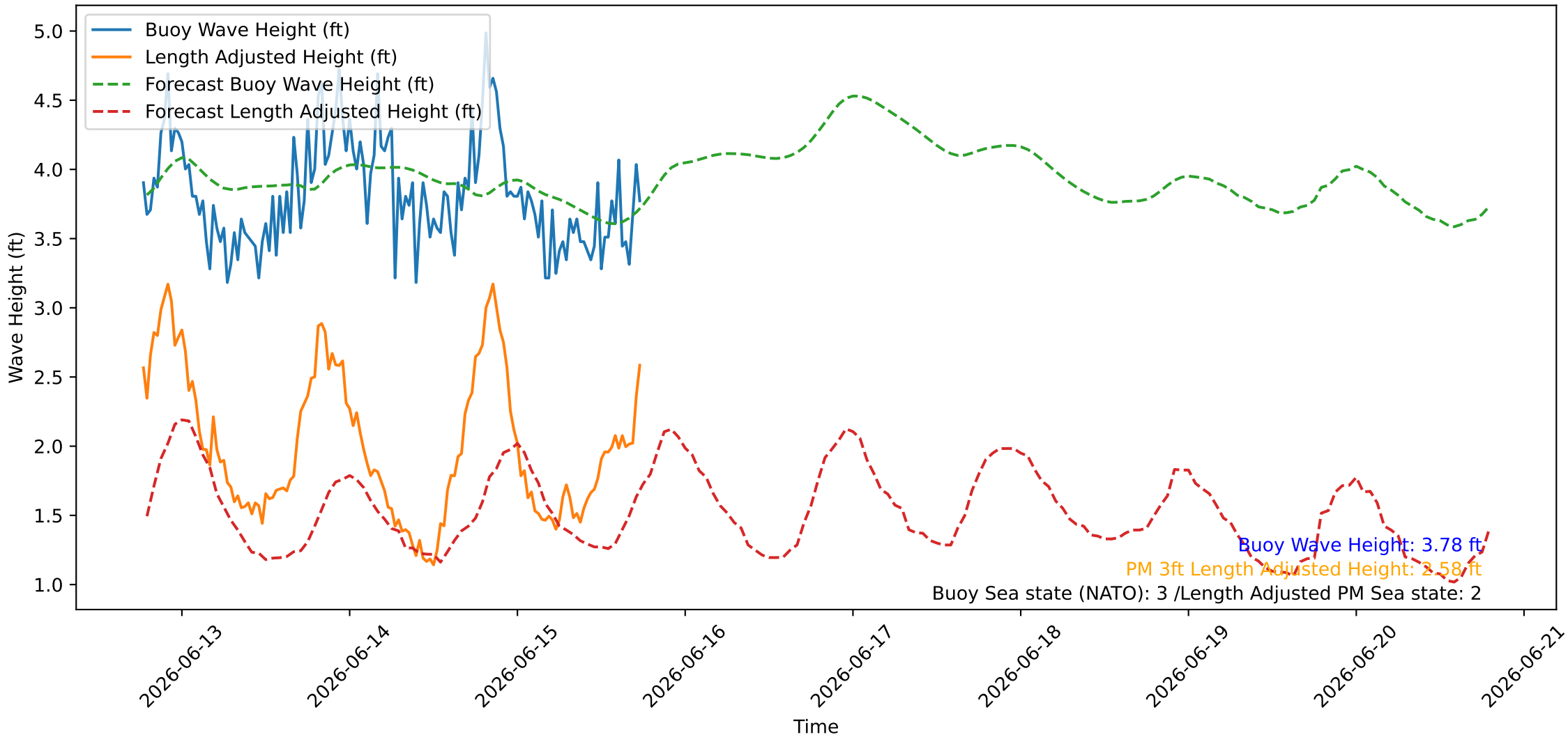
Wave Heights over Time for Oceanside Harbor at 2026-06-15 18:30:26
