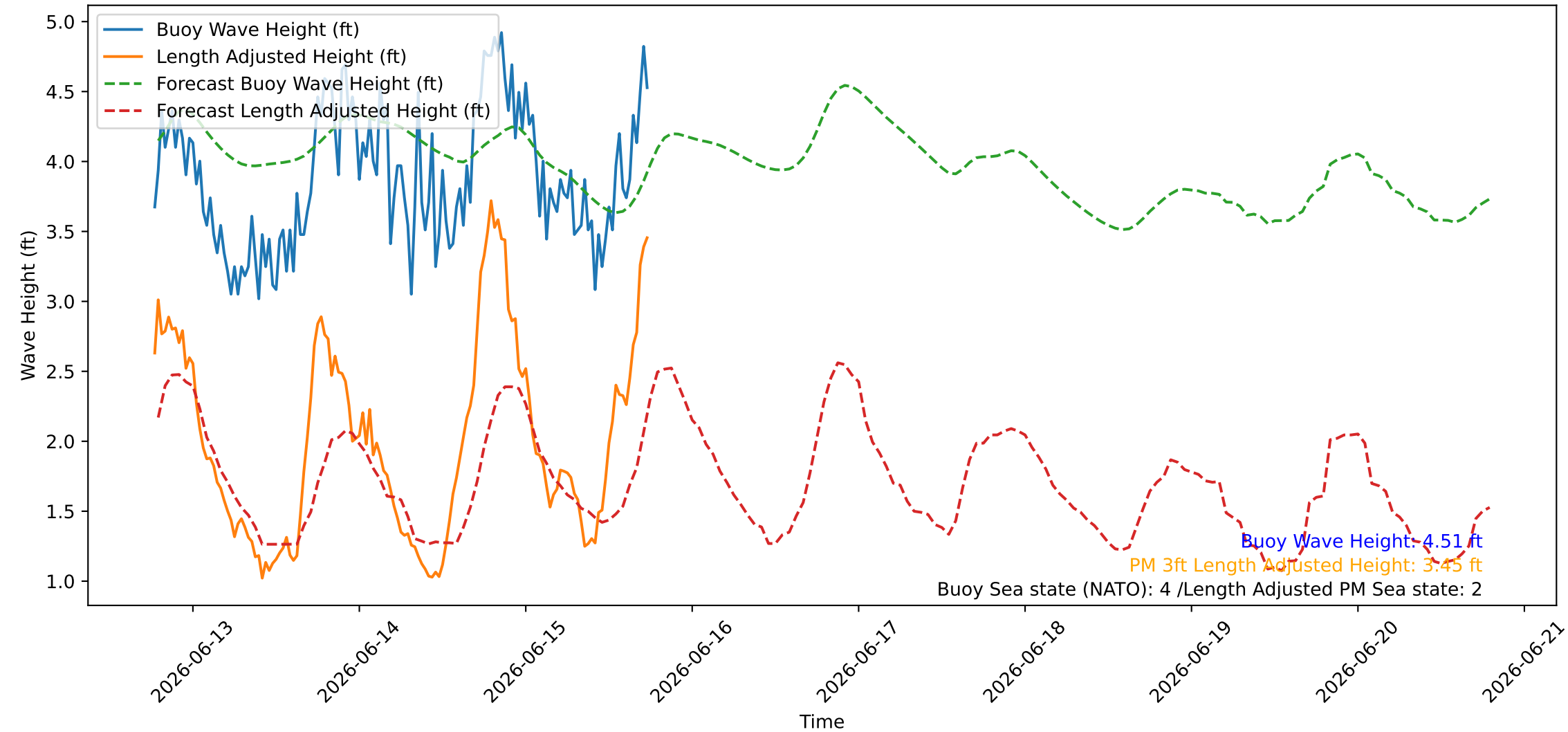
Wave Heights over Time for Green Beach at 2026-06-15 18:31:08
