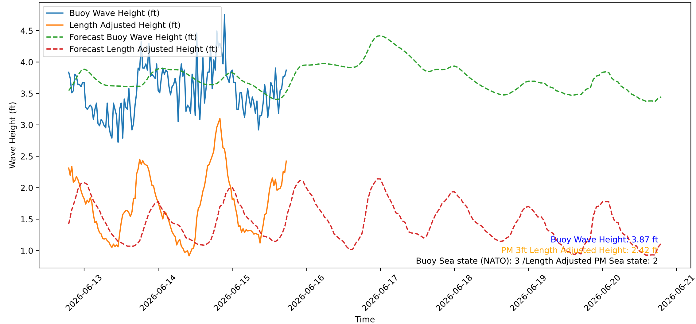
Wave Heights over Time for Red Beach at 2026-06-15 18:30:45
