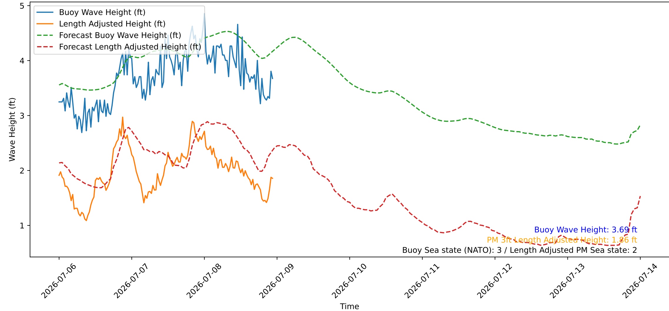
Wave Heights over Time for Red Beach at 2026-07-08 23:30:46
