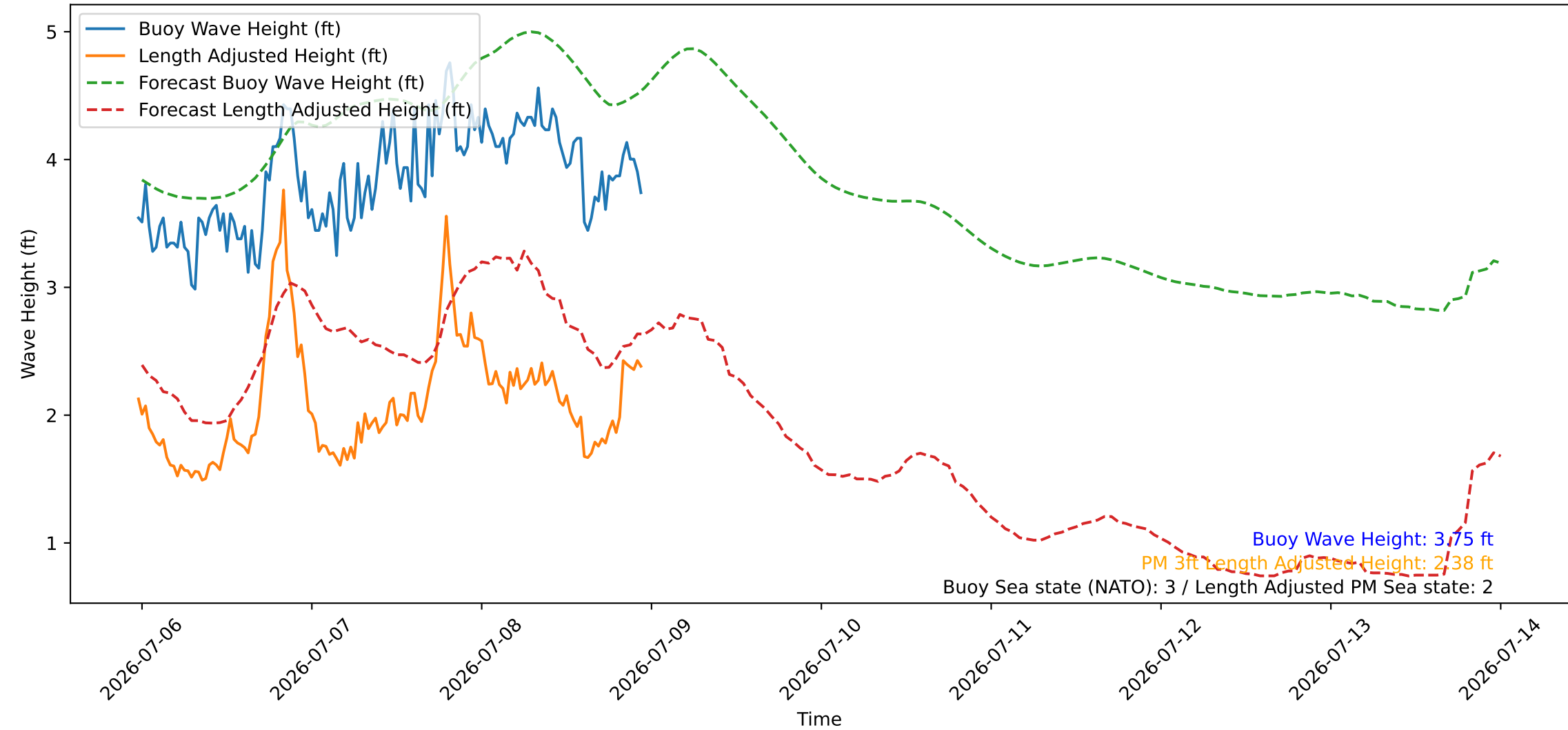
Wave Heights over Time for Green Beach at 2026-07-08 23:31:08
