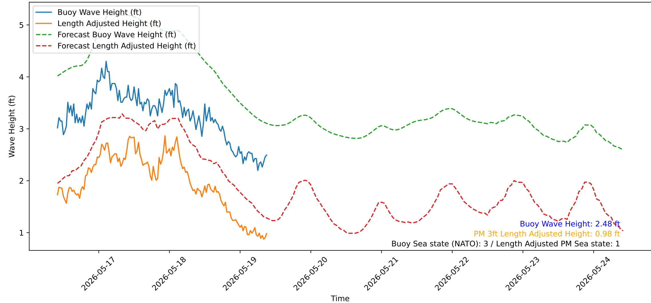
Wave Heights over Time for Oceanside Harbor at 2026-05-19 09:50:32
