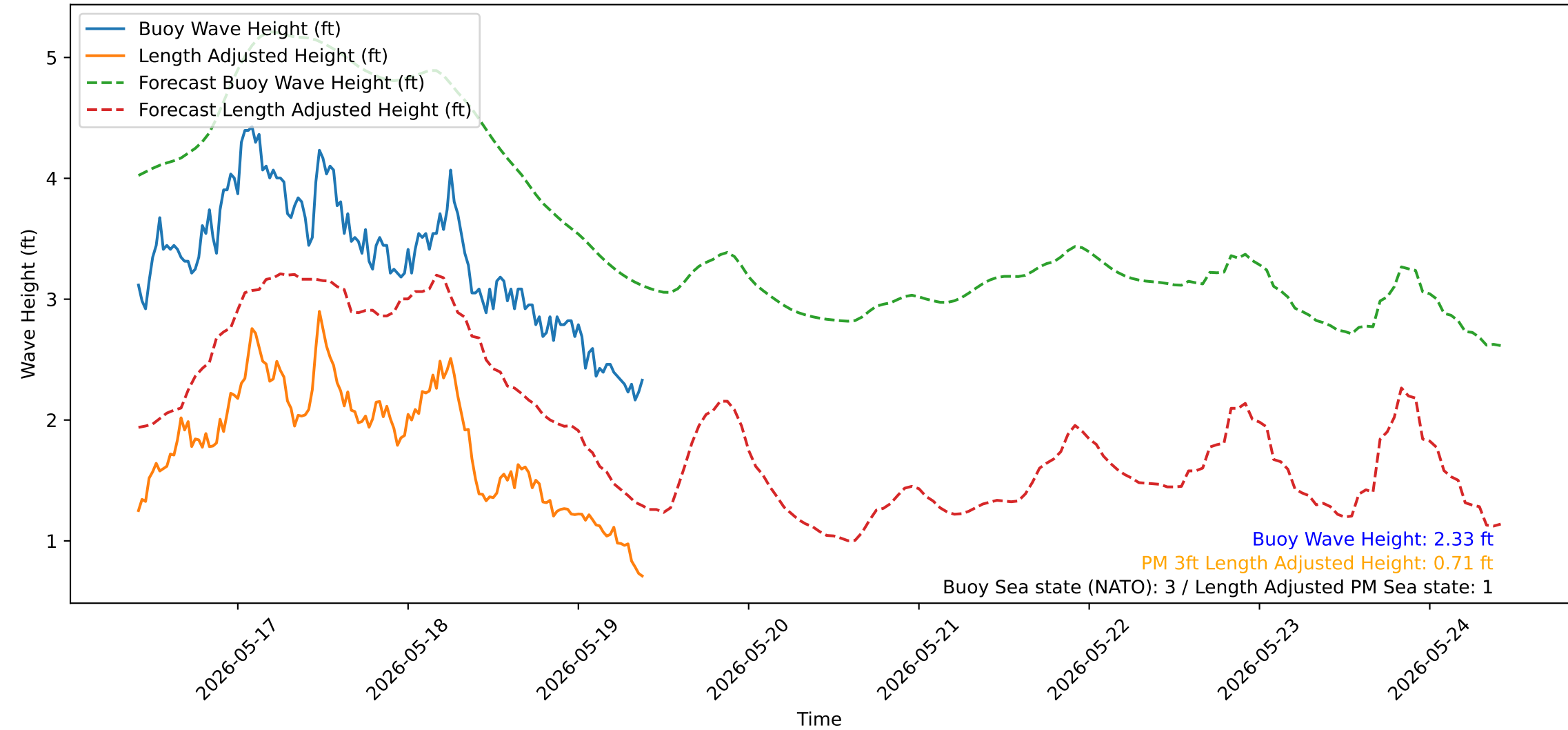
Wave Heights over Time for Green Beach at 2026-05-19 09:51:16
