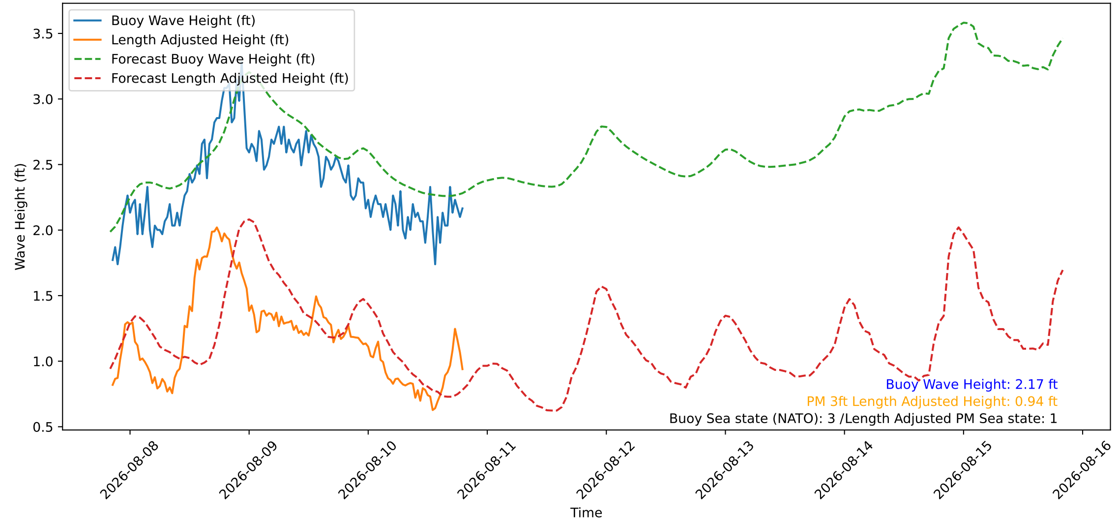
Wave Heights over Time for Red Beach at 2026-08-10 20:10:46
