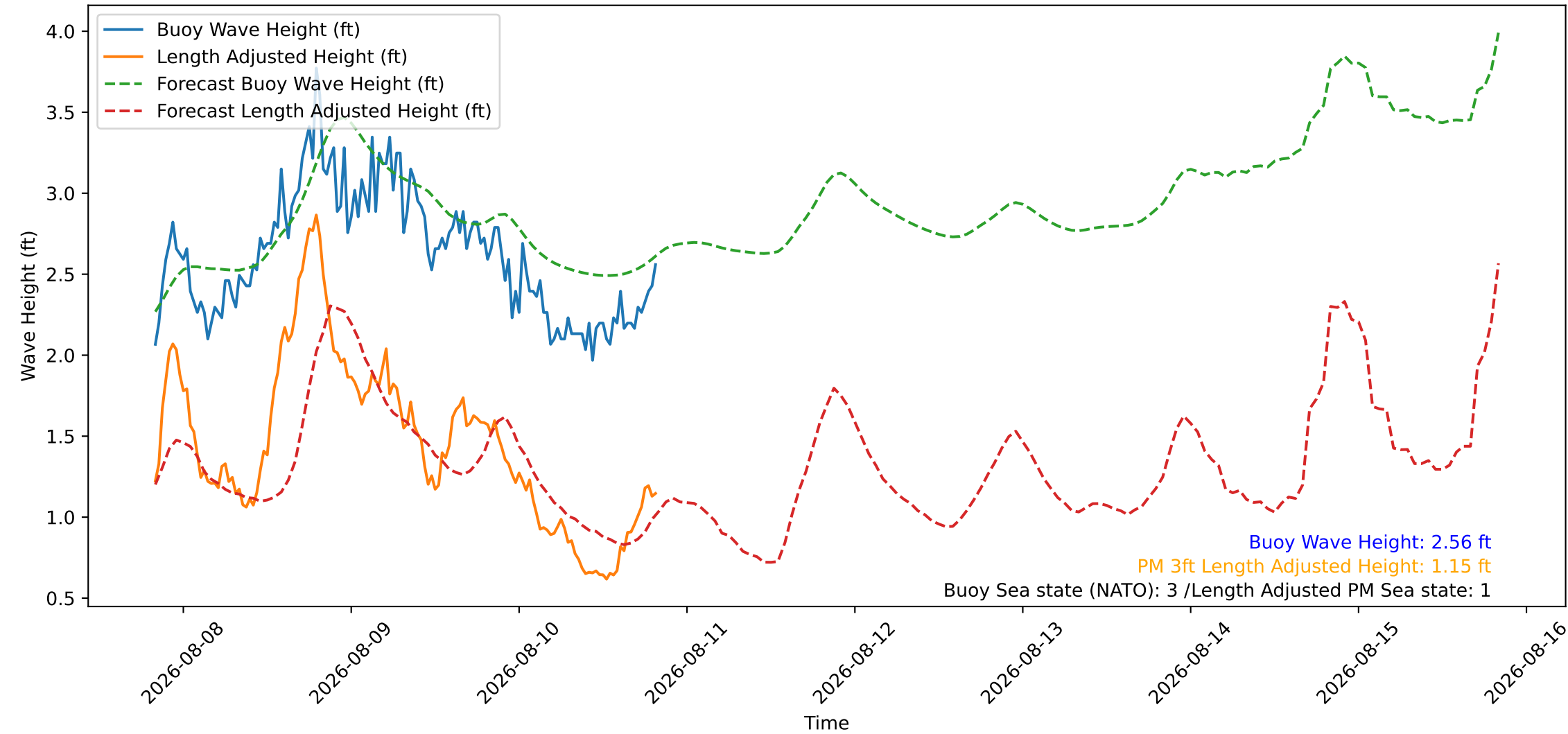
Wave Heights over Time for Green Beach at 2026-08-10 20:11:10
