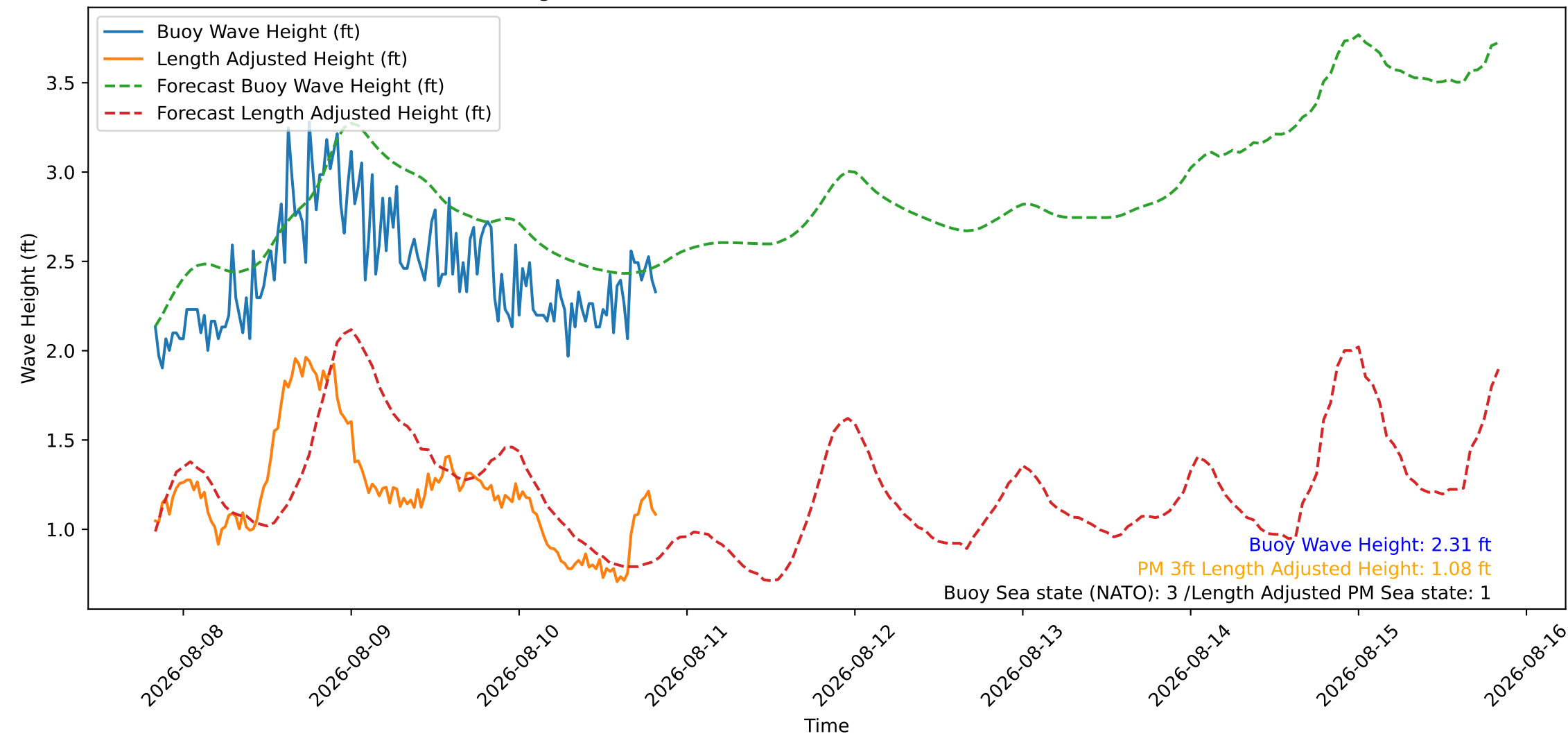
Wave Heights over Time for Oceanside Harbor at 2026-08-10 20:10:27
