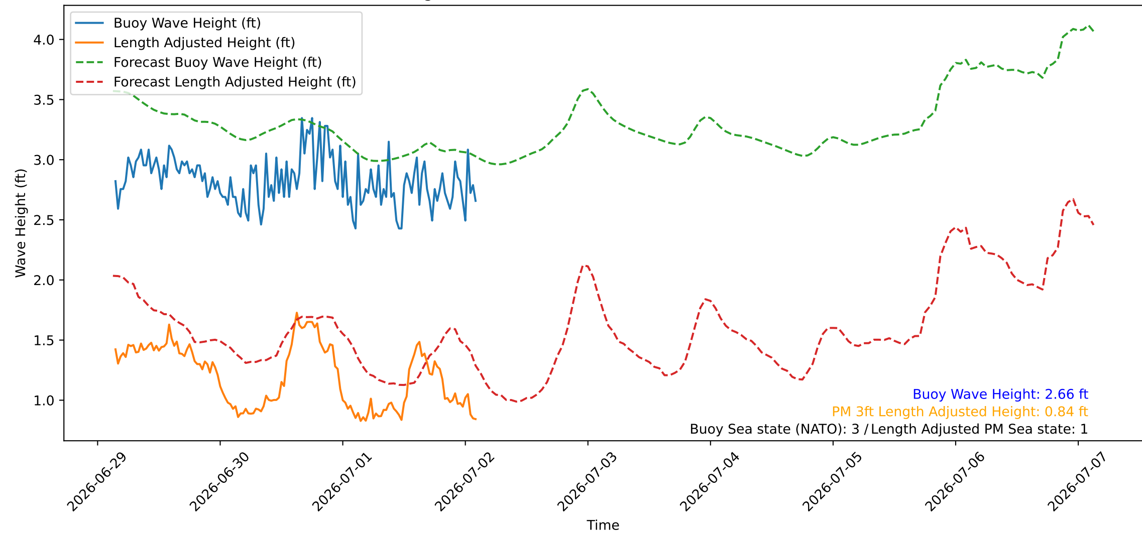
Wave Heights over Time for Red Beach at 2026-07-02 03:00:45
