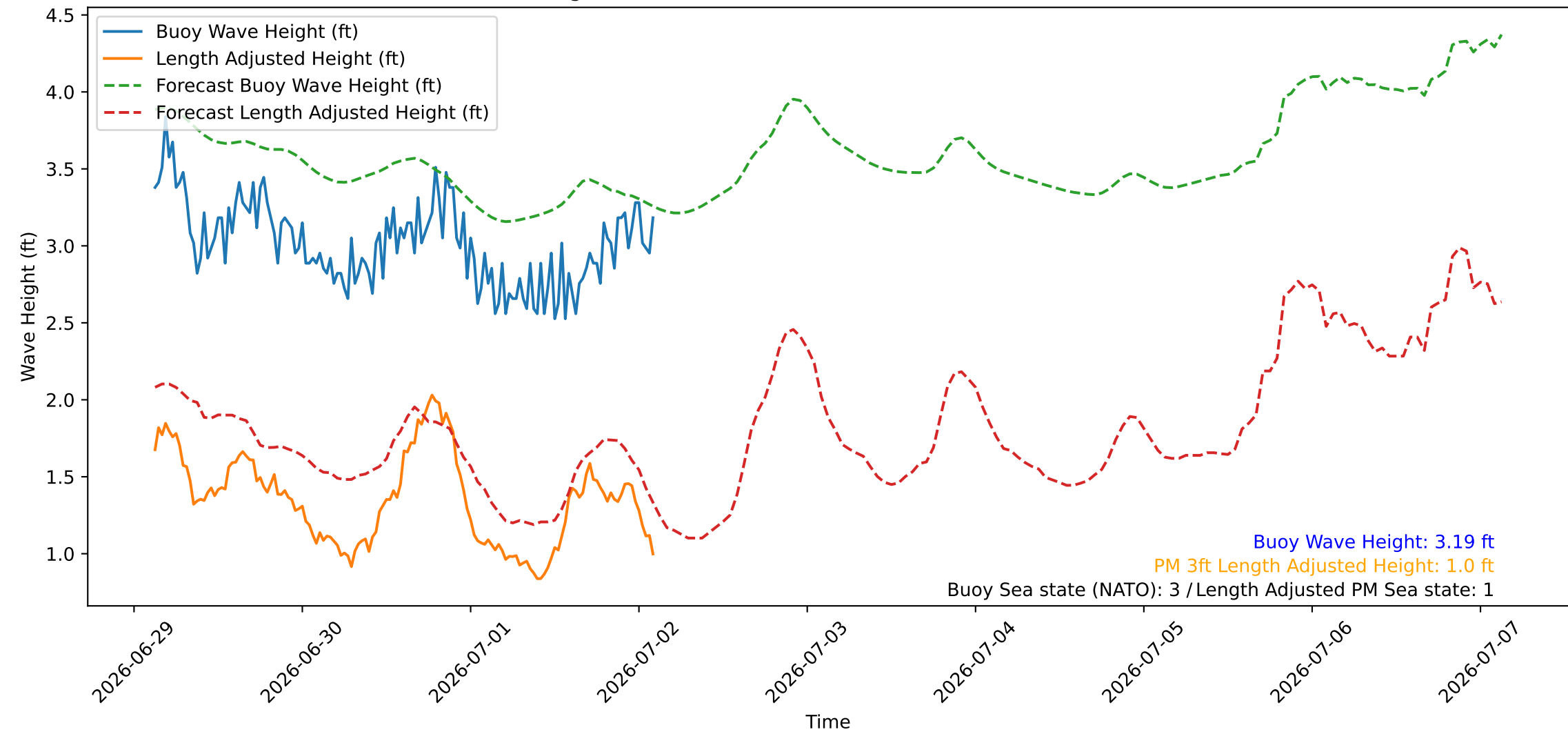
Wave Heights over Time for Green Beach at 2026-07-02 03:01:07
