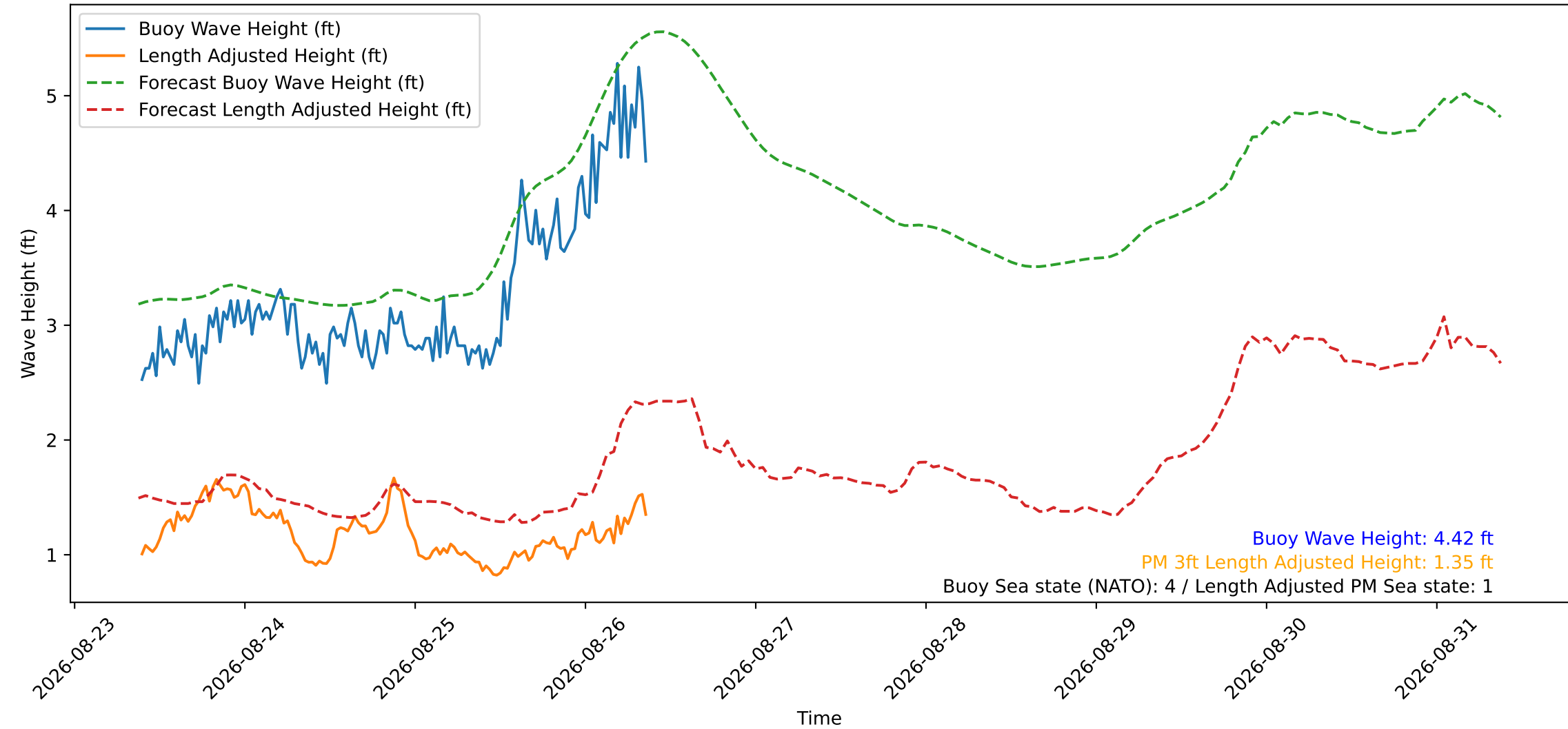
Wave Heights over Time for Green Beach at 2026-08-26 09:21:20
