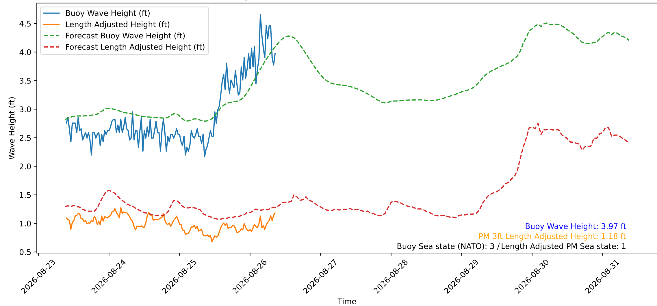
Wave Heights over Time for Red Beach at 2026-08-26 09:20:54
