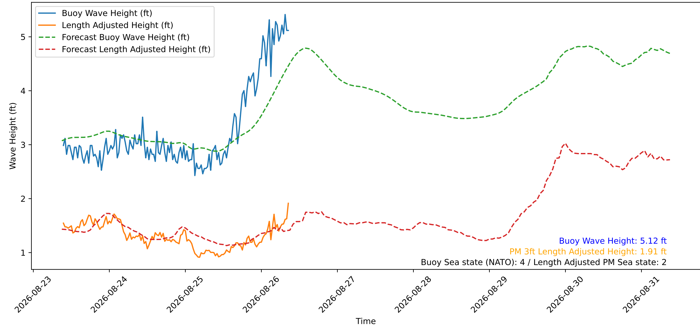
Wave Heights over Time for Oceanside Harbor at 2026-08-26 09:20:31
