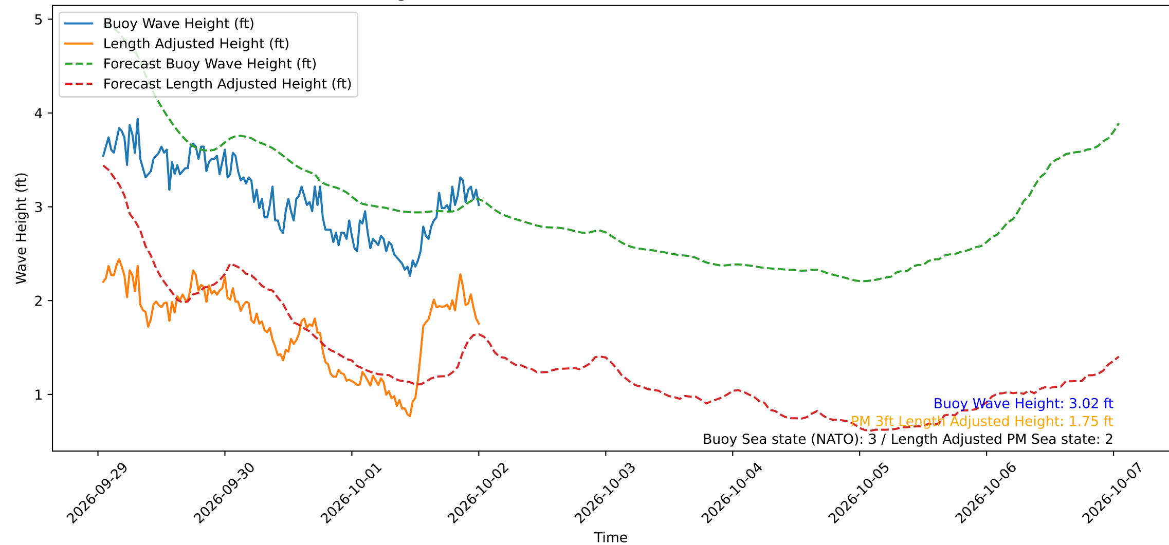
Wave Heights over Time for Oceanside Harbor at 2026-10-02 01:00:29
