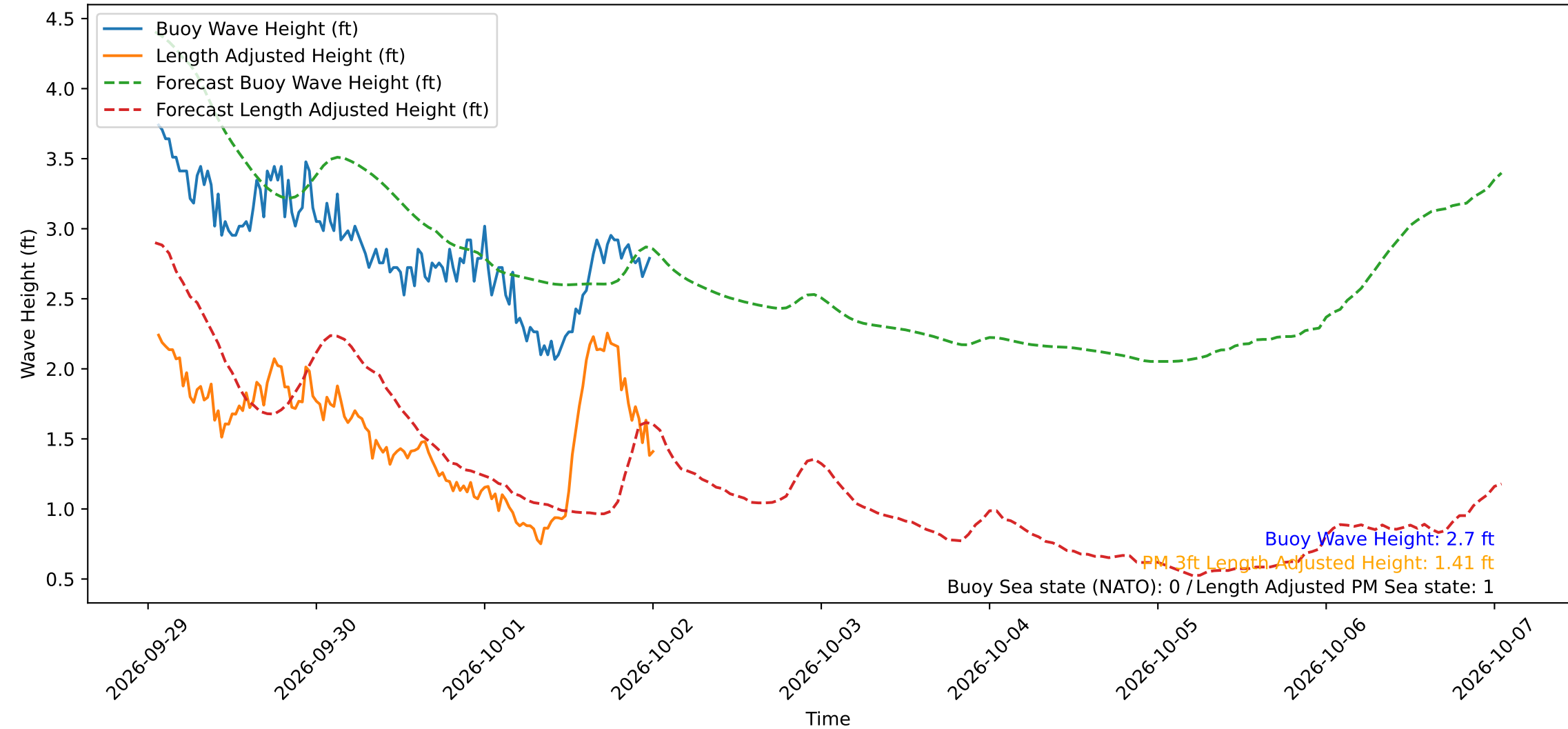
Wave Heights over Time for Red Beach at 2026-10-02 01:00:49
