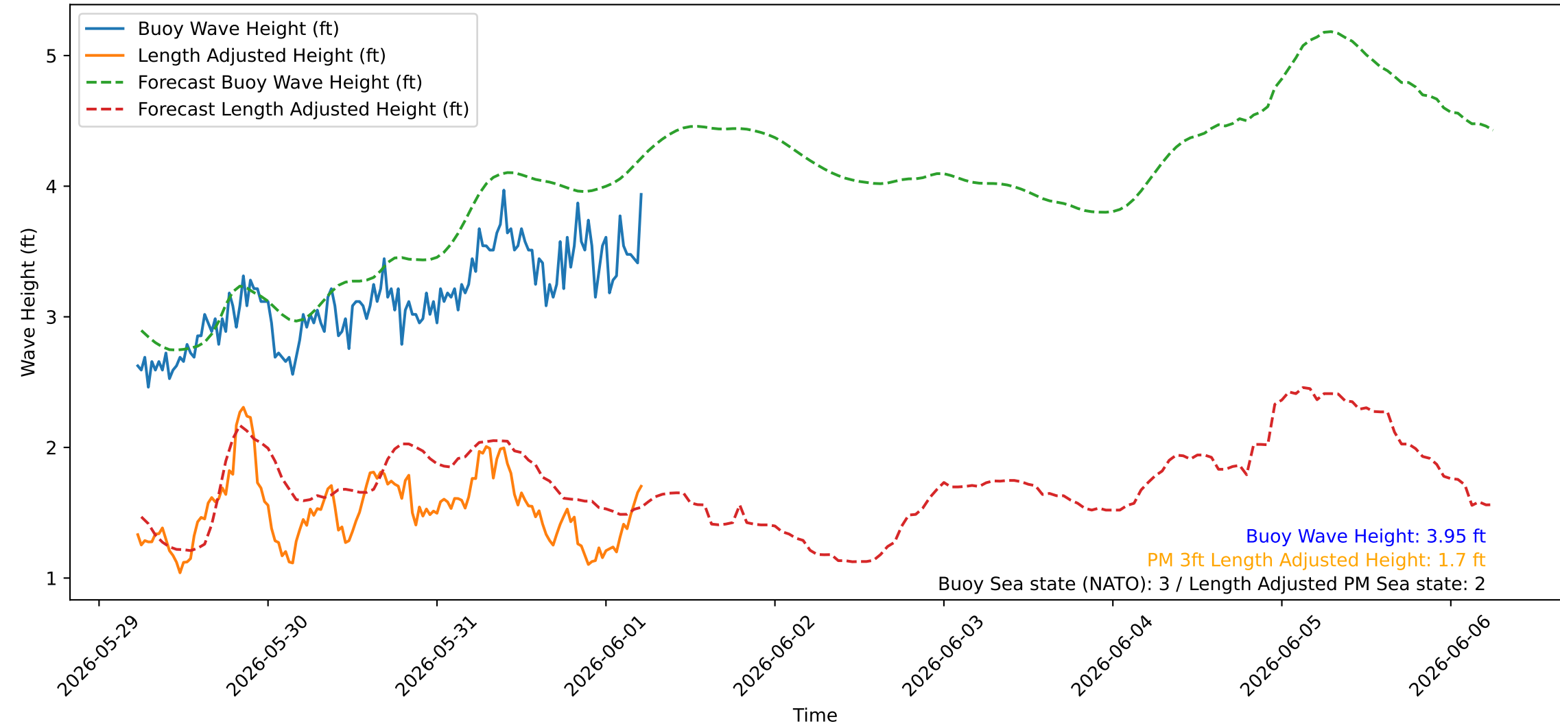
Wave Heights over Time for Green Beach at 2026-06-01 05:41:08
