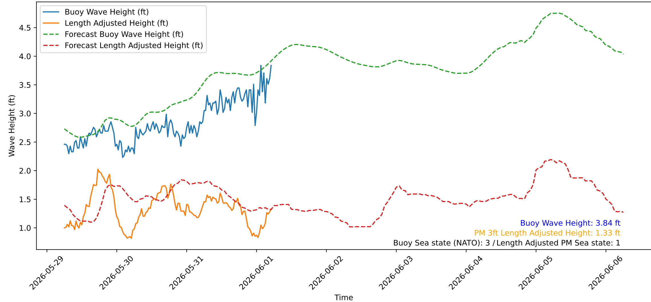
Wave Heights over Time for Red Beach at 2026-06-01 05:40:45
