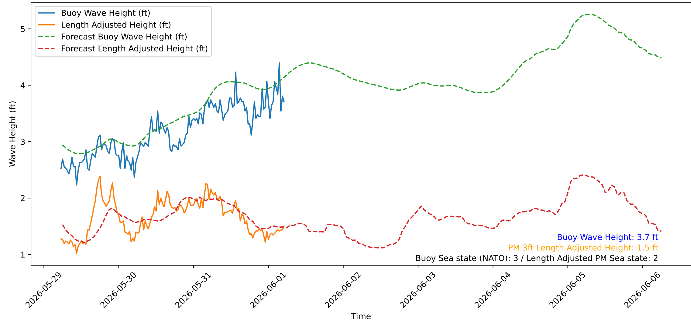
Wave Heights over Time for Oceanside Harbor at 2026-06-01 05:40:26
