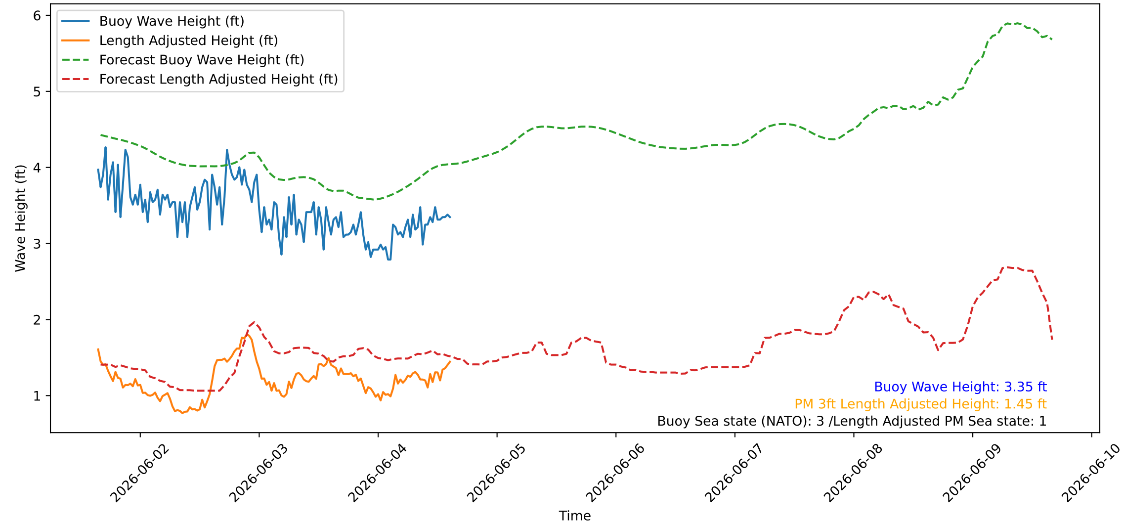
Wave Heights over Time for Green Beach at 2026-06-04 15:31:07
