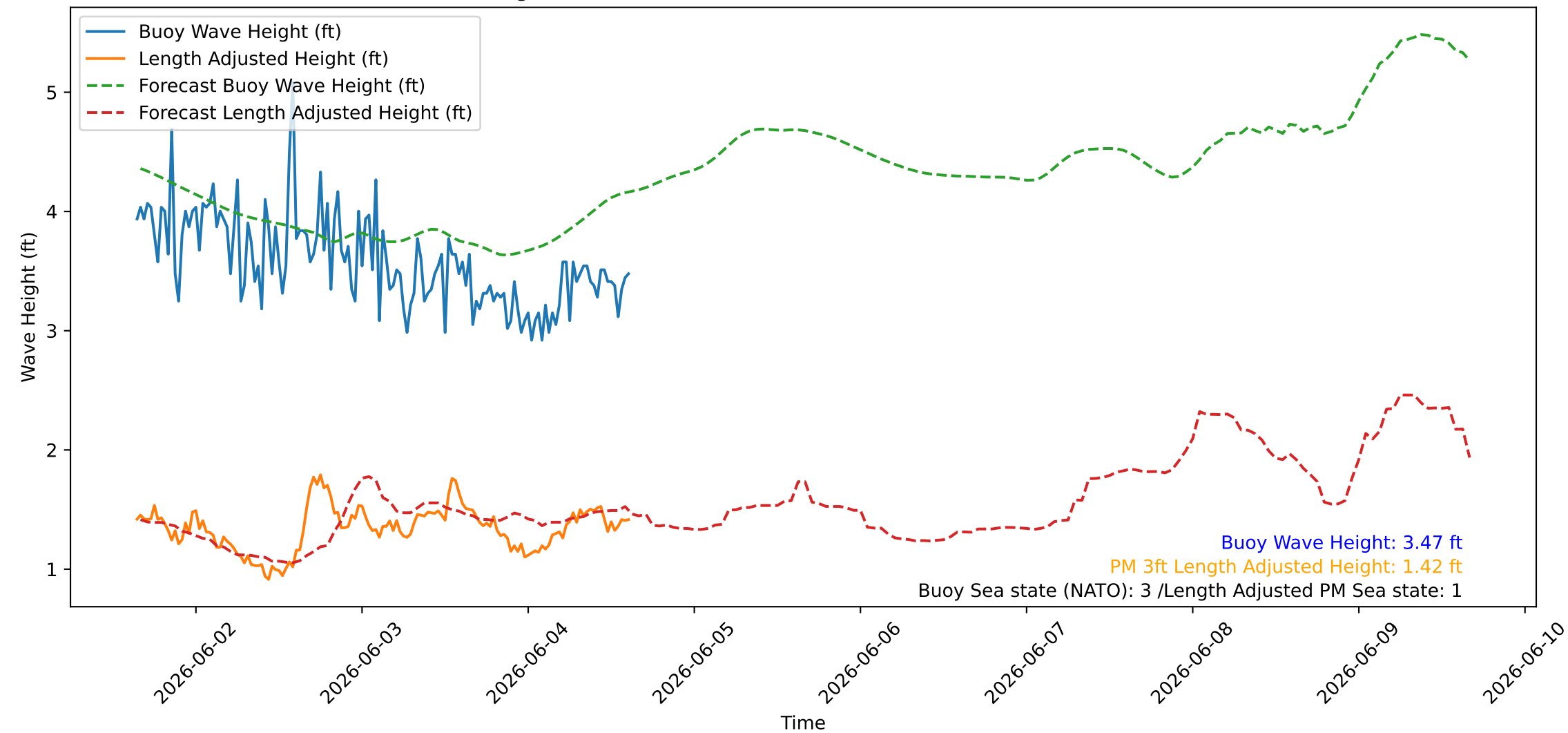
Wave Heights over Time for Oceanside Harbor at 2026-06-04 15:30:26
