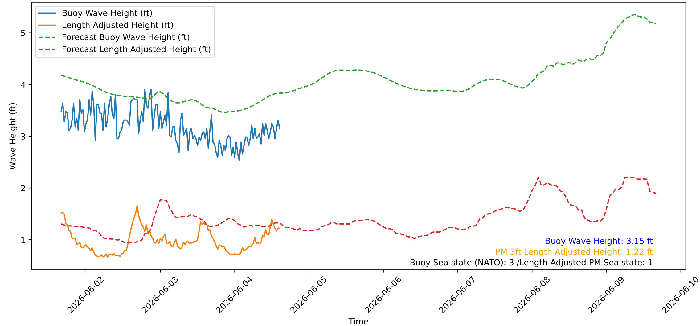
Wave Heights over Time for Red Beach at 2026-06-04 15:30:45
