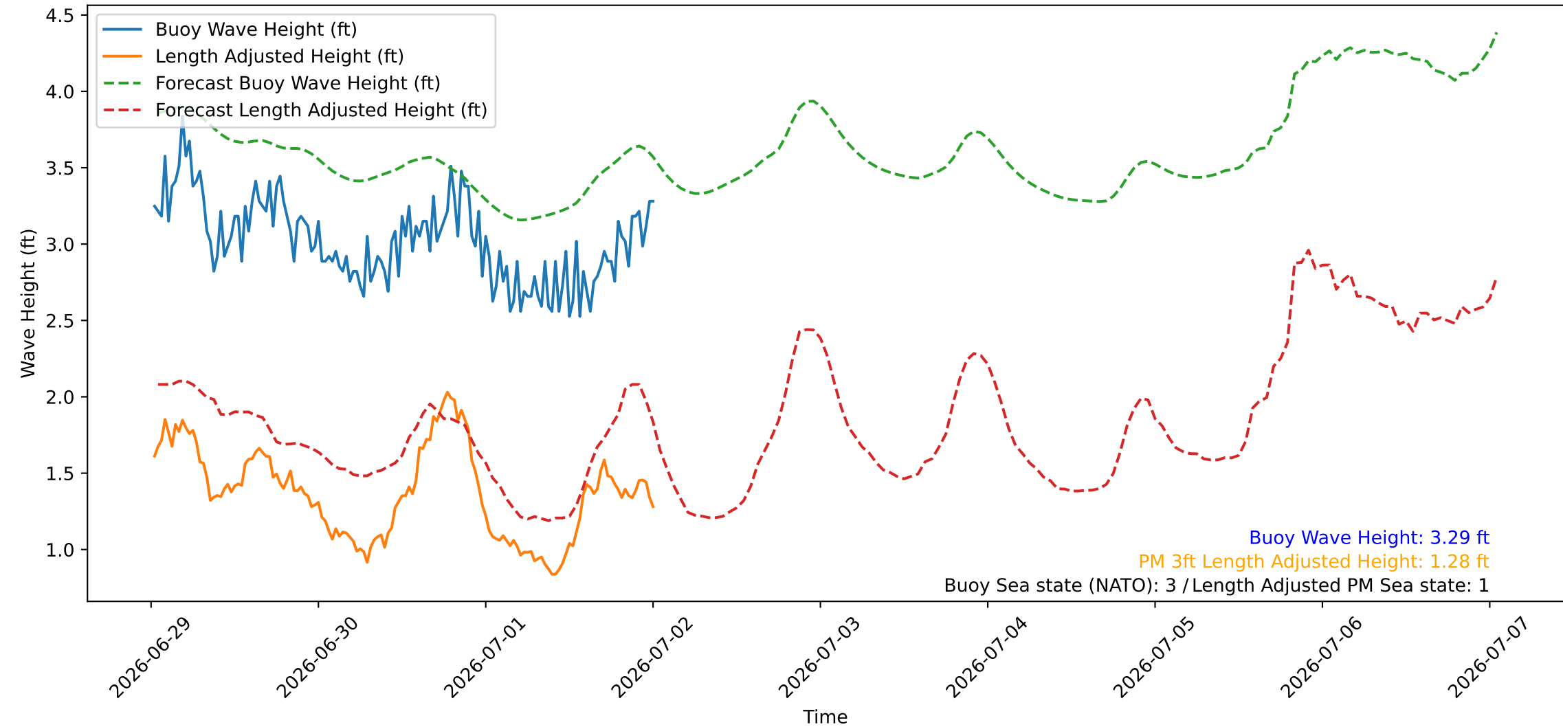
Wave Heights over Time for Green Beach at 2026-07-02 00:41:08
