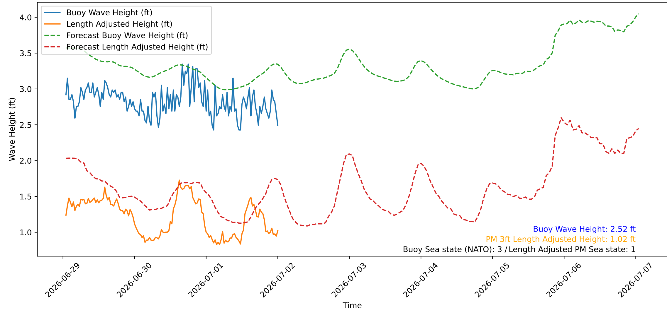
Wave Heights over Time for Red Beach at 2026-07-02 00:40:46
