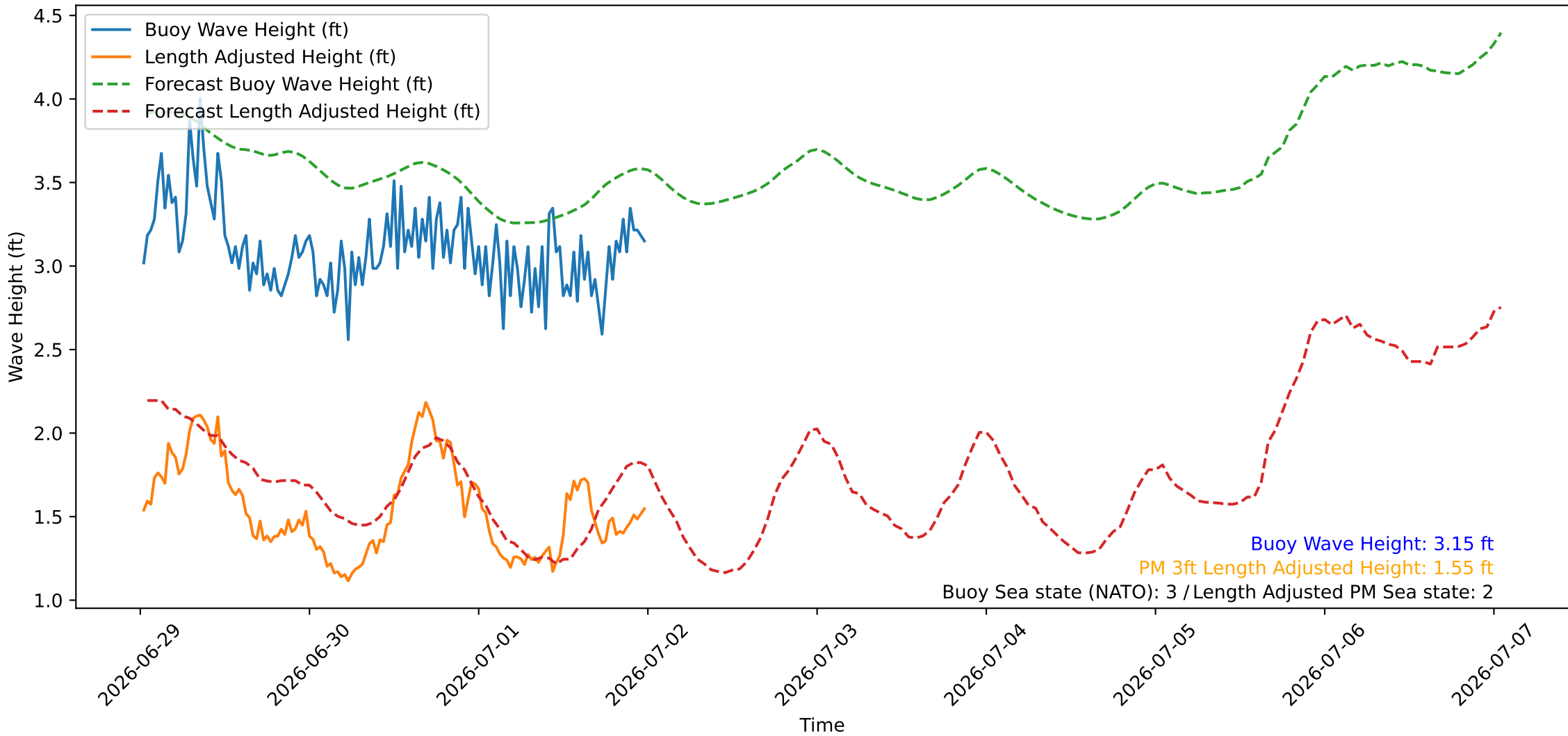
Wave Heights over Time for Oceanside Harbor at 2026-07-02 00:40:26
