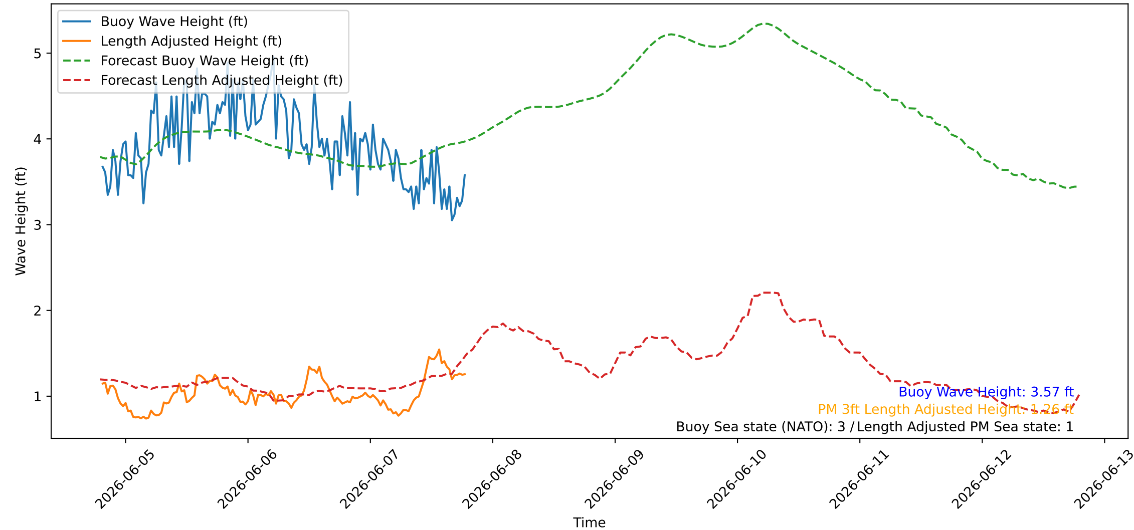
Wave Heights over Time for Red Beach at 2026-06-07 19:20:47
