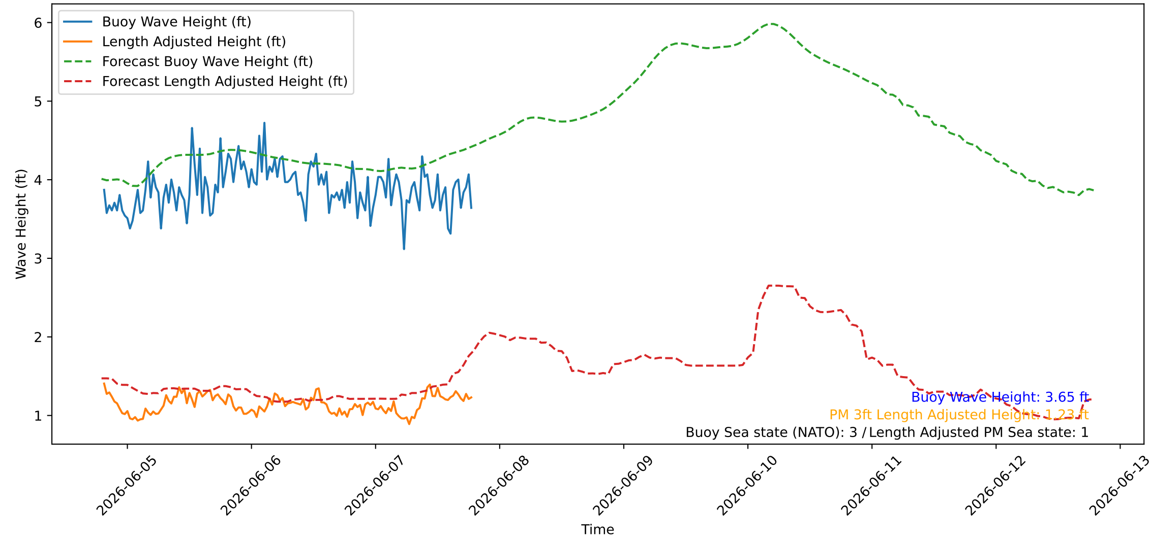
Wave Heights over Time for Green Beach at 2026-06-07 19:21:09
