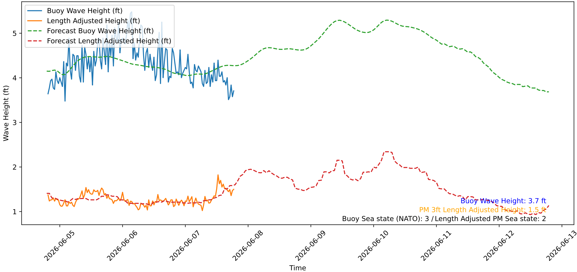
Wave Heights over Time for Oceanside Harbor at 2026-06-07 19:20:26
