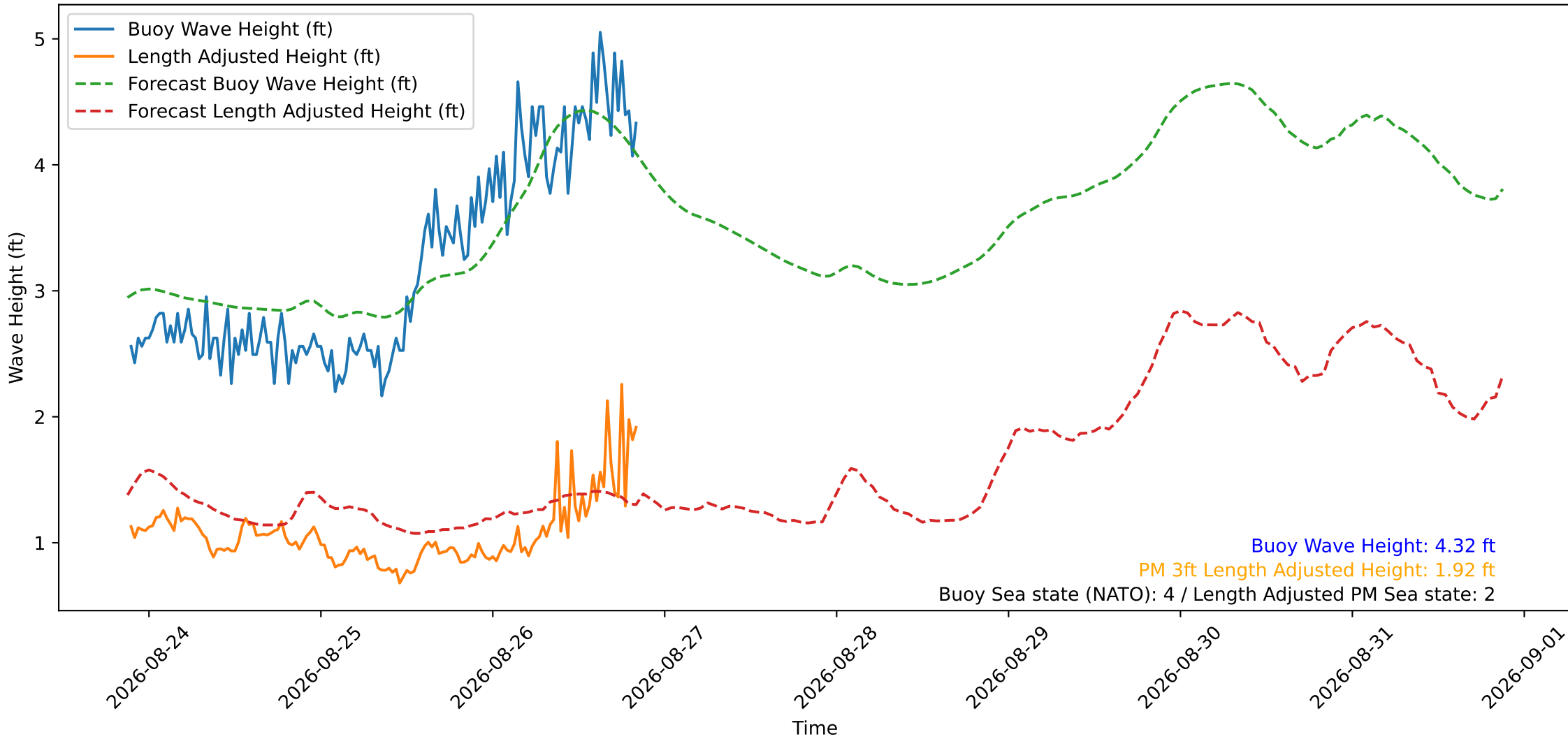
Wave Heights over Time for Red Beach at 2026-08-26 21:00:49
