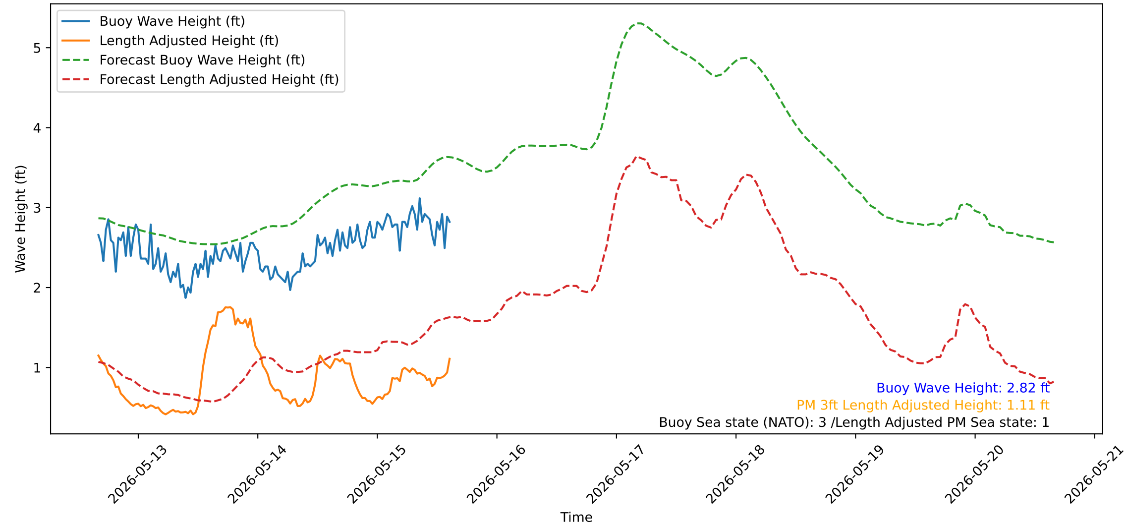
Wave Heights over Time for Red Beach at 2026-05-15 15:30:51
