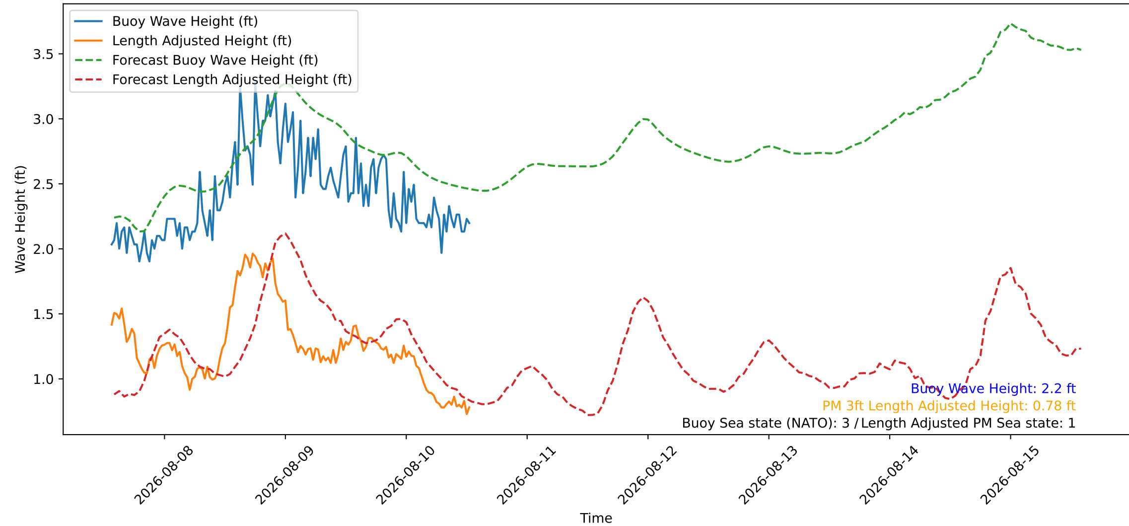
Wave Heights over Time for Oceanside Harbor at 2026-08-10 13:30:27
