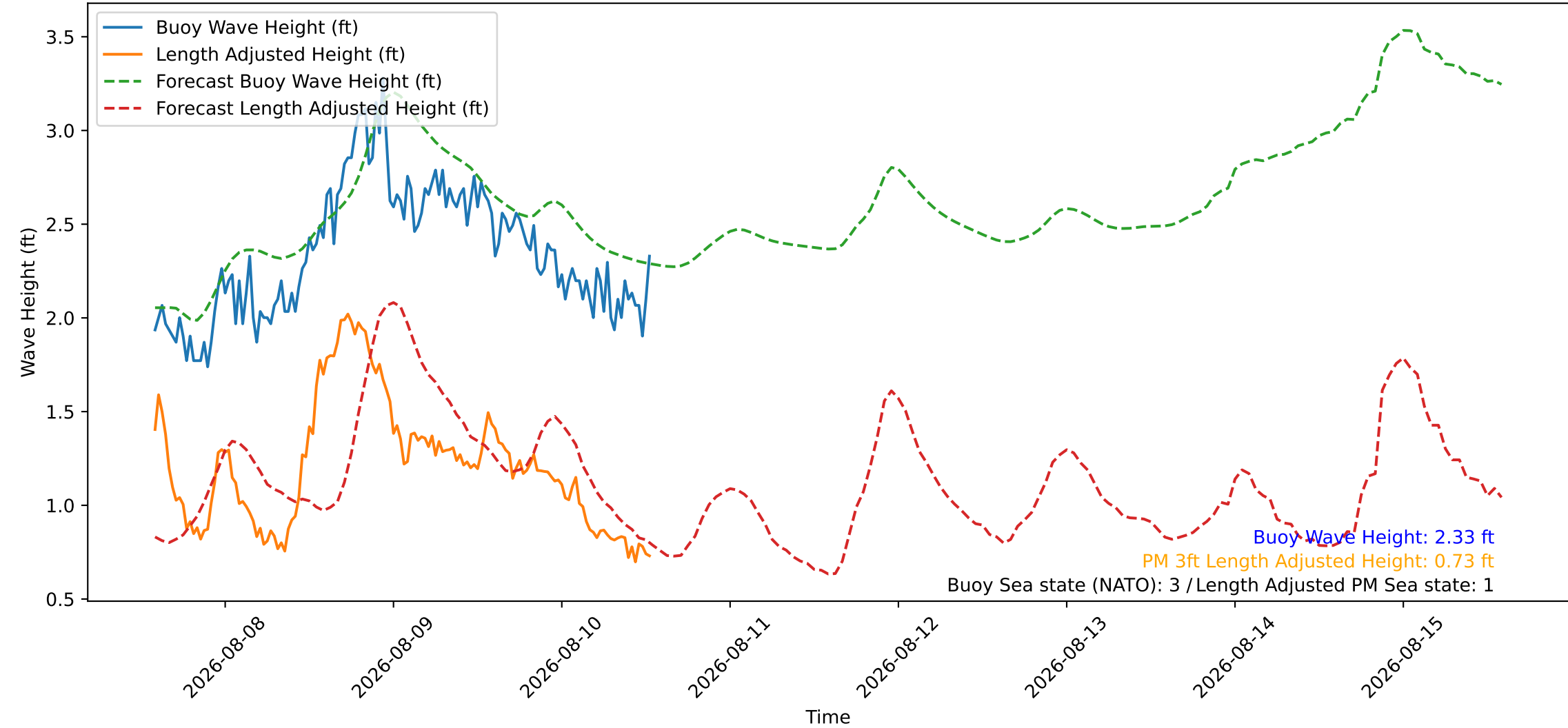
Wave Heights over Time for Red Beach at 2026-08-10 13:30:47
