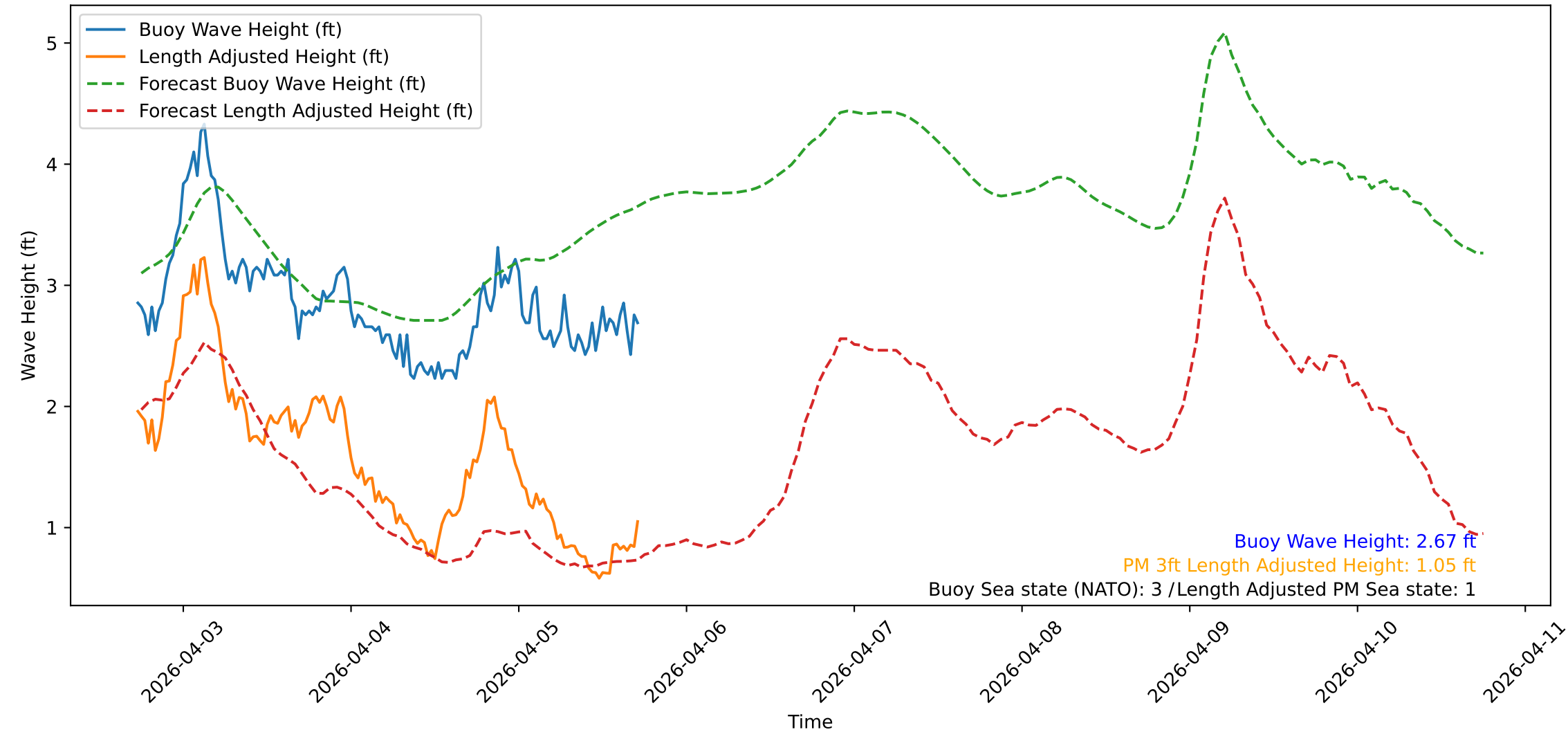
Wave Heights over Time for Green Beach at 2026-04-05 17:41:12
