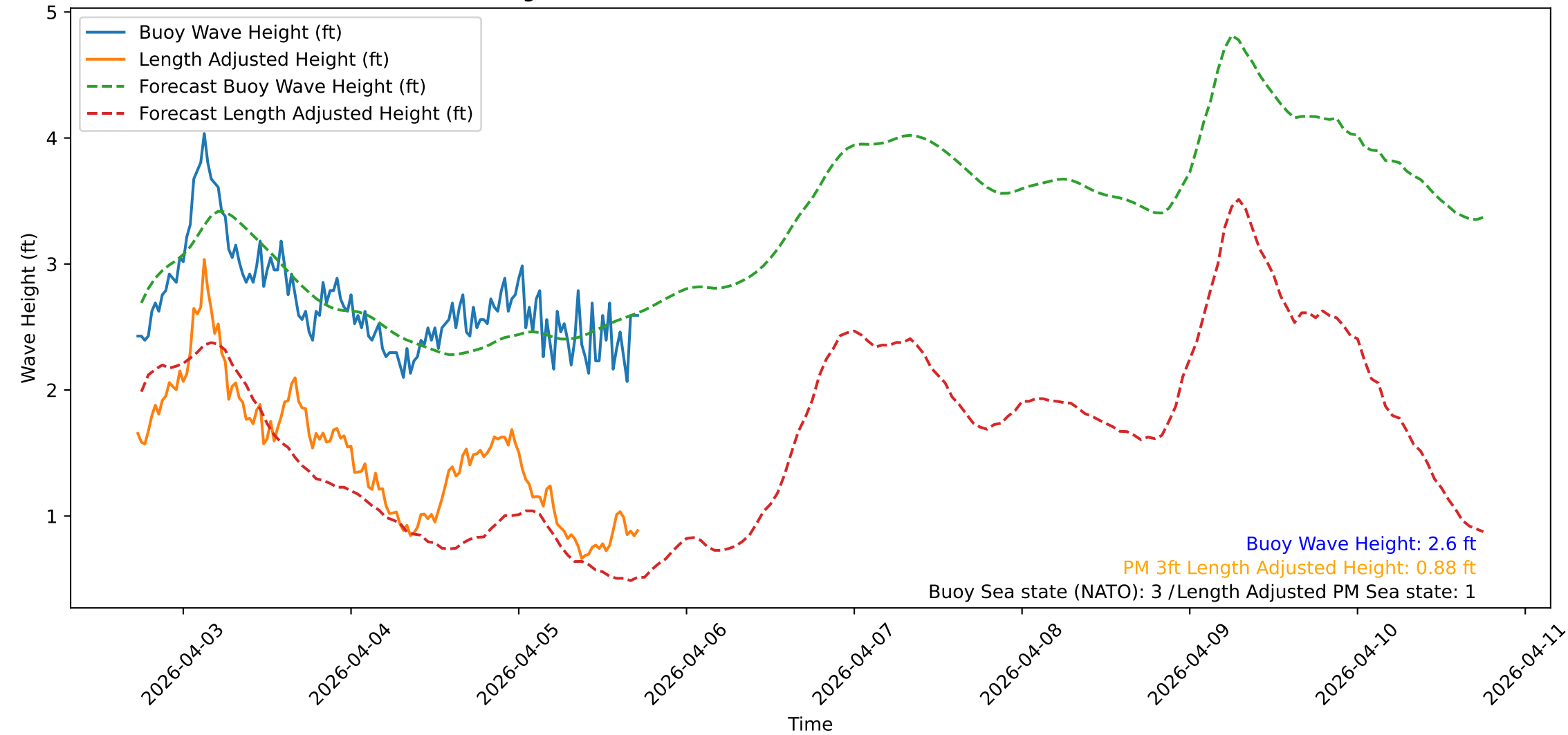
Wave Heights over Time for Oceanside Harbor at 2026-04-05 17:40:32
