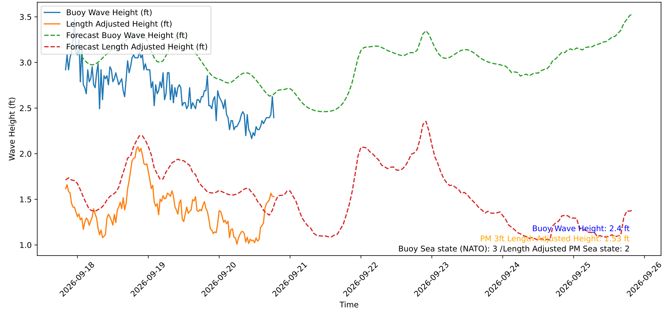
Wave Heights over Time for Green Beach at 2026-09-20 19:31:14
