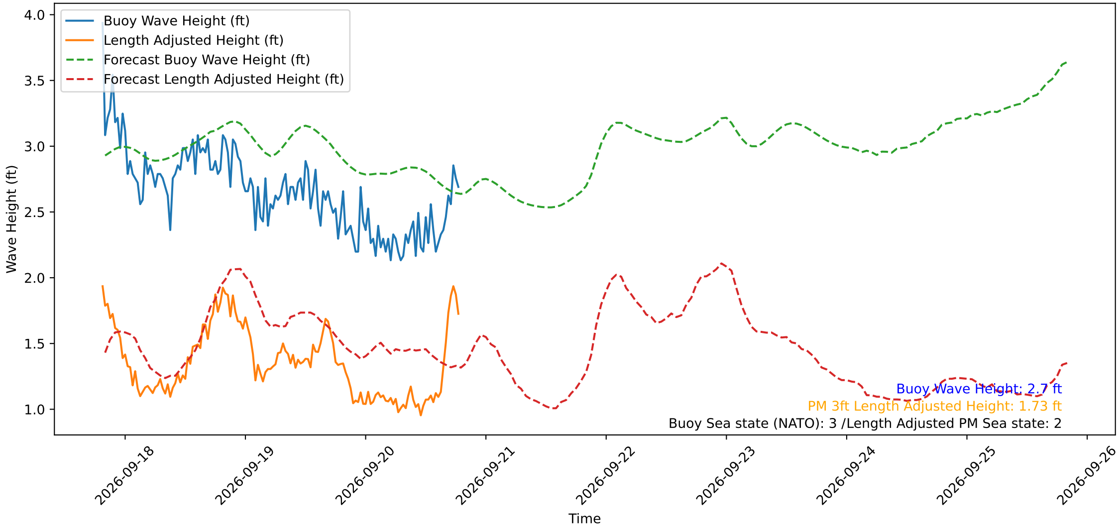
Wave Heights over Time for Oceanside Harbor at 2026-09-20 19:30:30
