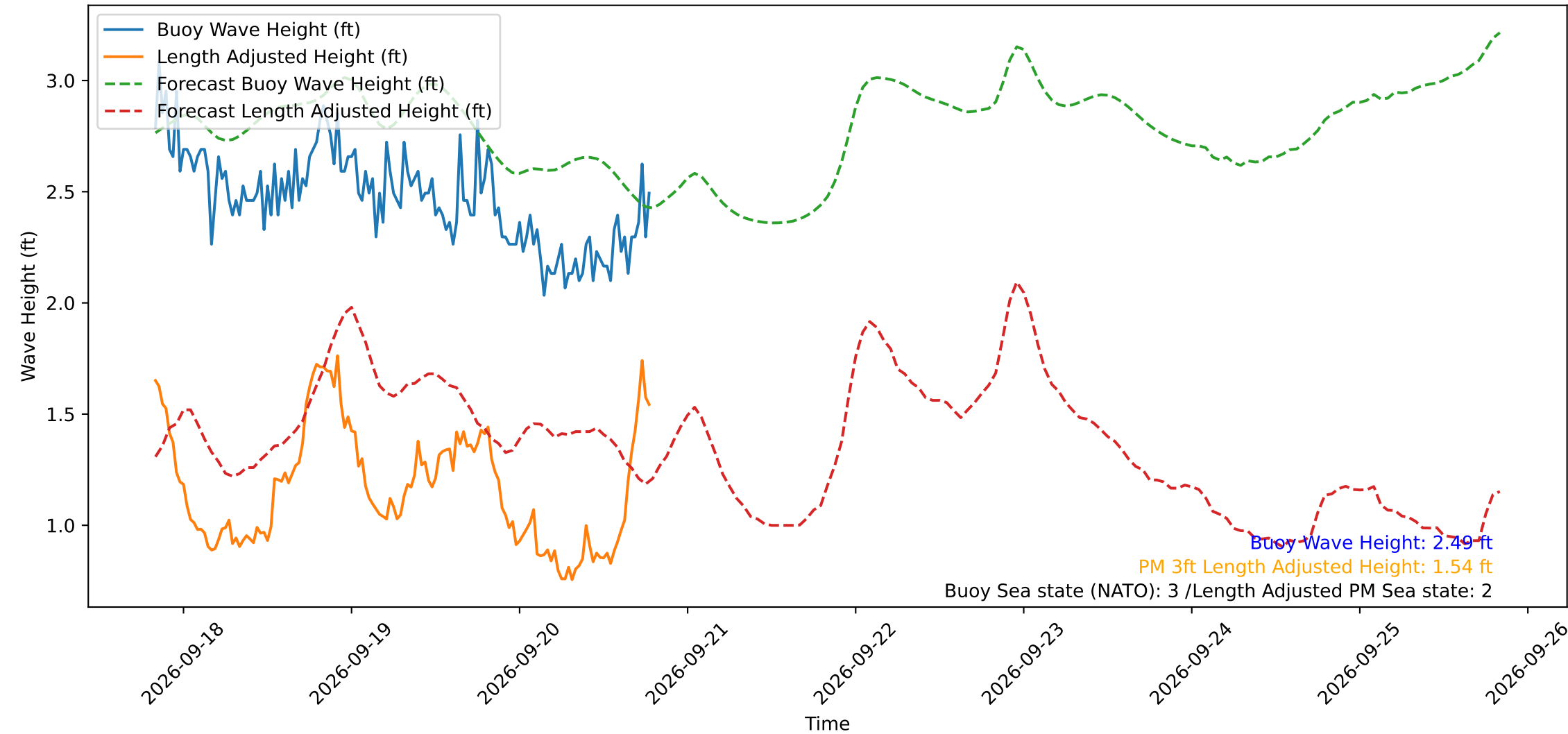
Wave Heights over Time for Red Beach at 2026-09-20 19:30:49
