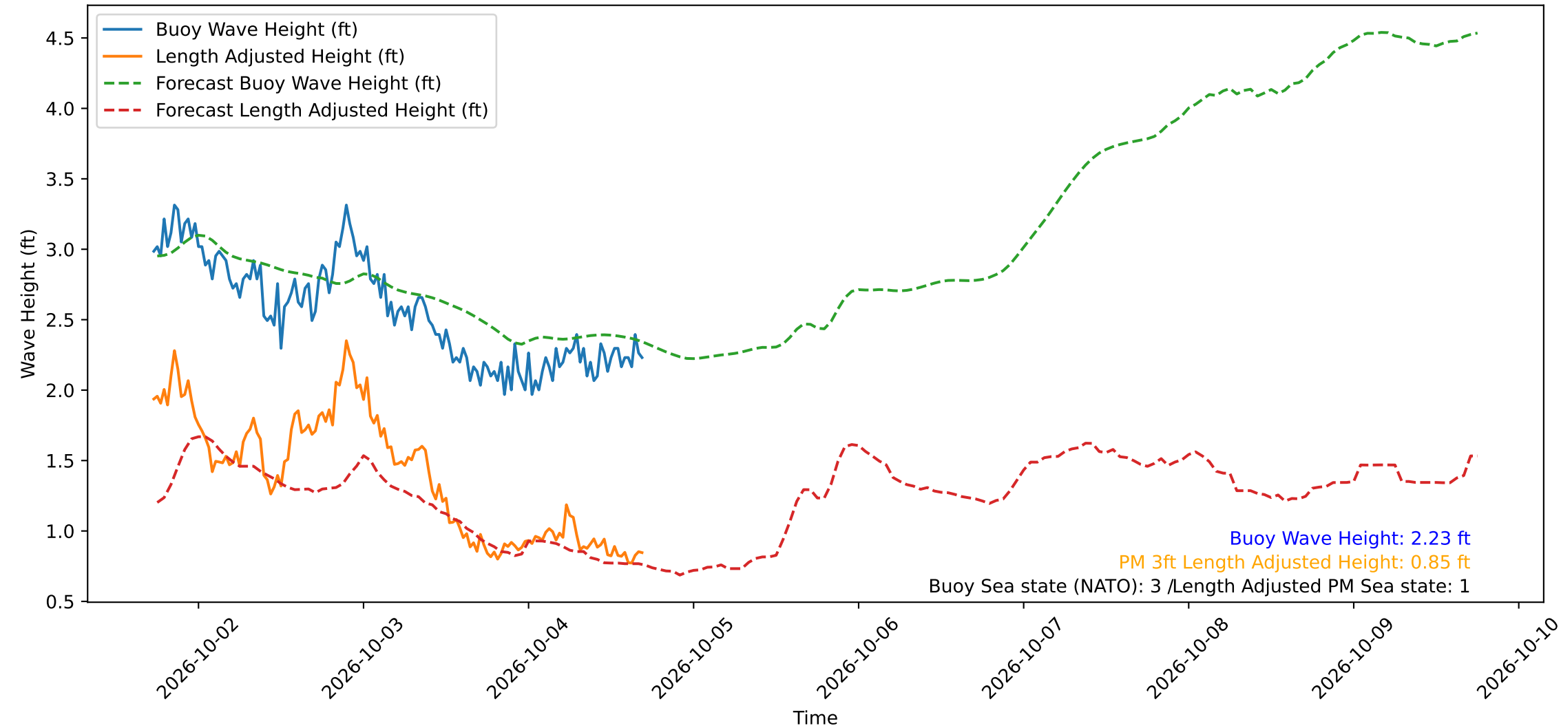
Wave Heights over Time for Oceanside Harbor at 2026-10-04 17:40:30
