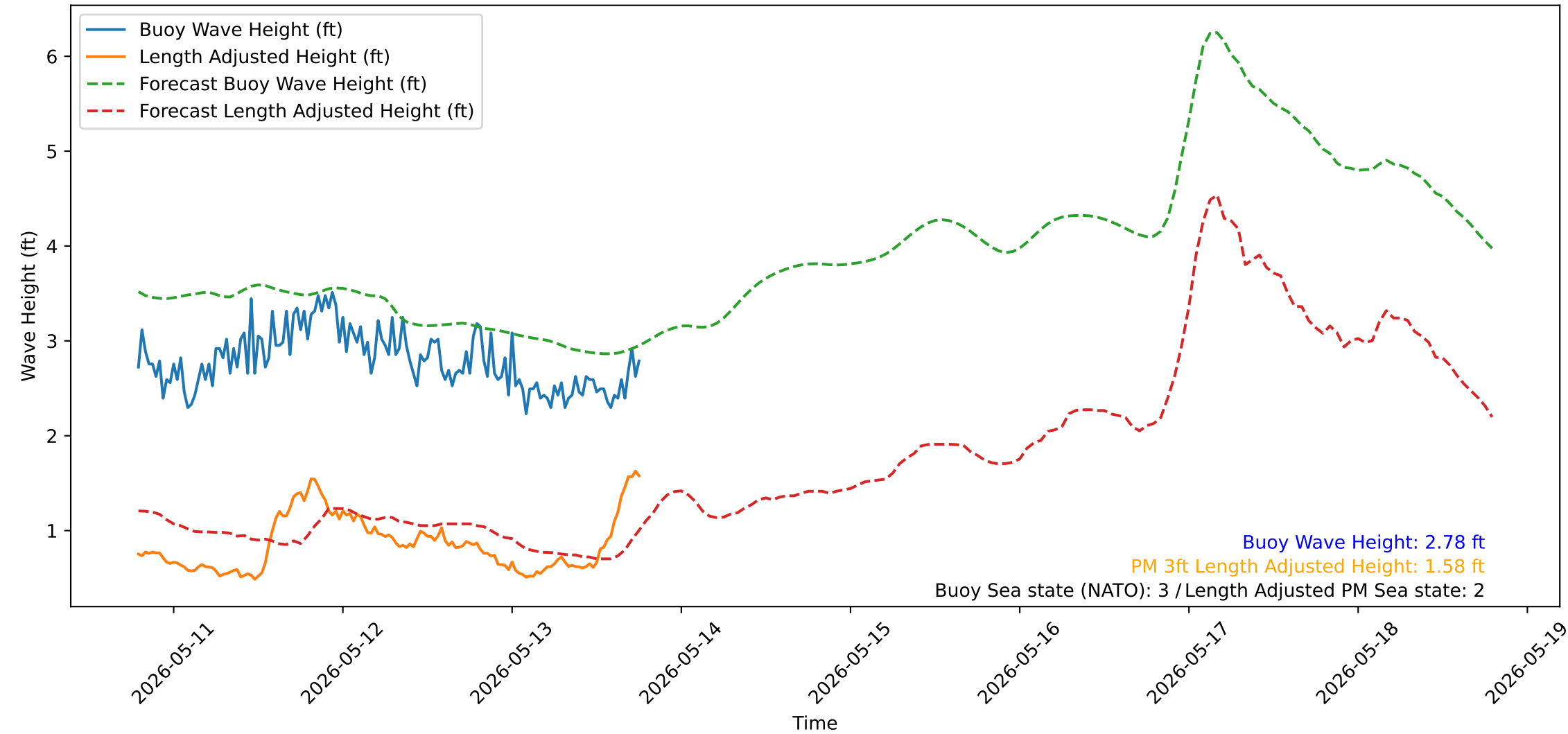
Wave Heights over Time for Green Beach at 2026-05-13 18:51:15
