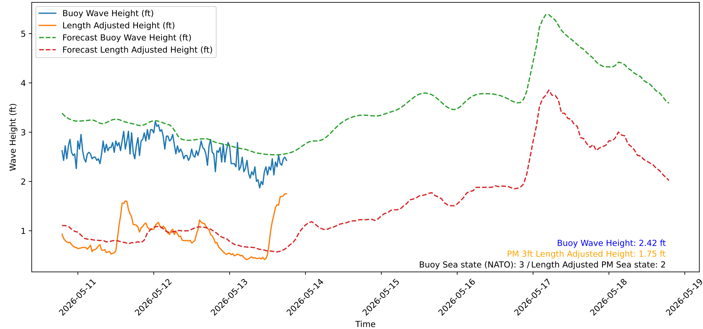
Wave Heights over Time for Red Beach at 2026-05-13 18:50:52
