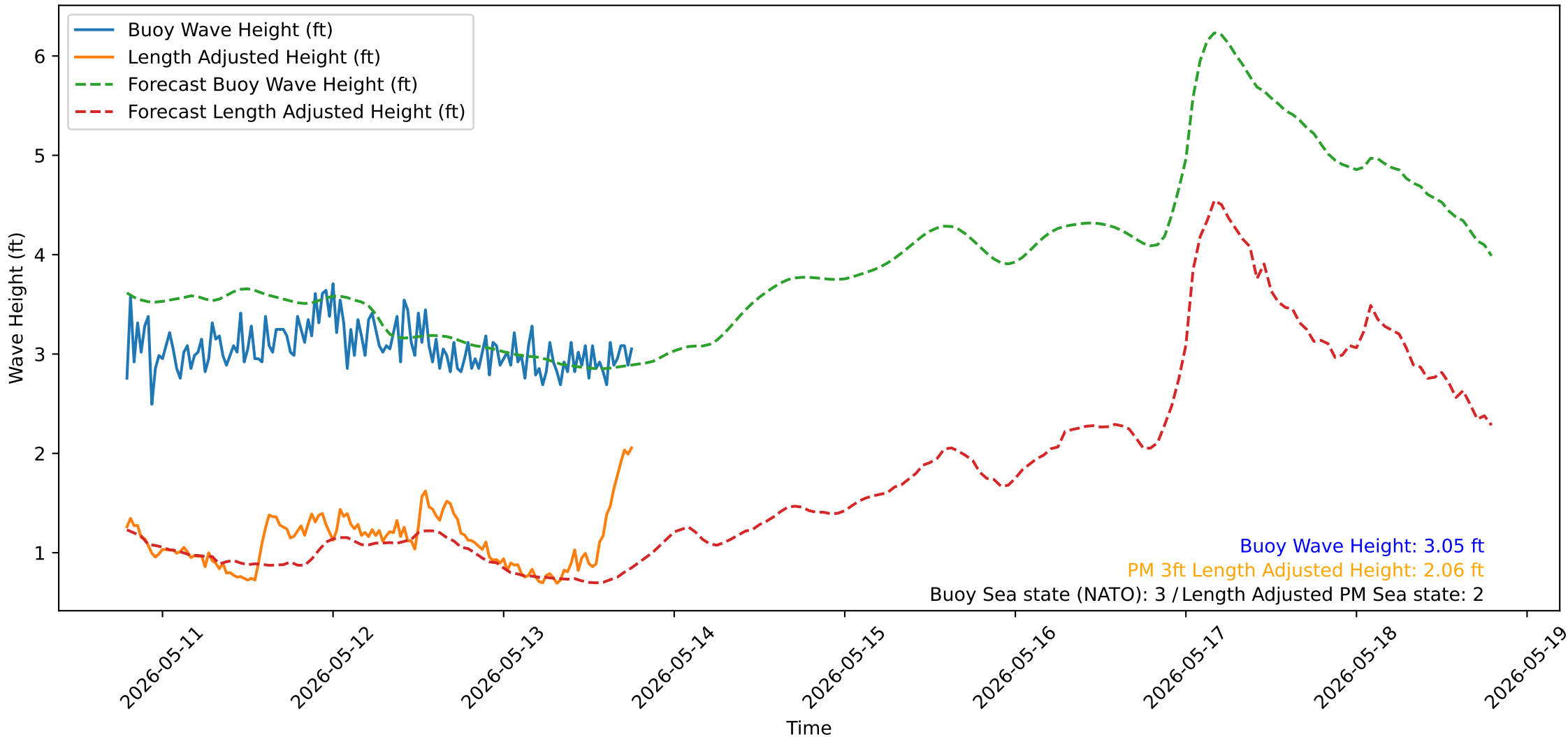
Wave Heights over Time for Oceanside Harbor at 2026-05-13 18:50:32
